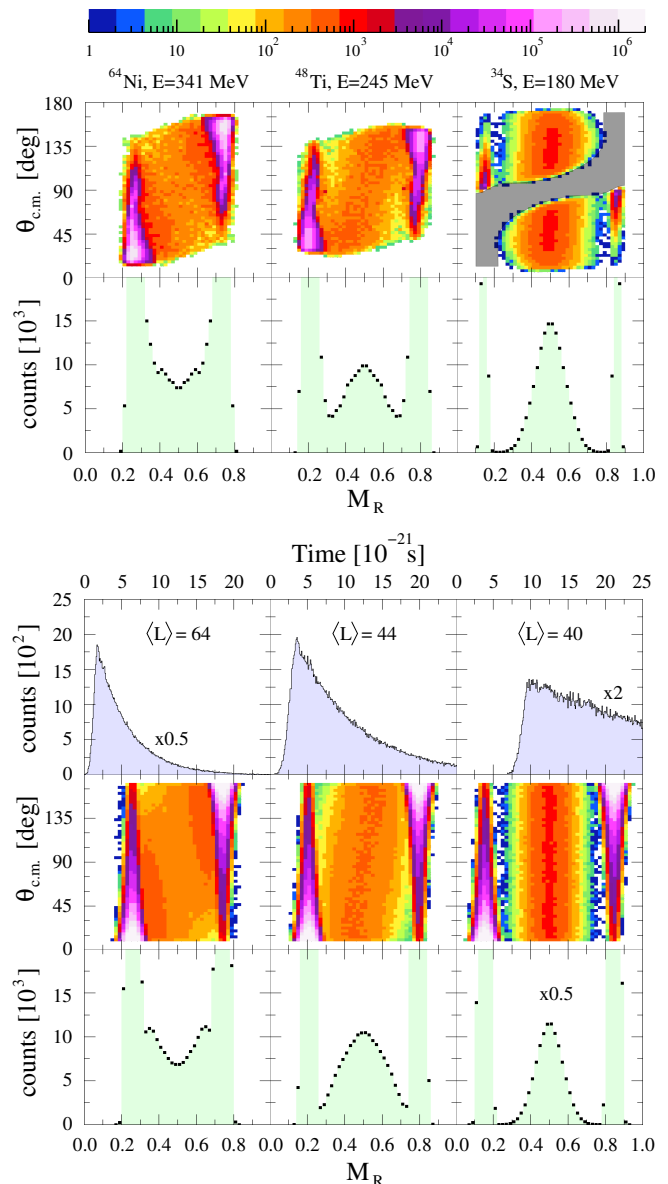
FIG. 2. (Color online) The upper panels show the experimental MAD and corresponding projection onto M_R for ^{64}\text{Ni}+^{184}\text{W} , ^{48}\text{Ti}+^{186}\text{W} and ^{34}\text{S}+^{186}\text{W} (see text). The lower panels show simulated MAD for same reactions and energies, with the M_R spectra at the bottom, and the sticking time distributions above. The capture mean angular momenta \langle L \rangle from CCFULL used in the simulations are also given. These result in good agreement between the simulations and the measurements (top panels).
