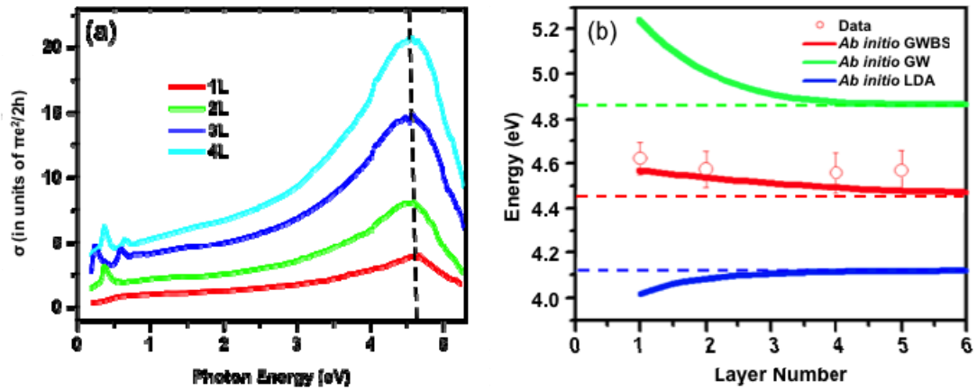
Figure 3: (a) Experimental optical conductivity for single- and few-layer graphene in the spectral range of 0.2 – 5.3 eV. The dashed line is a guide to the eye of the resonance peak. (b) Dependence of the peak energy of the excitonic resonance on layer thickness: experiment (symbols), values calculated from ab-initio LDA (blue), GW (green) and GWBS (red). The dashed lines show the calculated value for bulk graphite.
