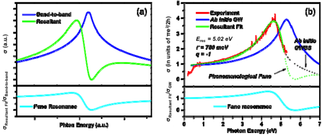
Figure 2 : Fano theory of saddle-point excitons in graphene. Upper panels: optical conductivity of unperturbed band-to-band transitions \sigma_{cont} (blue) and the resultant conductivity from a Fano interference of the exciton state and the continuum (green); lower panels: Fano line shape of Eq. 1. (a) Illustration of the model using the JDOS near the 2D saddle point for \sigma_{cont} and the Fano parameters as described in the text. (b) Fit of experiment (red) to the Fano model using the optical conductivity obtained from GW calculations [7] for \sigma_{cont} . The dashed line is the optical conductivity spectrum obtained from the full GW-Bethe-Salpeter calculation [7].
