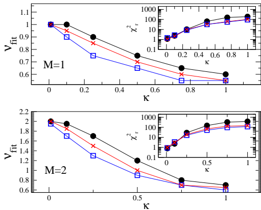
FIG. 2: (Color online) The best fitted value of \nu vs the coupling strength to the continuum, \kappa . Full circles refer to the case of GOE intrinsic Hamiltonian, crosses stand for the case of TBRE with v_0 = d_0/50 , and squares for the case of TBRE with v_0 = 0 (no intrinsic chaos); the number of channels is one (upper panel) and two (lower panel). The inserts show the reduced chi \chi_r^2 as a function of \kappa .
