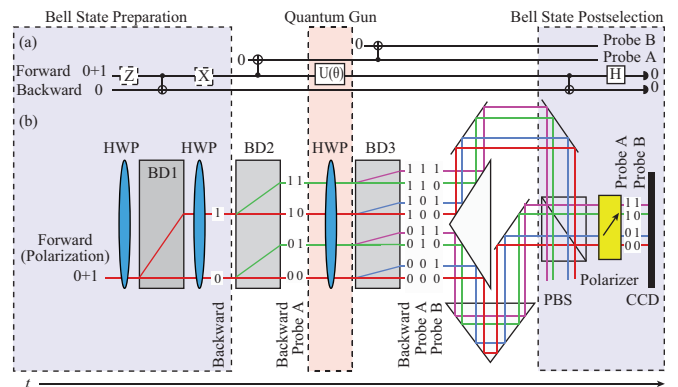
FIG. 3: Experiment to illustrate the P-CTC predictions of the grandfather paradox. a) Quantum circuit. Using a CNOT gate sandwiched between optional Z and X gates, it is possible to prepare all of the maximally entangled Bell states. The Bell state measurement is implemented using a CNOT and a Hadamard. Each of the probe qubits is coupled to the forward qubit via a CNOT gate. b) Experimental apparatus. The polarization and path degrees of freedom of single photons from a quantum dot are entangled via a calcite polarization-dependent beam displacer (BD1), implementing the CNOT. Half-wave plates (HWP) before and after BD1 implement the optional Z and X gates. To complete the teleportation, the post-selection onto |\phi^+\rangle is carried out by recombining the path degrees of freedom on a polarizing beamsplitter (performing a CNOT gate between path and polarization) and then passing the photons through a calcite polarizer set to 45^\circ and detecting them. A rotatable HWP acts as a quantum gun, implementing the unitary U(\theta) = e^{-i\theta\sigma_x} . Removable calcite beam displacers (BD2 and BD3) couple the polarization qubit to two probe qubits encoded in additional spatial degrees of freedom.
