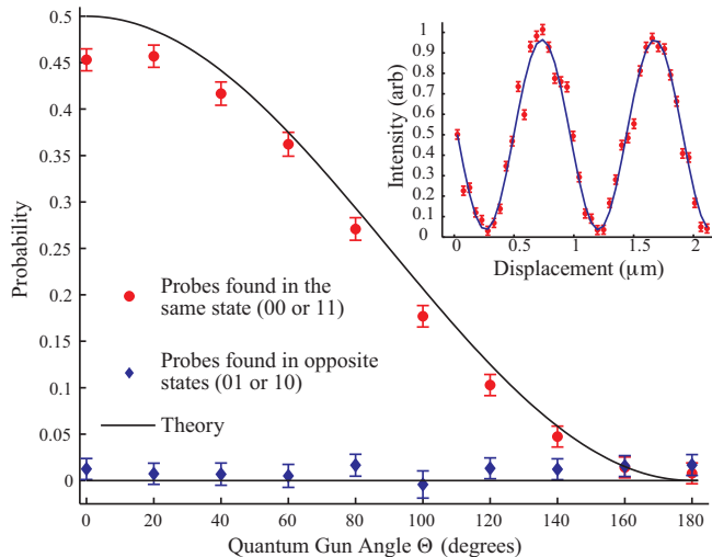
FIG. 4: Probability that the postselection simulating time travel succeeds and the probes are found in the same state (red circles) or in opposite states (blue diamonds). As the accuracy \theta of the quantum gun increases from 0 to \pi , the probability that the teleportation succeeds decreases. Nonetheless, the probability that the probe qubits are found in either the 10 or 01 state (i.e. the kill succeeds) is 0.01 \pm 0.04 . Solid curves correspond to theoretical predictions. The theory/experiment discrepancy is due to a 1.1 \pm 0.1^\circ mismatch between polarizers used for teleportation. The error bars are due to photon counting and background from the cooled CCD. Inset: the teleportation loop is a polarization interferometer with measured visibility 93 \pm 3\% .
