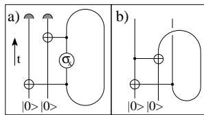
FIG. 2: a) Grandfather paradox circuit. If we take 1 to represent ‘time-traveler exists,’ and 0 to represent ‘she doesn’t exist,’ then the NOT ( \sigma_x ) operation implies that if she exists, then she ‘kills her grandfather’ and ceases to exist; conversely, if she doesn’t exist, then she fails to kill her grandfather and so she exists. The difference between Deutsch’s CTCs and our P-CTCs is revealed by monitoring the time-traveler with two controlled-NOTs (CNOT): the two controlled bits are measured to determine the value of the time-traveling bit before and after the \sigma_x . Opposite values mean she has killed her grandfather; same values mean she has failed. Using Deutsch’s CTCs, she always succeeds; using P-CTCs she always fails. b) Unproved theorem paradox circuit. The time-traveler obtains a bit of information from the future via the upper CNOT. She then takes it back in time and deposits a copy an earlier time in the same location from which she obtained it (rather, will obtain it), via the lower CNOT. The circuit is unbiased as to the value of the ‘proof’ bit, so it automatically assigns that bit a completely mixed value, as it is maximally entangled with the one emerging from the CTC.
