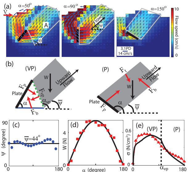
FIG. 5. (color online) Flow of grains and force-balance model: (a) Flow field in the vertical ( xz ) plane for three plate (solid black line) orientations. Gray boundary indicates regions with upward flow [18]. (b) Forces on a wedge for \alpha < \alpha_{vp} [regime (VP)] and on the band for \alpha \geq \alpha_{vp} [regime (P)]. (c) The average flow velocity angle \psi in the upward-flow region vs. \alpha ( \bullet ). (d) The weight of the upward-flow region as function of \alpha calculated from simulation ( \blacksquare ) and fit (black) to W = c \sin(\alpha) , where c = 5.7 N. (e) Normal component of the stress on the plate \sigma calculated from the model (black) and measured from simulation ( \blacktriangle ). The black dashed line \alpha = \alpha_{vp} = 97^\circ indicates the boundary between the two regimes (VP) and (P).
