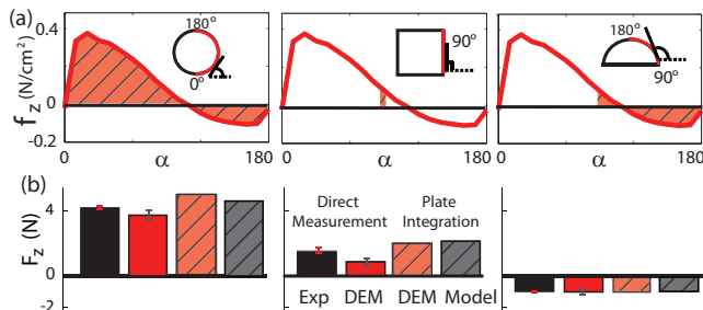
FIG. 4. (color online) (a) F_z on intruders calculated by integration of f_z(\alpha) . Red outlines on the shapes indicate the leading surface and the hatched area indicates the corresponding range of \alpha and region of integration. (b) F_z calculated by integration of f_z from simulation (red hatched bar) and model (gray hatched bar) compared to direct measurement of F_z in experiment (black bar) and simulation (red bar).
