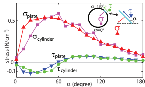
FIG. 2. Normal ( \sigma ), and shear ( \tau ), stress on the leading surface of the cylinder as a function of tangent angle \alpha compared to the stresses on a plate with the same \alpha . \blacksquare , \blacktriangle , \bullet , and \blacktriangledown represent \sigma_{cylinder} , \sigma_{plate} , \tau_{cylinder} and \tau_{plate} respectively.
