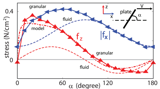
FIG. 3. (color online) (a) The drag ( |f_x| , blue) and lift ( f_z , red) components of the stress on a plate as a function of \alpha in granular media ( \blacktriangleleft and \blacktriangle ) as compared to a fluid with with Re \ll 1 (dashed lines) [17]. Dash-dot red line is granular wedge model (see Force model section).
