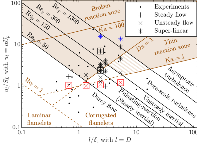
FIG. 4. Regime diagram of reacting flows in porous media populated with the flow conditions simulated in this study and those examined in literature experiments (black dots, see Fig. S7 in the Supplemental Material [31]). Regions of strong dispersion-chemistry coupling are indicated with brown shadings. The Reynolds transition values are obtained from non-reacting simulations and the lines shown are for \alpha = 0.3 , \nu = 1.6 \times 10^{-5} \text{ m}^2/\text{s} , S_L = 23 \text{ cm/s} , and \delta_c = 0.6 \text{ mm} . The colored symbols indicate simulations with reaction fronts propagating upstream (in red, U_D < \overline{S_c} ), or downstream (in blue, U_D > \overline{S_c} ). Cases for which \overline{S_c}/S_L > 1.15 \overline{A_f}/A_\perp are denoted as super-linear. The symbols enclosed in squares correspond to the cases shown in Fig. 1. The location of symbols are offset by up to 10% for readability.
