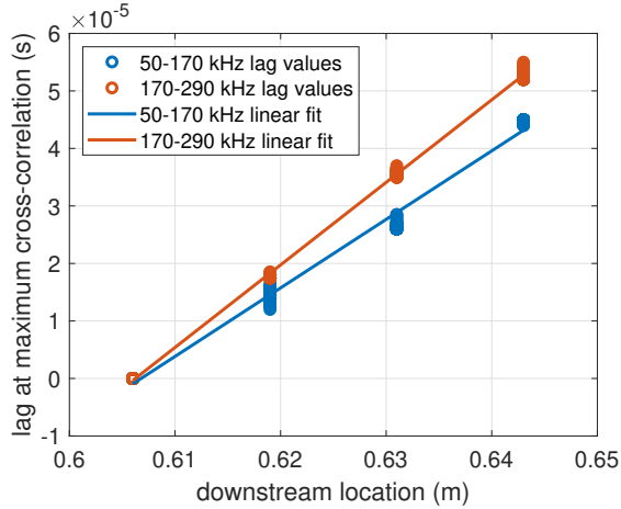
FIG. 25: Lag times used to estimate disturbance velocities for the shear-layer and second-mode waves. The data are accumulated from 60 runs across two entries. All results are at Re = 11.6 \times 10^6/m .
