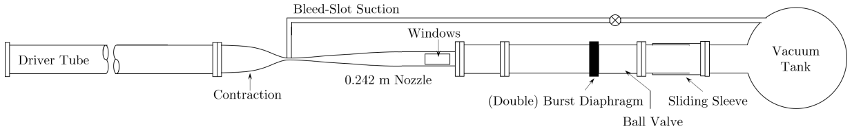
FIG. 2: BAM6QT schematic
