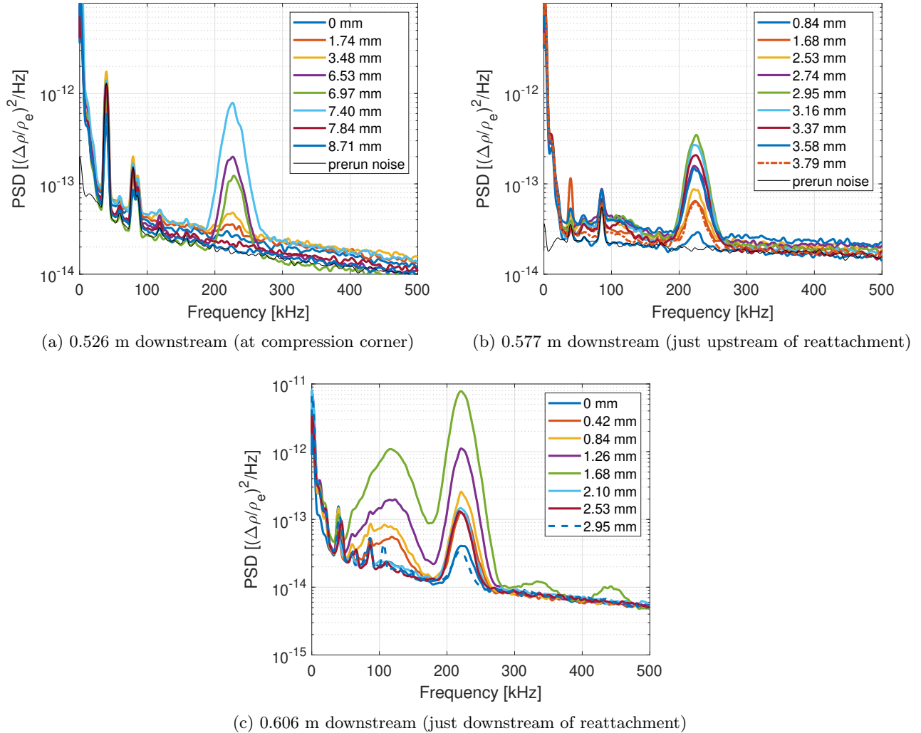
FIG. 28: FLDI density gradient fluctuation PSDs for Re = 11.5 \times 10^6/m . Only second mode waves can be seen in the shear layer at the compression corner. The shear-layer traveling waves start to rise up from the noise floor in measurements taken in the downstream portion of the shear layer. Distances in the legends correspond to heights off the surface.
