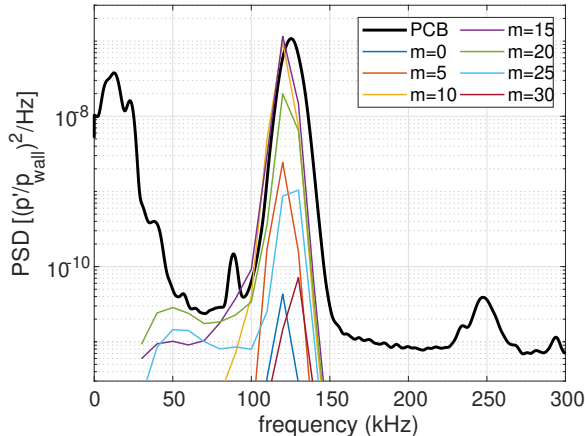
FIG. 8: Measured and computed surface pressure spectra 0.752 m downstream of the nosetip. The thick black line corresponds to the PCB measurement, while the colored lines correspond to the linear amplification of computed planar and oblique waves at different azimuthal wavenumbers, m . Re = 11.5 \times 10^6/m .
