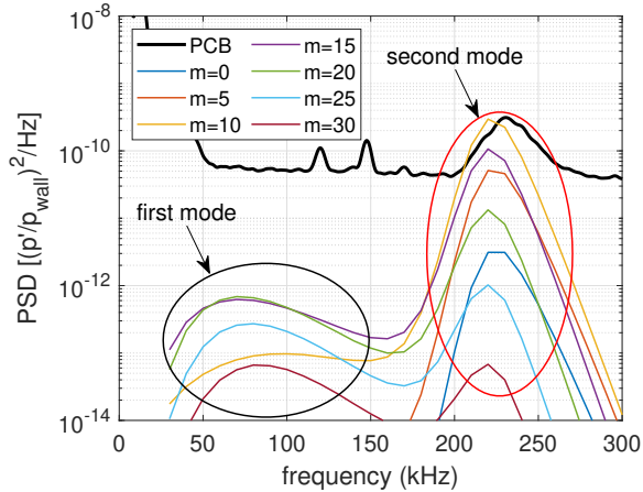
FIG. 21: Measured and computed surface pressure spectra on the cone, 0.387 m downstream of the nosetip. The vertical axis has been expanded to show the first mode from the computations. Re = 11.5 \times 10^6/m , data from Paredes et al. [31].
