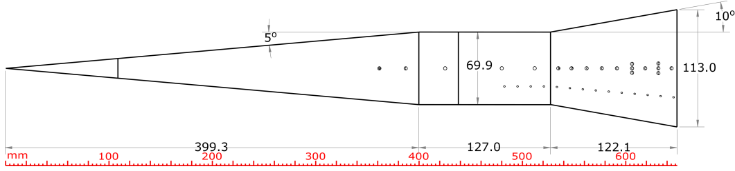
(b) 10° flare model illustration
