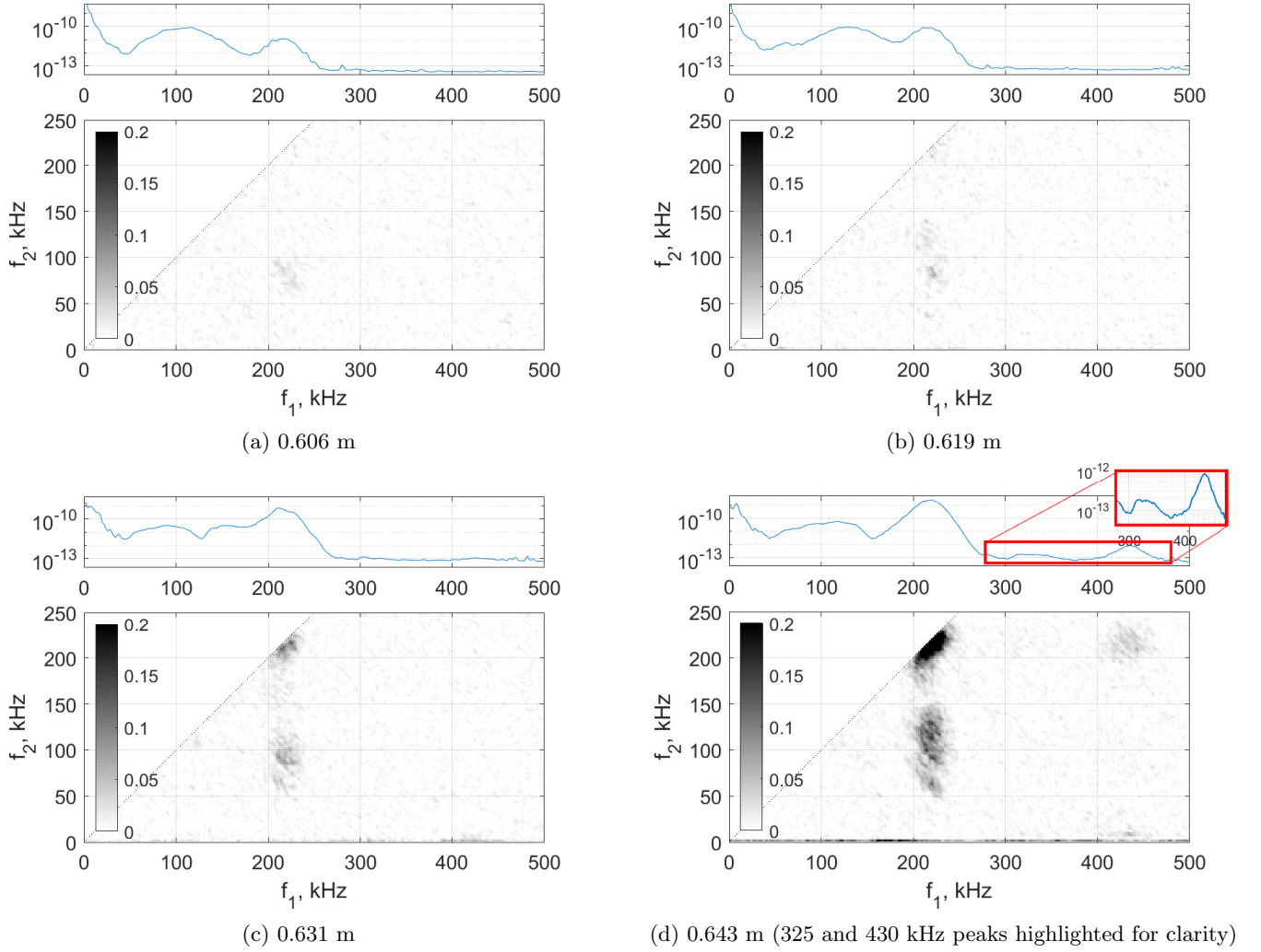
FIG. 26: Bicoherences for PCB sensors under reattached boundary layer on the flare. Upper plot displays power spectral density for the same data. Bicoherence significance threshold b_{95}^2 = 0.0075 .
