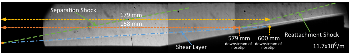
FIG. 14: Illustration of bubble size estimation methods overlaid on composite schlieren image at Re = 11.7 \times 10^6/m . The orange dots represent the estimated separation and reattachment points found by extrapolating the separation and reattachment shocks to the shear layer, while the yellow dots represent those found by extrapolating the shear layer to the model surface. The separation point for both methods is in approximately the same location for this case. Flow is from left to right.
