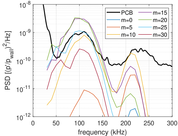
FIG. 22: Measured and computed surface pressure spectra along the cone 0.606 m downstream of the nosetip. The thick black line corresponds to the PCB measurement, while the colored lines correspond to the linear amplification of computed planar and oblique waves at different azimuthal wavenumbers, m . Re = 11.5 \times 10^6/m , data from Paredes et al. [31].
