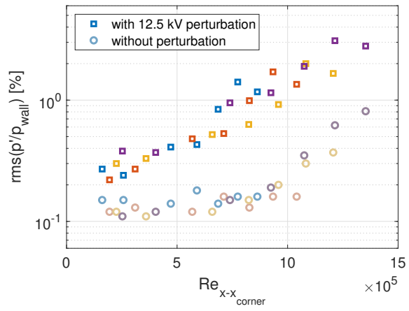
FIG. 37: Integrated RMS amplitudes with and without perturbation (integrated between 50 and 270 kHz).
