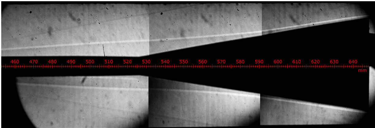
FIG. 13: Composite of six schlieren images at Re = 11.7 \times 10^6/m . Flow is from left to right. Dimensions in mm from the sharp nosetip.
