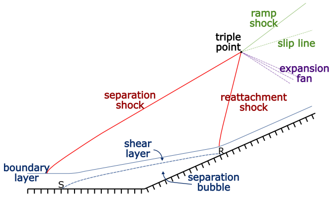
FIG. 1: Canonical SBLI
