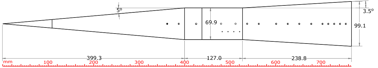
(a) 3.5° flare model illustration
