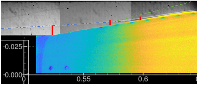
FIG. 27: FLDI sweep locations (red lines), with schlieren and heat flux overlays, Re = 11.5 \times 10^6/m . Flow is from left to right. The shear layer is outlined with a blue dotted line, while the reattachment shock is extrapolated with a green dashed line. Note that, based on the schlieren measurements, reattachment is not believed to have occurred until around 0.58-0.60 m downstream. Therefore, the two upstream locations are likely both measurements of the shear layer, while the third is most likely the reattached boundary layer.
