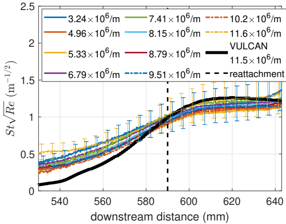
FIG. 18: Normalized heat flux for Re between 3.24 \times 10^6 and 11.6 \times 10^6/m . The compression corner is at the left edge (526 mm downstream) and reattachment is estimated to be between 579 and 600 mm downstream (the black dashed line represents the center of this range).
