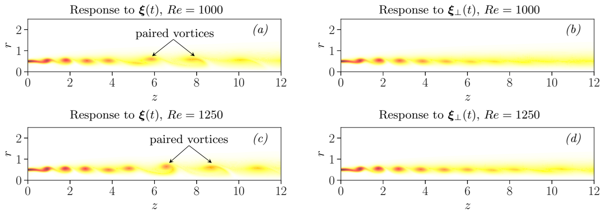
FIG. 9. In panels (a) and (b) we show the vorticity field from the nonlinear response to inputs (39) and (41), respectively, at time t = 40T , Re = 1000 and forcing amplitude \varepsilon = 5 \times 10^{-3} . Panels (c) and (d) show the analog for Re = 1250 and forcing amplitude \varepsilon = 10^{-3} . The colorbar is shown in figure 4a.
