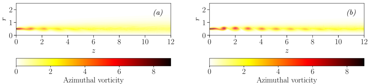
FIG. 4. Vorticity snapshots from the T -periodic solution at time t = 0 for (a) Reynolds number Re = 500 and (b) Reynolds number Re = 1250 . The colorbar ranges from 0 to 9 and it has been slightly saturated to better visualize downstream vortices.
