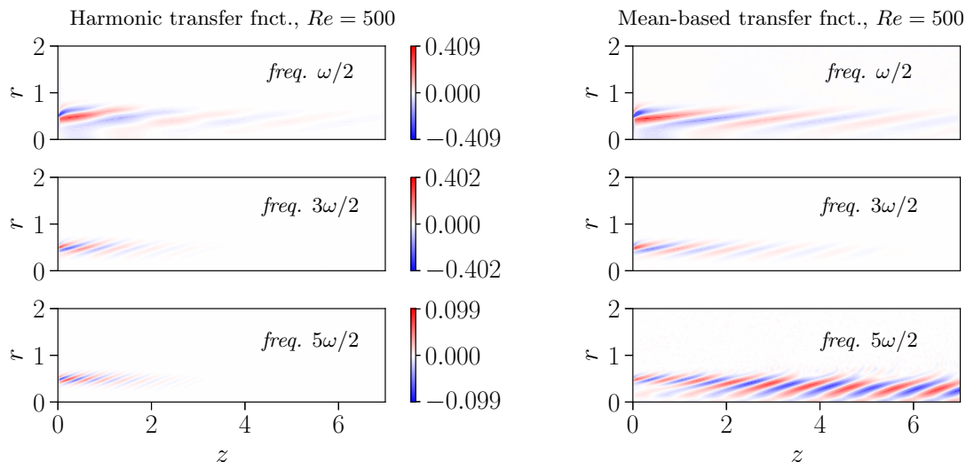
FIG. 7. On the left we show the vorticity field from the \omega/2 -, 3\omega/2 - and 5\omega/2 -entries of the first right singular vector (i.e., the first input mode) of \tilde{\mathbf{H}}(i\omega/2) at Re = 500 . The right panels are the analog of the left ones for the mean-based transfer functions \tilde{\mathbf{R}}(i\omega/2) , \tilde{\mathbf{R}}(i3\omega/2) and \tilde{\mathbf{R}}(i5\omega/2) . The colorbar is not shown on the right because these frequencies are decoupled and the modes are scaled arbitrarily.
