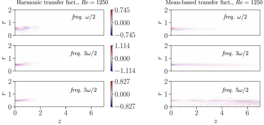
FIG. 8. Analog of figure 7 for Re = 1250 .
