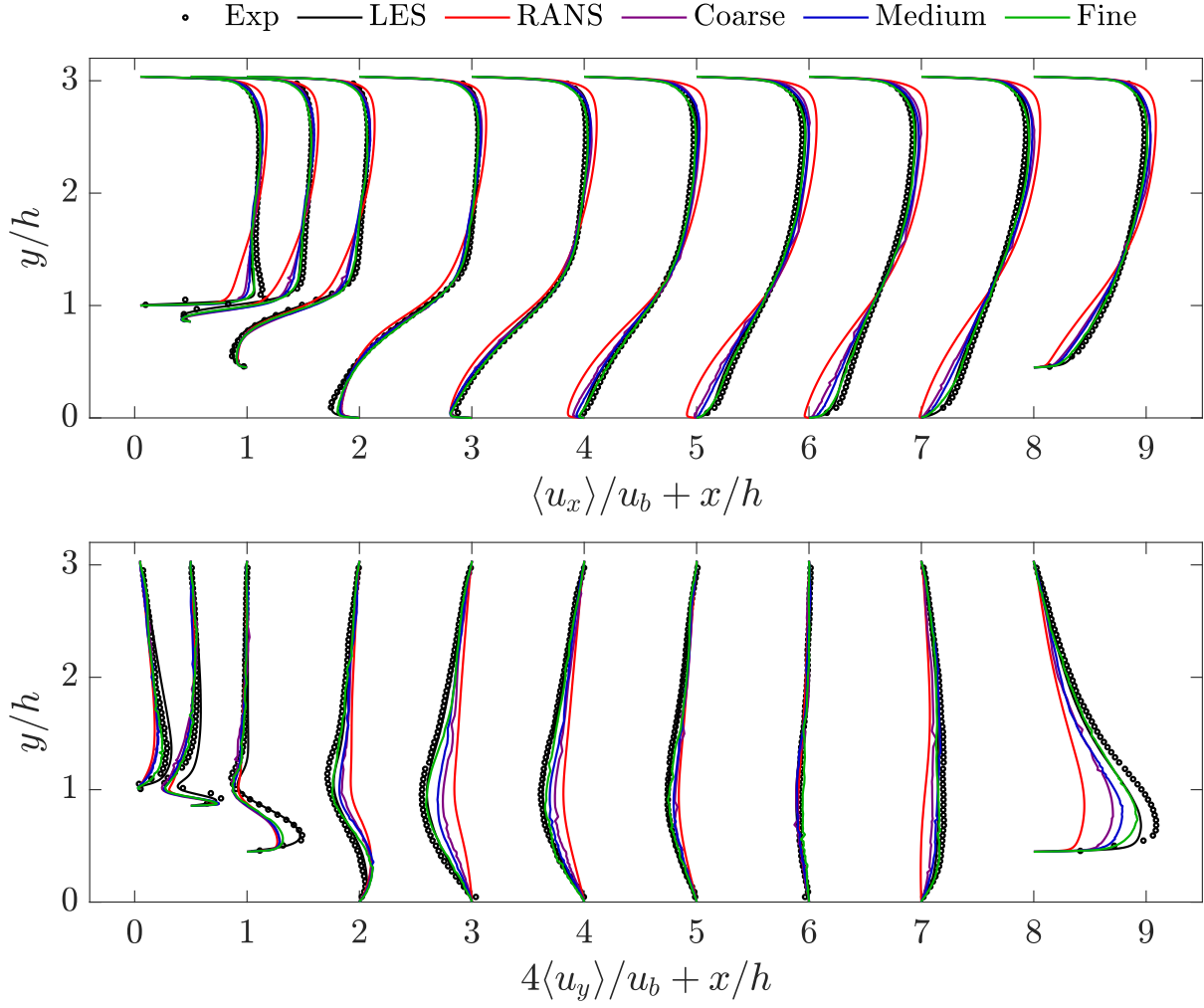
FIG. 10: Mean streamwise (top) and vertical (bottom) velocity profiles normalized by the bulk velocity, u_b , offset by streamwise location normalized by the hill height, h , for all resolutions in Table II, along with data from the experiments of [82] and WRLES of [48]. Note that the vertical velocity is multiplied by a factor of four to enhance visibility.
