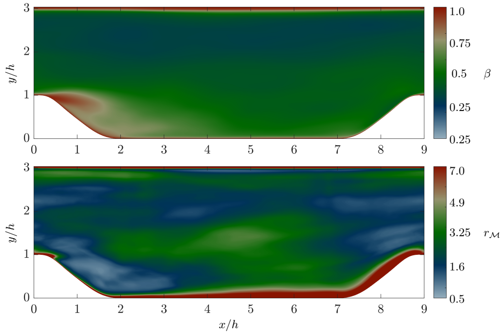
FIG. 11: Mean contours of the unresolved turbulence energy fraction \beta (top) and resolution adequacy r_M (bottom) for the fine resolution simulation.
