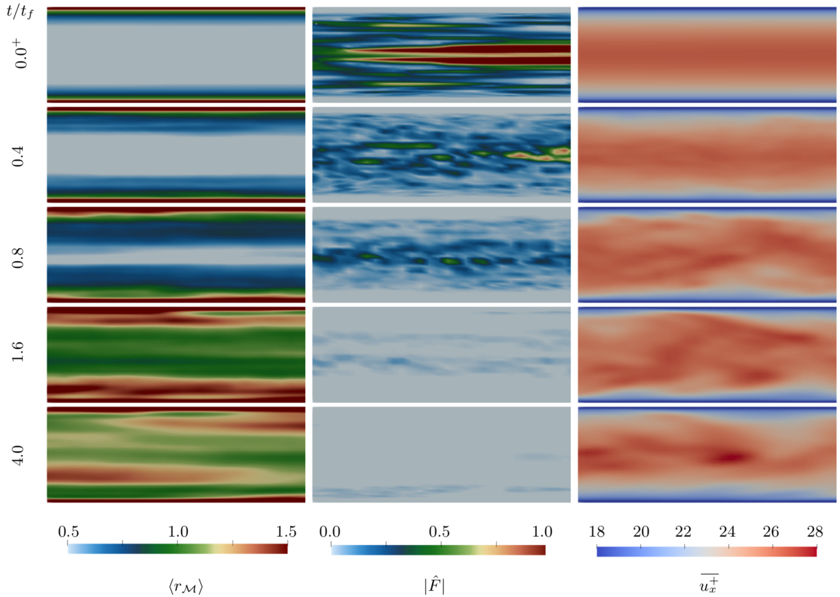
FIG. 4: Snapshots of (left) mean resolution adequacy parameter, \langle r_{\mathcal{M}} \rangle (34), (middle) magnitude of scaled forcing vector field, \hat{F}_i = F_i/F_c where F_c = 0.25(\Delta_x\Delta_y\Delta_z)^{-1/3}k_{tot}^{3/2} (45), and (right) resolved streamwise velocity in x - y planes for the temporally developing hybrid simulation of channel flow at Re_\tau \approx 5200 . Note that k_{tot} used to define F_c is a function of wall distance. Only results for the coarse resolution are shown here. Time since initiation of forcing t/t_f is shown, where t_f is the flow-through time.
