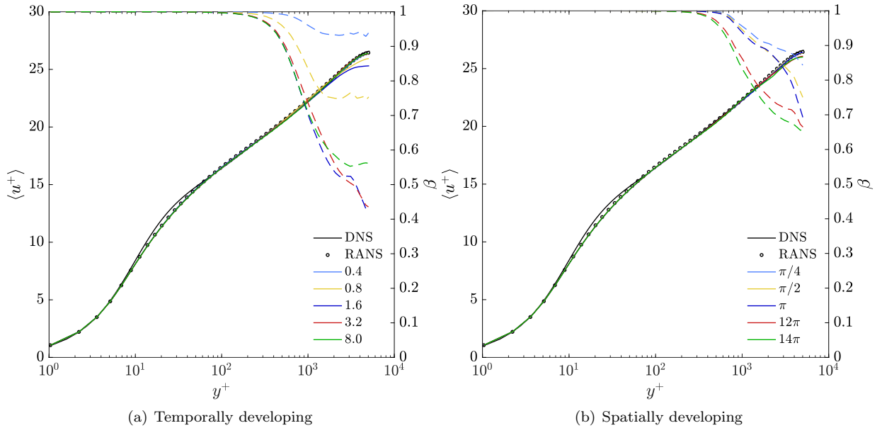
FIG. 5: Mean streamwise velocity for fully developed channel flow at Re_\tau \approx 5200 along with the fraction of unresolved turbulent kinetic energy \beta (dashed). In (a) the simulation evolves in time from the stationary RANS solution to the stationary hybrid solution. Numbers in the legend refer to t/t_f , the time in flow through units. In (b), the hybrid simulation evolves in the streamwise direction from the inlet RANS solution to a hybrid solution. Numbers in the legend refer to x/\delta , the down-stream distance normalized by channel half-width.
