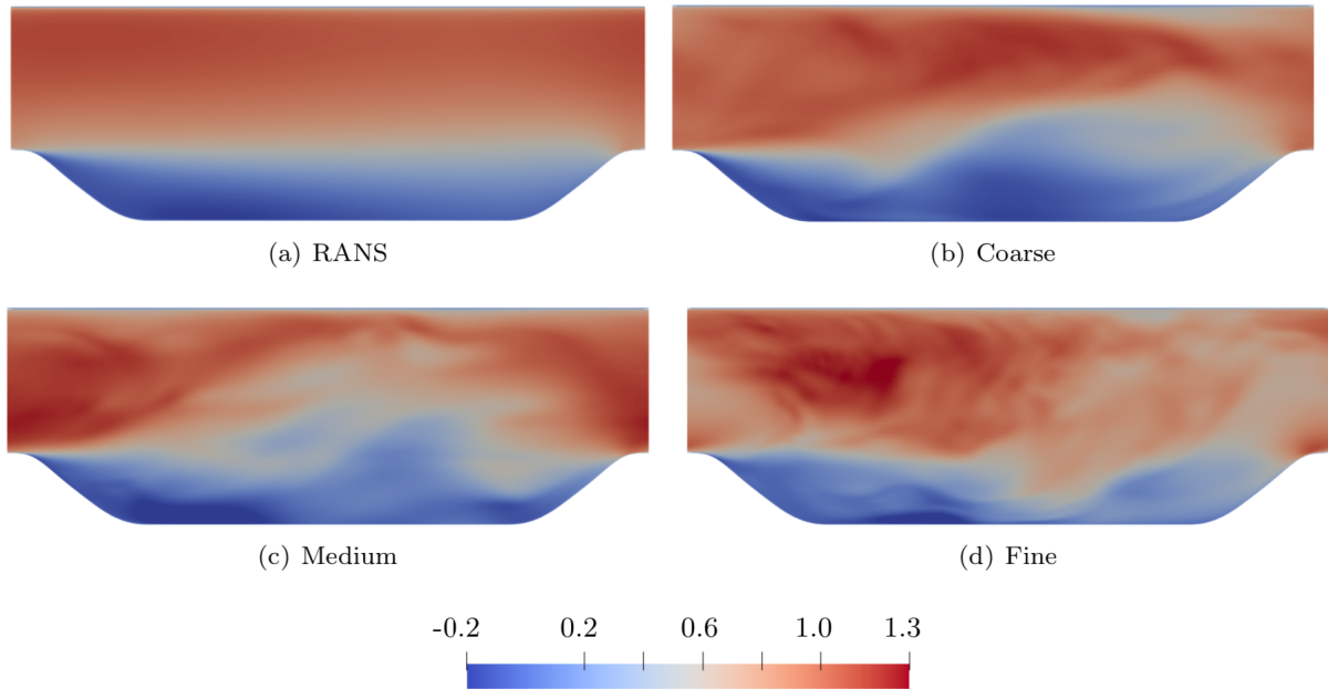
FIG. 9: Streamwise velocity contours for the periodic hill test case using (a) \overline{v^2} - f RANS and (b-d) AMS using the coars through fine grids of Table II. Instantaneous AMS snapshots are shown here to illustrate the degree of resolved turbulence, mean velocity profiles for AMS are shown in Fig. 10.
