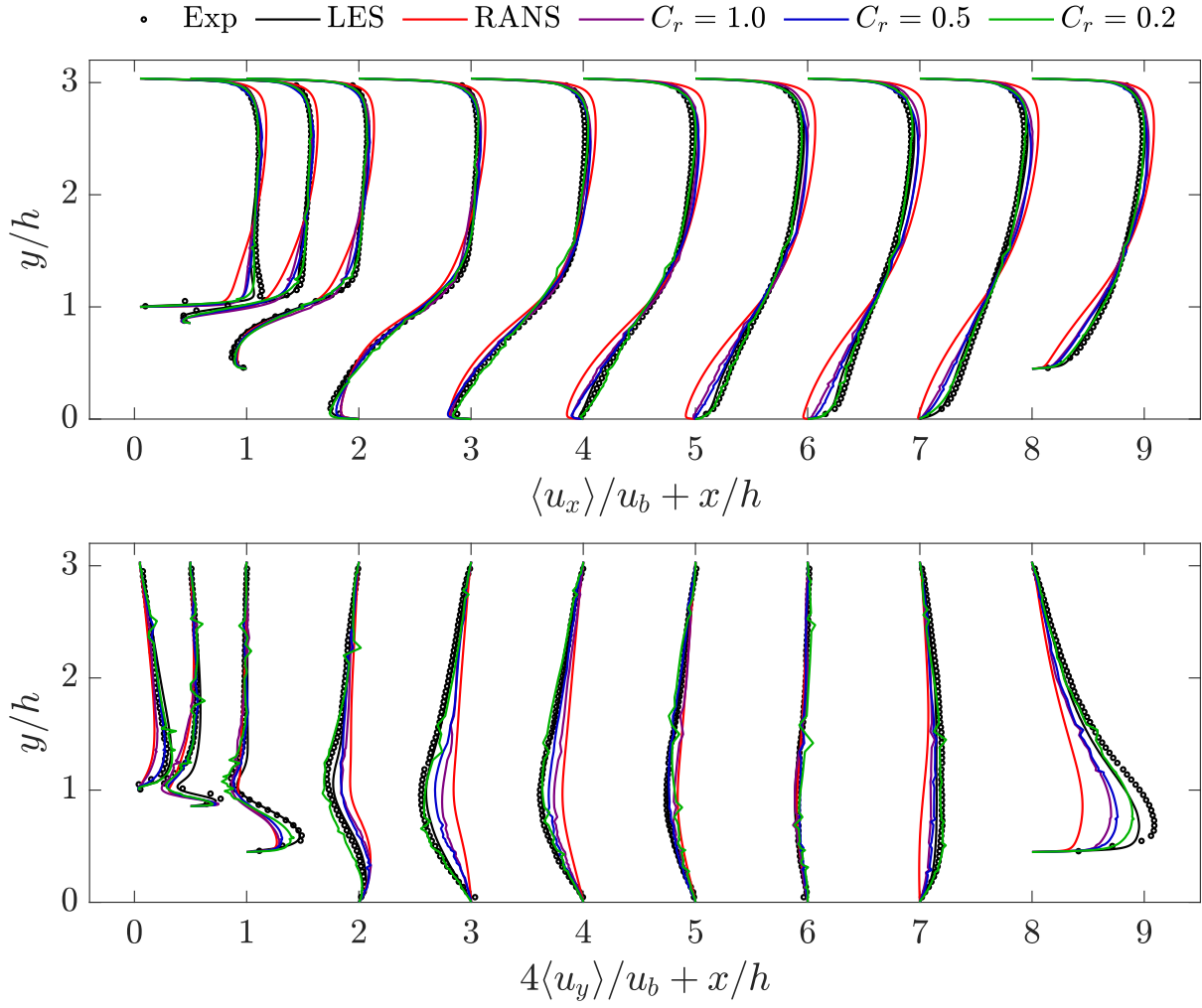
FIG. 14: Mean streamwise (top) and vertical (bottom) velocity profiles normalized by the bulk velocity, u_b , offset by streamwise location normalized by the hill height, h , for only the coarse grid in Table II using different C_r values, along with data from the experiments of [82] and WRLES of [48], of four to enhance visibility.
