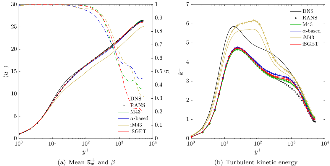
FIG. 16: Mean streamwise velocity in wall units (a) for fully developed channel flow at Re_\tau \approx 5200 along with the fraction of unresolved of resolved turbulence \beta (dashed), and (b) turbulent kinetic energy k^+ of the statistically steady solution using different energy transfer models and the fine resolution of Table I. In (b), the lines marked with + symbols are k^+ obtained directly from the RANS model while the unmarked lines are the time-averaged resolved turbulence plus \beta times the RANS k^+ . Simulations have been run for approximately 80 flow-throughs.
