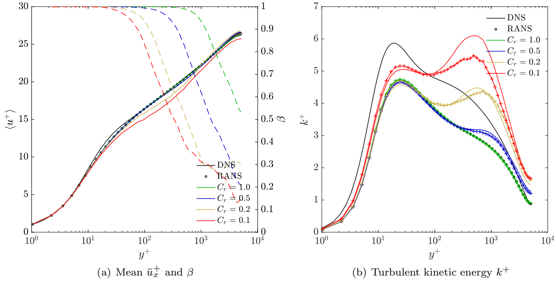
FIG. 13: Mean streamwise velocity in wall units (a) for fully developed channel flow at Re_\tau \approx 5200 along with the fraction of unresolved turbulence \beta (dashed), and (b) turbulent kinetic energy k^+ of the statistically steady solution highlighting the sensitivity to the parameter C_r . In (b), the lines marked with + symbols are k^+ obtained directly from the RANS model while the unmarked lines are the time-averaged resolved turbulence plus \beta times the RANS k^+ . Simulations have been run for approximately 80 flow-throughs.
