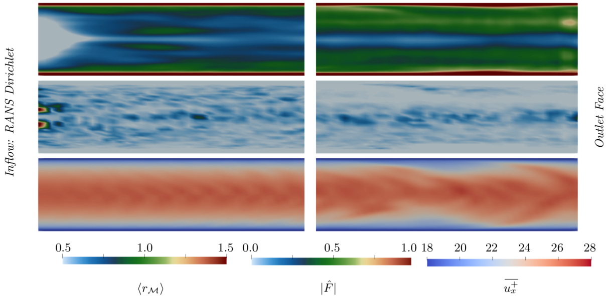
FIG. 7: Inlet (left) and outlet (right) sections of the spatially evolving channel with coarse resolution. Shown are (top) pseudo-mean resolution adequacy parameter \langle r_{\mathcal{M}} \rangle , (middle) magnitude of the scale forcing |\hat{F}| , and (bottom) resolved streamwise velocity \overline{u_x^+} . Inflow/outflow streamwise sections of 4h , out of the total 16\pi , are shown.
