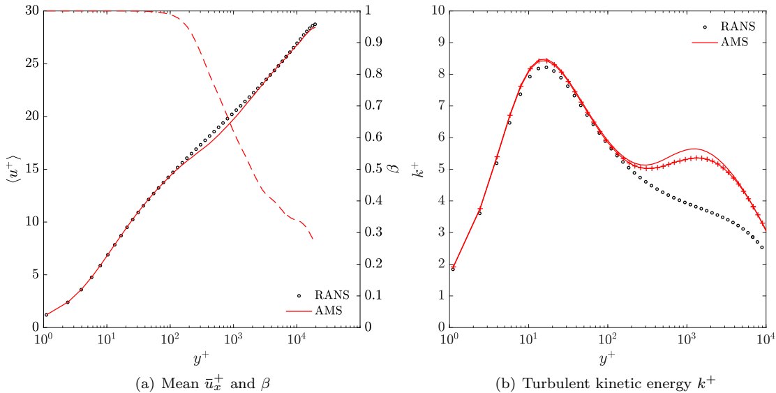
FIG. 8: Mean streamwise velocity in wall units (a) for fully developed channel flow at Re_\tau = 20K along with the fraction of unresolved turbulence \beta (dashed), and (b) turbulent kinetic energy k^+ of the statistically steady solution. In (b), lines marked with + symbols are k obtained directly from the hybrid RANS model while the unmarked lines are the time-averaged resolved turbulence plus \alpha times the RANS k^+ . Simulations have been run for nearly 100 convective times.
