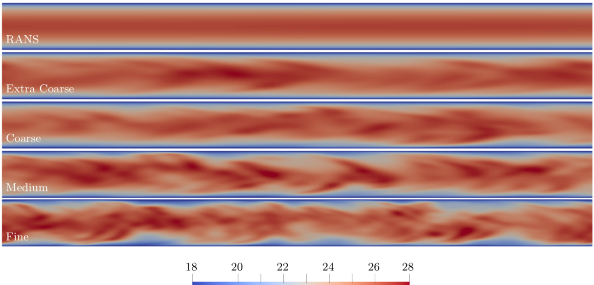
FIG. 2: Instantaneous streamwise velocity in an x - y plane in fully developed channel flow at Re_\tau \approx 5200 using the Chien k - \varepsilon RANS model and the AMS hybrid formulation, with resolutions described in Table 1.
