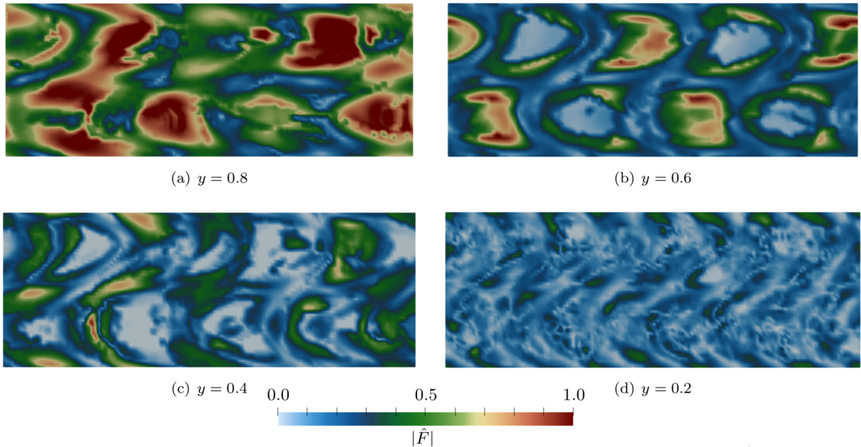
FIG. 6: Magnitude of scaled forcing vector field, \hat{F}_i = F_i/F_c where F_c = 0.25(\Delta_x\Delta_y\Delta_z)^{-1/3}k_{tot}^{3/2} , at multiple wall-parallel planes a t = 0.04 after initiating forcing from the steady RANS solution. Entire spanwise domain is displayed. Early forcing experiences no clipping yielding large coherent acceleration with the size of the structures decreasing with proximity to the wall. Note that k_{tot} is dependent on wall distance.
