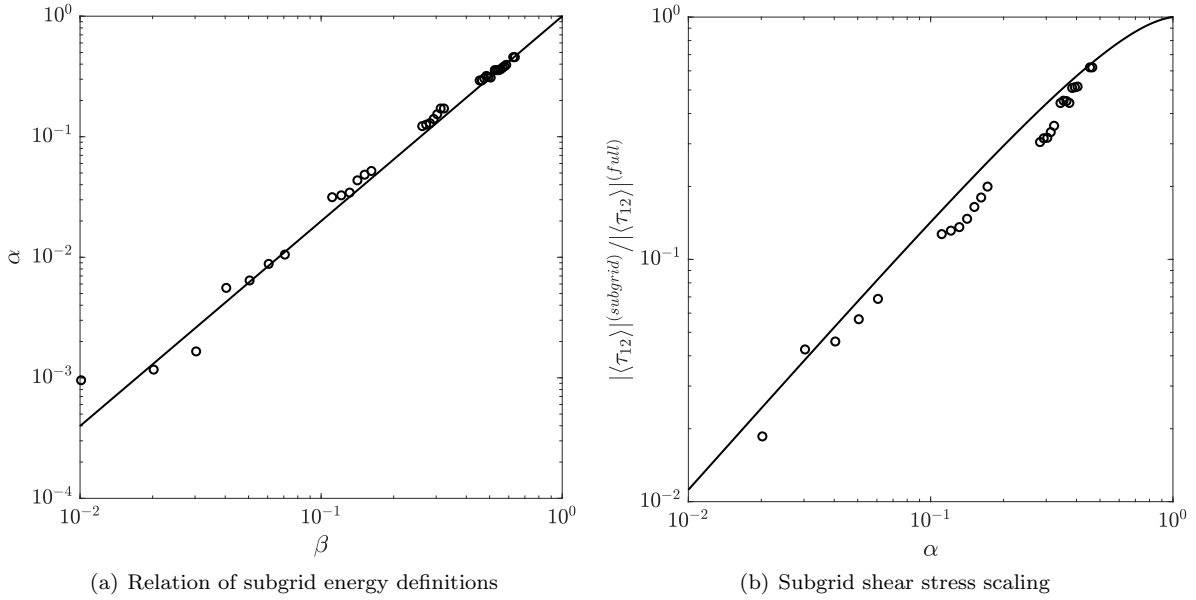
FIG. 1: Subgrid information determined by applying box filters to channel flow DNS data at Re_\tau = 1000 [71], (a) relationship between \alpha = \langle u_i^< u_i^</> / \langle u_j' u_j' \rangle and \beta = 1 - \langle u_i^> u_i^> / \langle u_j' u_j' \rangle overlaid with \alpha = \beta^{1.7} and (b) ratio of total subgrid shear stress (including mixed terms) and total shear stress, overlaid with \alpha(2 - \alpha) .
