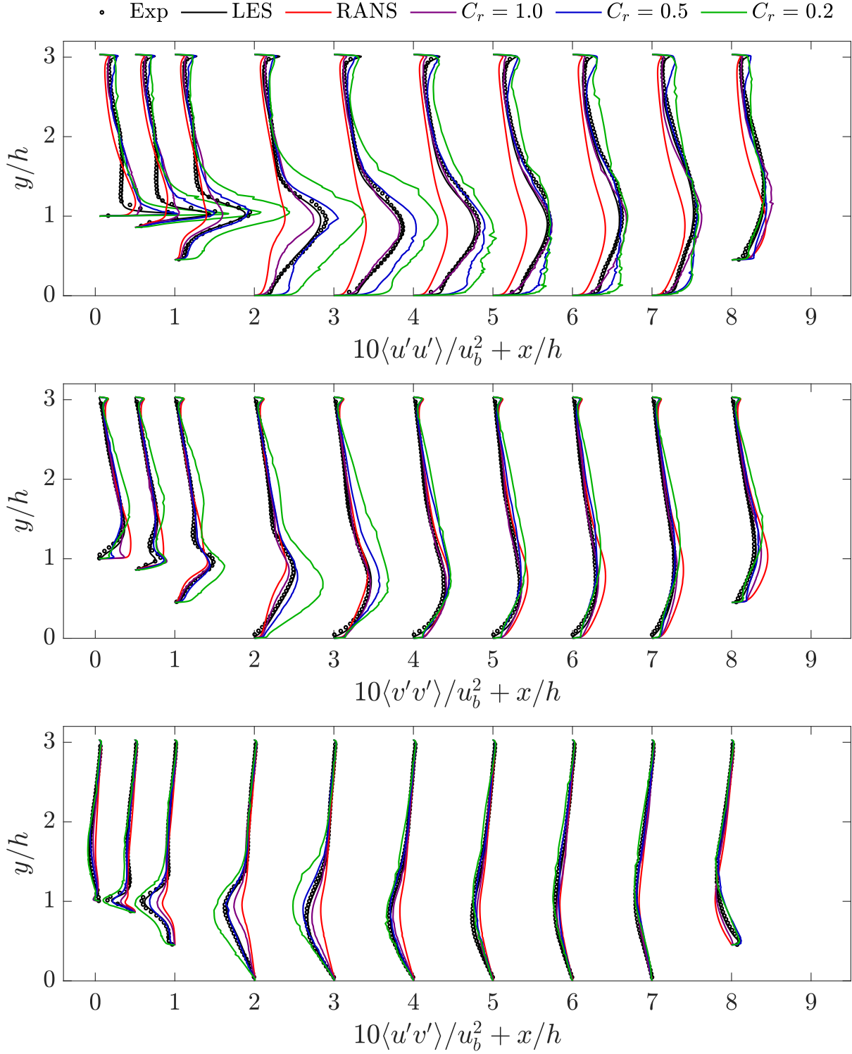
FIG. 15: Profiles of the mean total (model plus resolved) Reynolds stress components normalized by the bulk velocity, u_b , offset by streamwise location normalized by the hill height, h , for only the coarse grid in Table II using different C_r values, along with data from the experiments of [82] and WRLES of [48]. Shown are the streamwise velocity variance (top) vertical velocity variance (middle) and Reynolds shear stress (bottom). Note amplification by a factor of 10 for visibility.
