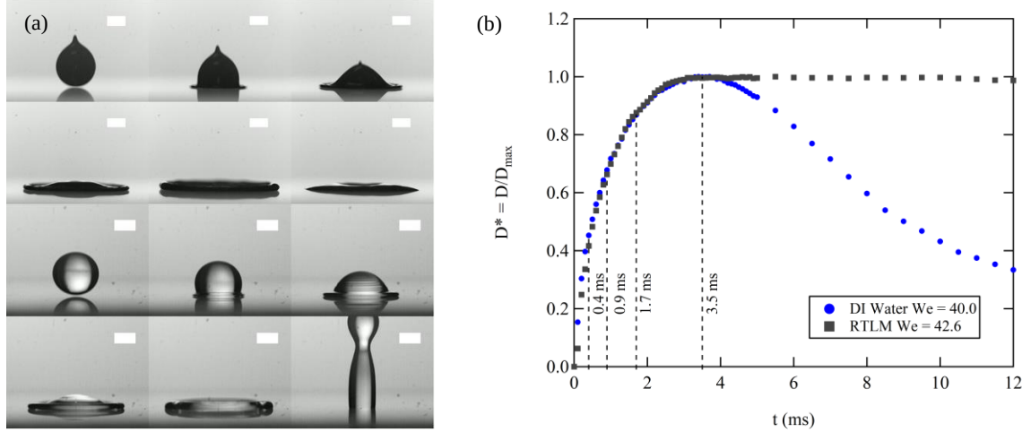
FIG 2. (a) Impact sequence of liquid metal droplets at We = 42.6 (top) and DI water droplets at We = 40.0 (bottom) on hydrophobic substrate. Time stamps are 0 ms, 0.4 ms, 0.9 ms, 1.7 ms, 3.5 ms, and 15.4 ms for both sequences. Scale bar indicates 1 mm. (b) the same sequence normalized by D_{max} note that \xi_{max} is not the same for both data sets.
