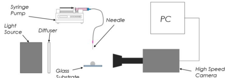
FIG 3. Experimental set up for droplet impact experiments.
