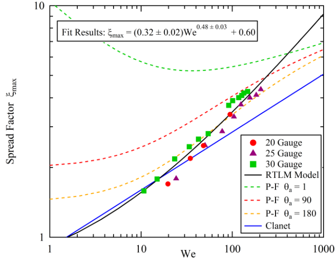
FIG 5. Comparison of spread factor scaling models and impact data. Green, red and orange dashed lines are the Pasandideh-Fard model for normal surfaces [22] for advancing contact angles of 1, 90 and 180 respectively, the solid blue line is the Clanet model for water on a superhydrophobic surface [24], and the solid black line is this work. The markers indicate the impact data and are differentiated by needle size.
