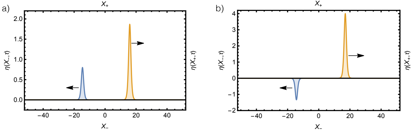
Figure 3. a) Left (blue) and right (yellow) moving soliton in the weak parity breaking regime with parameters |\bar{v}_o| = \frac{1}{15} , \bar{k} = 1 and \tau = 1 . b) Left (blue) and right (yellow) moving soliton in the strong parity breaking regime with parameters |\bar{v}_o| = \frac{1}{3} , \bar{k} = 1 and \tau = 1 .
