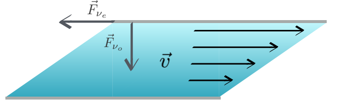
Figure 1. A shearing flow \vec{v} is subjected to a dissipative force opposite to the direction of the fluid motion due to shear viscosity whereas the odd viscosity \nu_o generates an in-plane force normal to the fluid motion. The normal force to the motion is non-dissipative.
