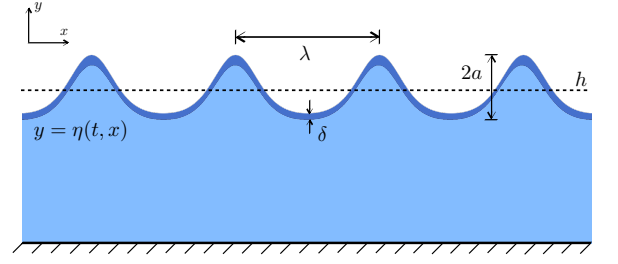
Figure 2. Schematics of the shallow fluid dynamics with free surface. Here a denotes the amplitude of the edge profile and \delta is the boundary layer thickness. The vertical direction is exaggerated to highlight these features.
