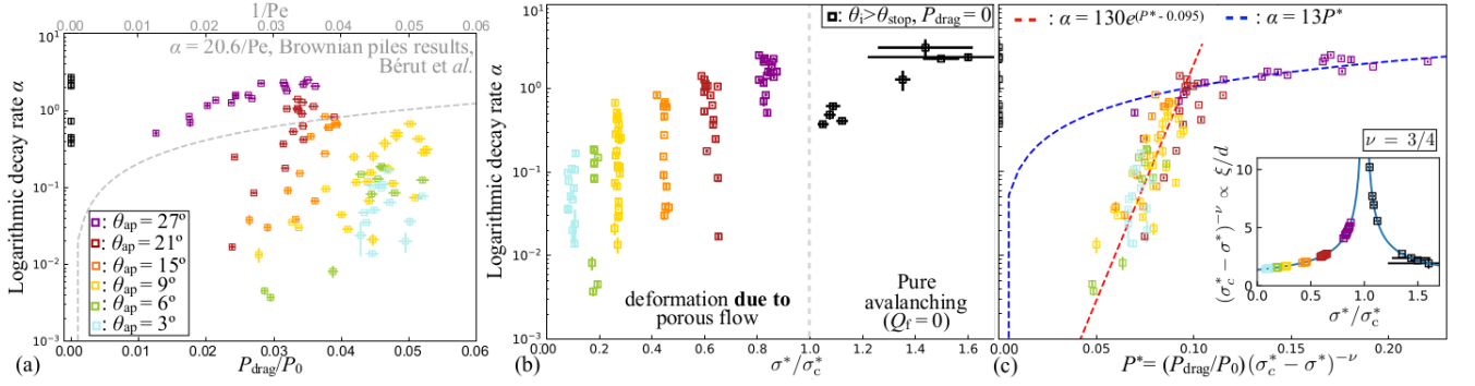
FIG. 3. Logarithmic decay of the surface slope of athermal pile ( 1/\text{Pe} = 10^{-9} ) with dimensionless time t^* , \alpha , (a) as a function of the normalized mean porous flow stress on particles, P_{\text{drag}}/P_0 . The dashed grey line shows results from experimental pile creep triggered by slight brownian agitation, where \alpha scales as \text{Pe}^{-1} . (b) \alpha as a function of the stress ratio \sigma^*/\sigma_c^* \simeq \tan \theta_i / \tan \theta_{\text{stop}} , and, (c) as a function of the parameter P^* defined in (1), using \nu = 3/4 . Red and blue dashed lines visually indicate an exponential and a linear trend respectively. Insert: values of (\sigma_c^* - \sigma^*)^{-3/4} reported as a function \sigma^*/\sigma_c^* in our experiments; the cyan line is the corresponding analytical form.
