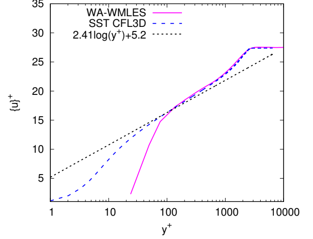
(b) Velocity profile scaled by the wall units.
