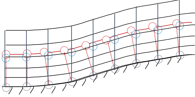
FIG. 1. An illustration depicting the non-orthogonal LES mesh, the closest LES mesh points (blue) to the exchange locations, and the boundary points for the RANS ODEs on the wall (black) and the exchange layer (red).
