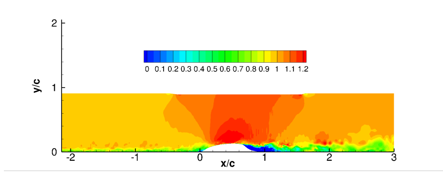
FIG. 12. The instantaneous streamwise momentum on the streamwise and wall normal plane for the hump flow.
