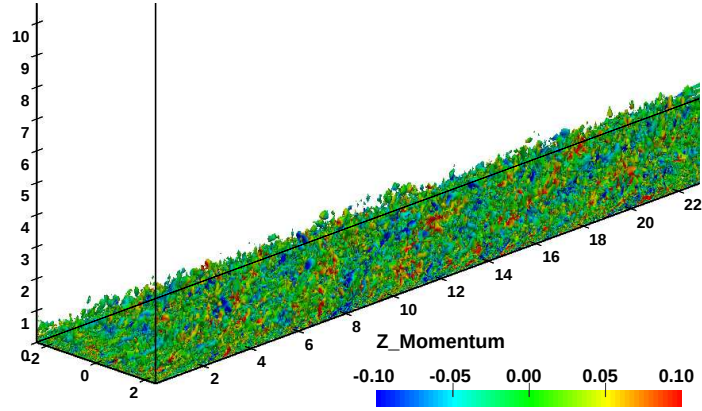
FIG. 5. The instantaneous Q-criterion isosurface colored by instantaneous spanwise momentum for the subsonic flat plate turbulent boundary layer flow. Axis labels are in the unit of the boundary layer thickness at the inflow.
