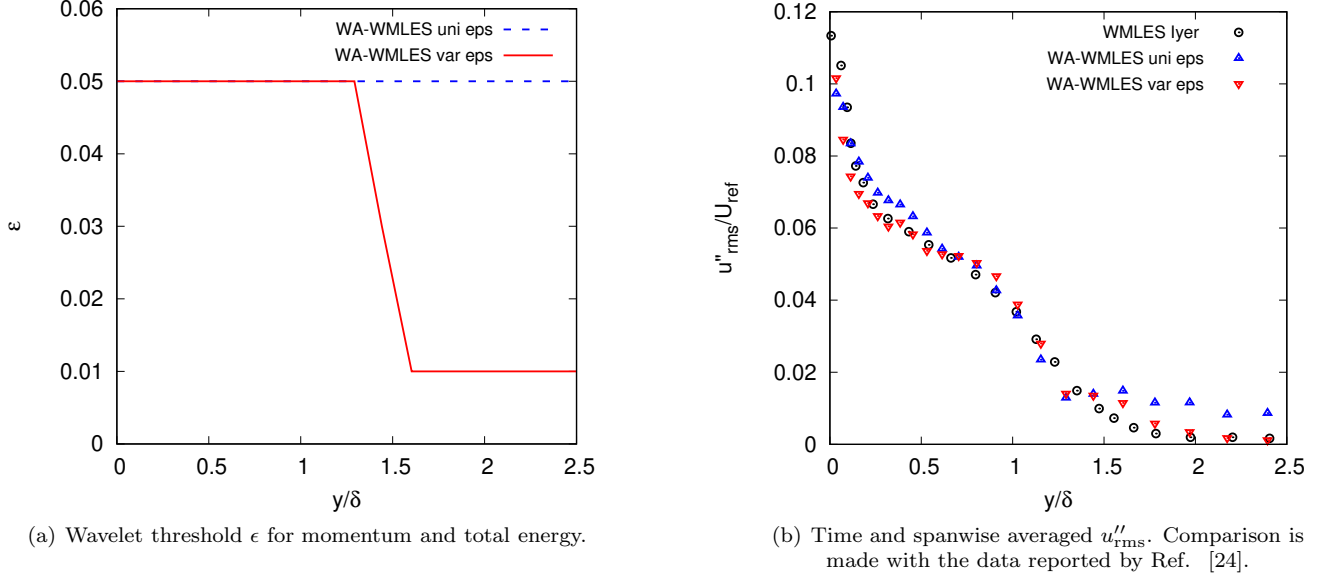
FIG. 2. Wall-normal profiles at a streamwise location x/\delta = 24 downstream of the inlet of the flat boundary layer case with uniform and zonal variable \epsilon for the WA-WMLES method.
