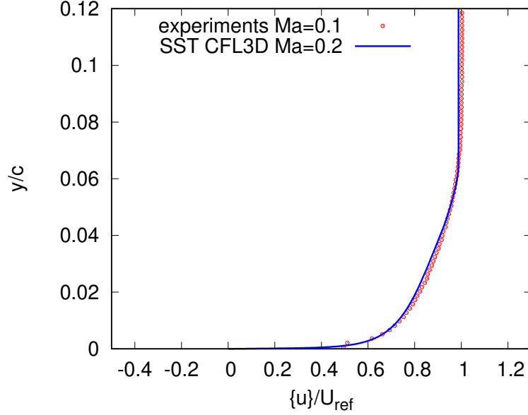
FIG. 8. Time and spanwise averaged streamwise velocity profile at the inflow plane x/c = -2.14 for the hump flow compared with the RANS data from the k - \omega SST model based RANS computation using CFL3D.
