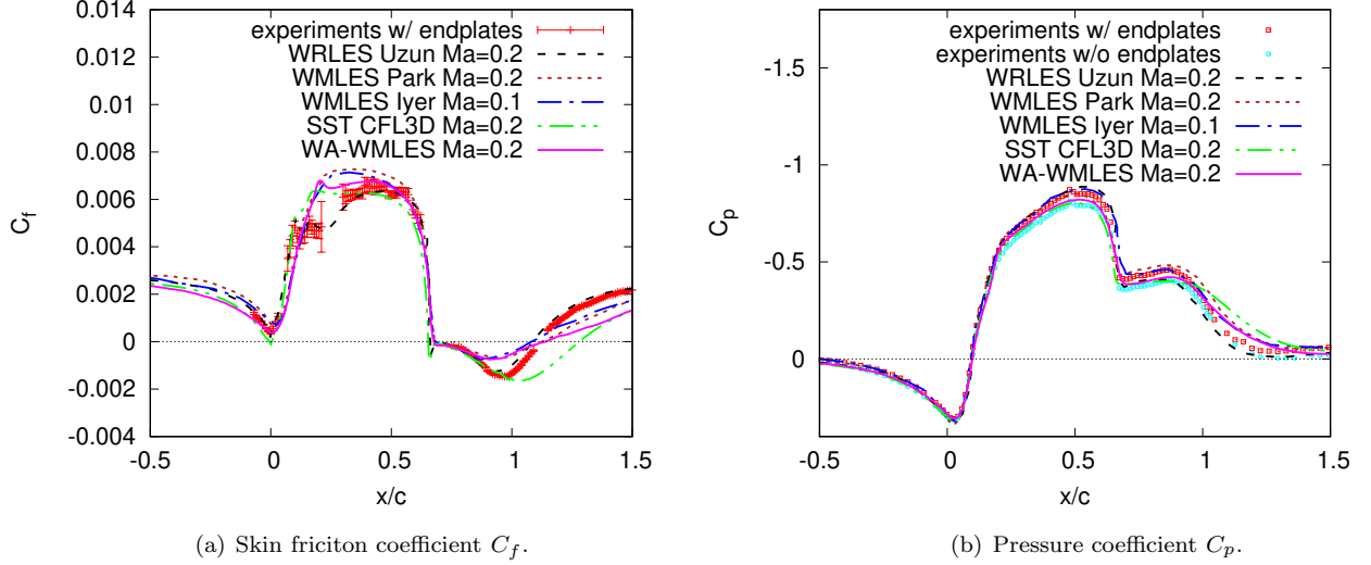
FIG. 15. Time and spanwise averaged skin friction and pressure coefficients over the wall for the hump flow. Comparison are made with the wall resolved LES data [46], non-adaptive WMLES results [35] and [24], the RANS data using the k - \omega SST model by CFL3D i.e., the initial condition of WA-WMLES, and the experimental data [23].
