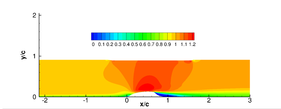
FIG. 14. The time and spanwise averaged streamwise momentum on the streamwise and wall normal plane for the hump flow.
