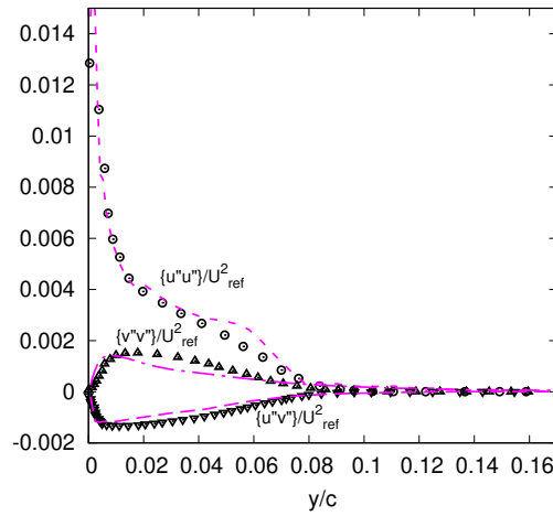
FIG. 17. Time and spanwise averaged profiles (lines) of turbulence fluctuation statistics at x/c = -0.81 for the hump flow compared with the non-adaptive WMLES case [24] (symbols).
