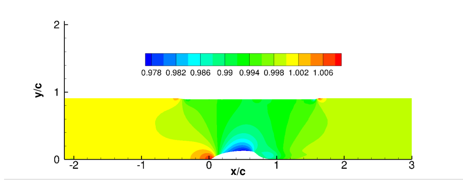
FIG. 13. The time and spanwise averaged pressure on the streamwise and wall normal plane for the hump flow.
