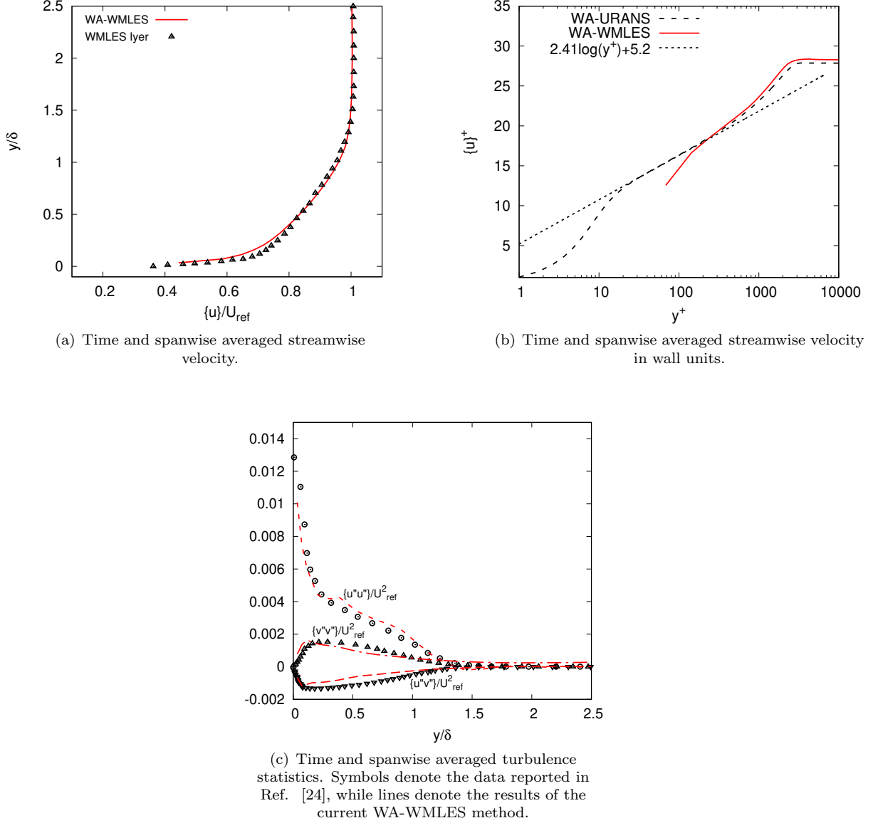
FIG. 7. The mean velocity profile and the turbulence statistics at a streamwise location x/\delta = 24 downstream of the inlet. Comparisons are made with the results of the inflow flat plate turbulent boundary layer in Ref. [24].
