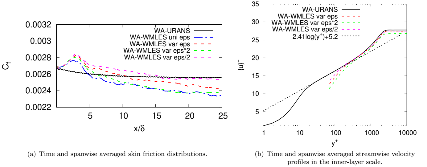
FIG. 3. Result comparison of the flat plate turbulent boundary layer case with uniform and different zonal variable \epsilon for the WA-WMLES method.
