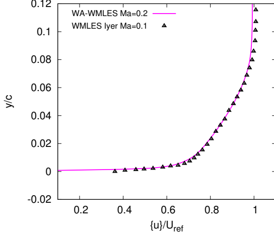
(a) Velocity profile scaled by the free-stream velocity.
