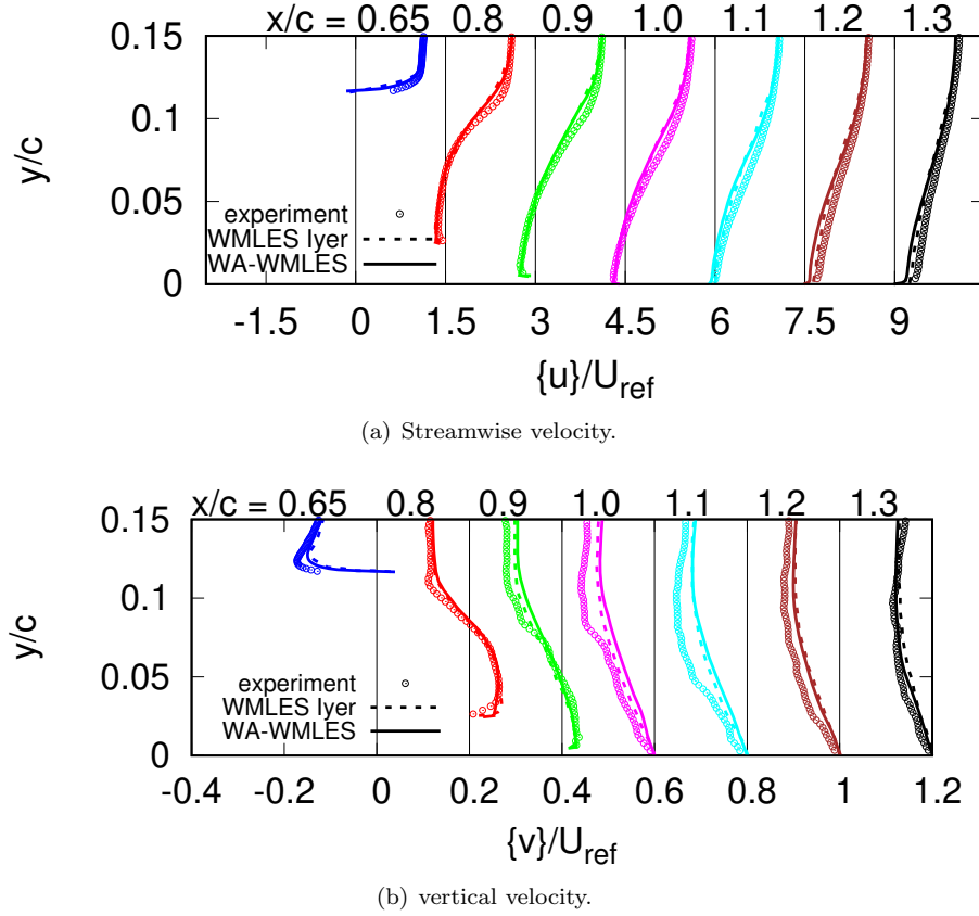
FIG. 18. Time and spanwise averaged velocity profiles at different streamwise locations. The experimental data [23] and those of the non-adaptive WMLES [24] are shown for comparison.
