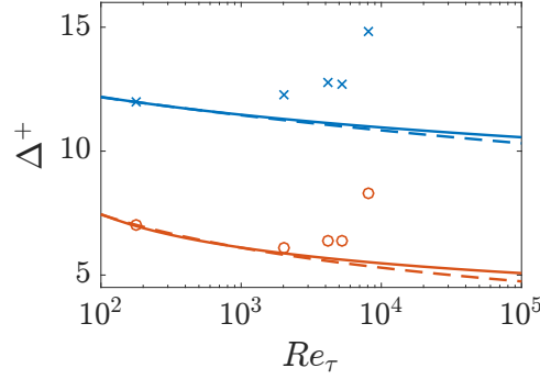
FIG. 5. The grid resolution required to resolve 99% of the wall-shear stress events. Blue lines: \Delta x^+ . Red lines: \Delta z^+ . Solid lines: assuming \sigma^{+2} \sim \log(Re_\tau) . Dashed lines: assuming \sigma^+ \sim \log(Re_\tau) . Cross symbols: \Delta x^+ in some of the channel flow DNSs. Round symbols: \Delta z^+ in some of the channel flow DNSs. The references are: for Re_\tau = 180 , Ref [3]; for Re_\tau = 2000 , Ref [41, 49]; for Re_\tau = 4200 , Ref [42]; for Re_\tau = 5200 , Ref [41]; and for Re_\tau = 8000 , Ref [48].
