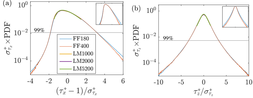
FIG. 4. Scaled PDFs of (a) the streamwise wall shear stress and (b) the spanwise wall shear stress in FF180, FF400, and the channel flow DNSs at Re_\tau = 1000, 2000 , and 5200 [41]. Details of the LM cases can be found in Ref [41]. As we will show later in this section, the rare events, i.e., the tails of the wall-shear stress PDFs, are not accurately predicted at higher Reynolds number if one uses the standard DNS grid resolution, and therefore the tails of the wall-shear stress PDFs for LM1000, LM2000, and LM5200 are not shown here. The plotted part of the PDFs integrates to 0.9. The two insets are un-scaled PDFs of the streamwise and the spanwise wall-shear stresses for FF180 and FF400. The two horizontal lines are at a constant \sigma_\tau^+ \times \text{PDF} location above which the PDF integrates to 0.99.
