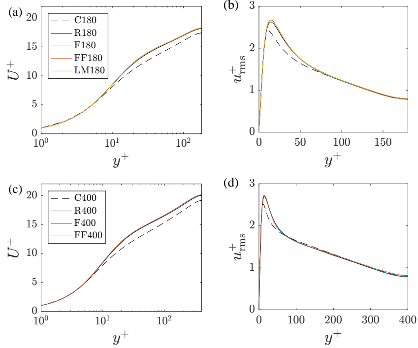
FIG. 1. (a, c) Mean velocity. (b, d) Streamwise velocity's rms. (a, b) Results at Re_\tau = 180 , (c, d) Results at Re_\tau = 400 .
