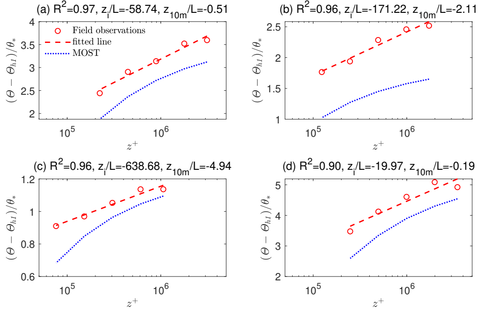
FIG. 3. Vertical profiles of normalized potential temperature in 4 different unstable conditions at the Cabauw Experimental Site for Atmospheric Research in Netherlands. R^2 denotes the coefficient of determination for the relation between \frac{\Theta - \Theta_{ht}}{\theta_*} and \log(z^+) , and z_{10m}/L denotes the stability parameter z/L at z = 10 m. “MOST” denotes the computed temperature profiles based on Monin-Obukhov similarity theory.
