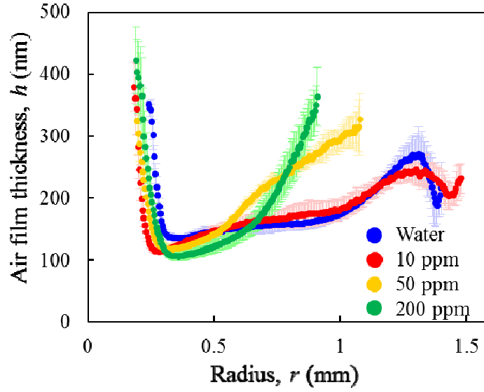
Figure 4. Air film shapes for various PEO concentrations at t \approx 3 ms from impact using TIRM for We \approx 9 . The error bars were obtained from three experiments.
