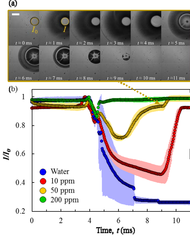
Figure 6. (a) The TIRM image sequence of a droplet with 50 ppm PEO. (b) The change in the averaged normalized intensity (across five separate droplet impacts, where the shaded areas are the error bars of one standard deviation), I/I_0 , at the droplet dimple center as a function of time for various PEO concentrations for We \approx 9 . The dotted arrow connects the TIRM image sequence to the processed data where I_0 is the average grayscale intensity at t=0 and I is the average grayscale intensity for each sequential frame. The scale bar represents 0.5 mm.
