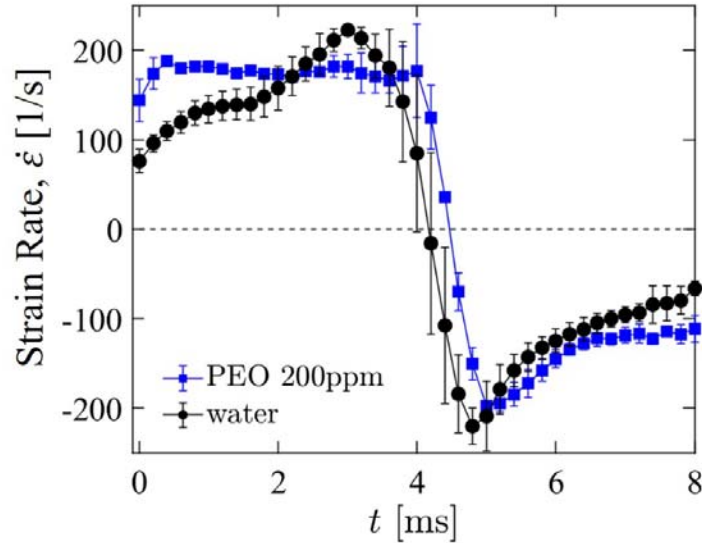
Figure 5. Particle tracking velocimetry (PTV) data showing the strain rate as a function of time for 200 ppm and water droplets for We \approx 6 . The time t = 0 is set as the beginning of the apparent impact with the surface and the start of the spreading phase of the droplet. The error bars were obtained from three experiments.
