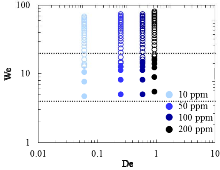
Figure 7. Phase diagram for droplet bouncing. The dotted lines indicate the inertia-capillary dominant regime for air film failure for pure water droplets. Beyond We > 20 , the contact is initiated by disjoining pressure [19]. Empty symbols represent no bouncing and solid symbols represent droplet bouncing for > 80 percent of the tests. Half-filled symbols represent < 50 percent of the droplets bounced. At least 100 impact tests were conducted for the solid symbols and the transitional data points below We < 20 .
