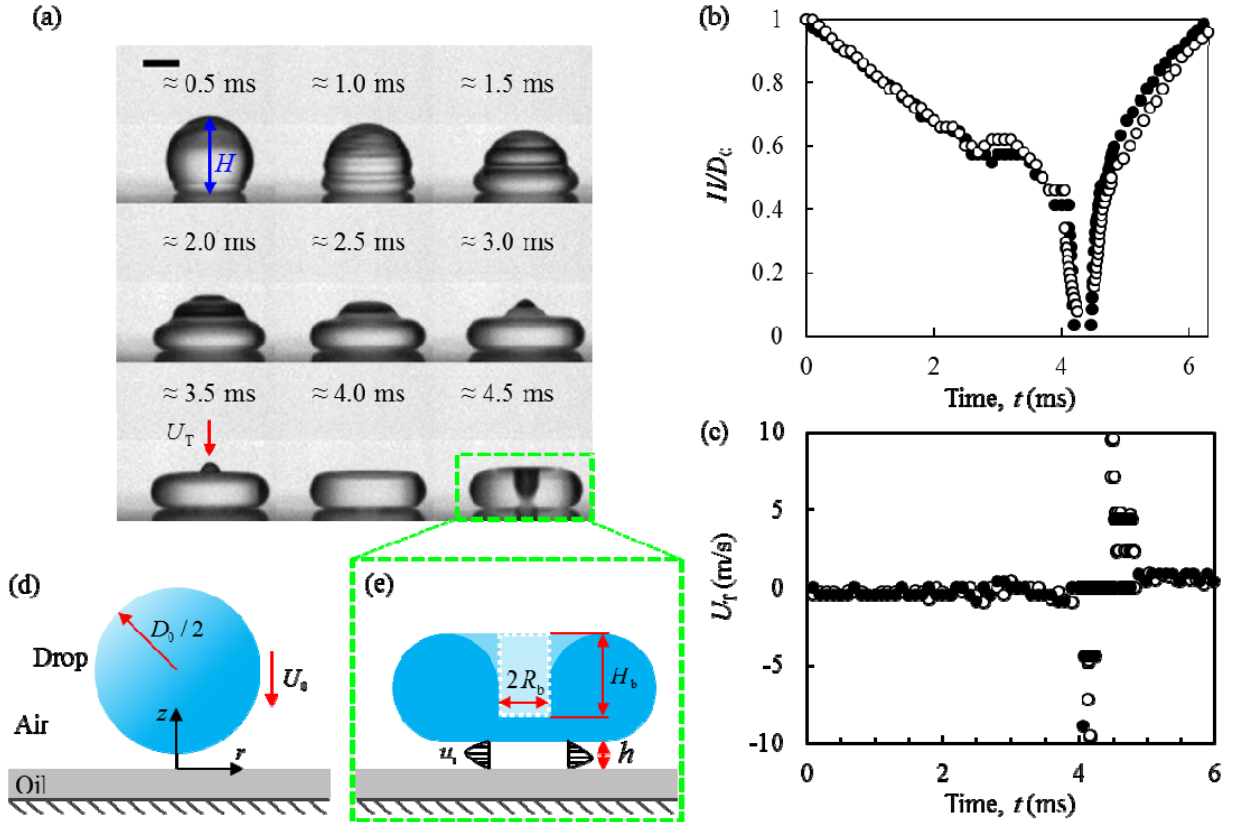
Figure 3. (a) Droplet impact showing capillary wave propagation as a function of time. The red arrow indicates the final wave prior to the inversion of the droplet top surface, which occurs
