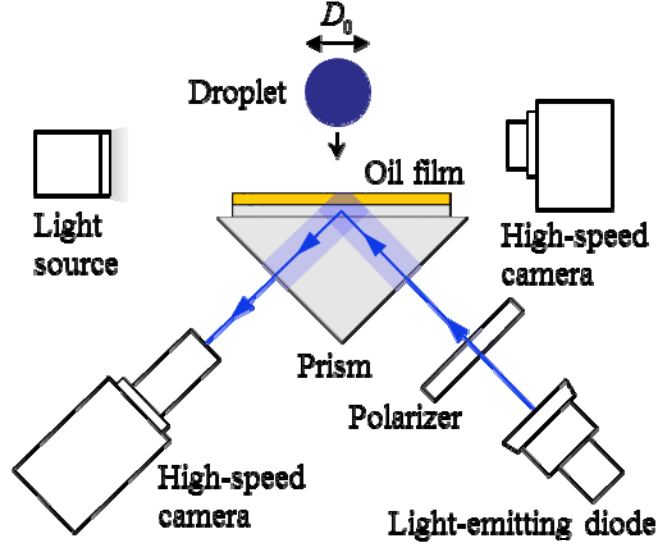
Figure 1. Experimental schematic of the total internal reflection microscopy (TIRM) technique for studying droplet impact on a substrate.
