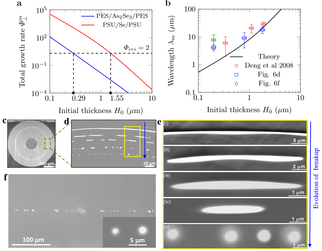
FIG. 6. Fiber applications. (a, b) Theoretical predictions agreeing with experimental data. (a) \Phi_{\perp}^m for PES/As 2 Se 3 /PES and PSU/Se/PSU, the dashed line for \Phi_{cri} = 2 . (b) For PSU/Se/PSU, the predicted wavelength agreeing with the measured wavelength (Deng et al 2008: [11]). (c-e) SEM imaging for evolution of instability and breakup for five final targeted film thickness of 300, 170, 90, 40 and 10 nm, respectively. (f) SEM imaging for a ribbon-fiber cross-section for a final targeted 10-nm-thick film, and its inset presenting the circular shapes. Dark color for PSU, bright color for Se, and arrow indicating the decreased targeted thickness.
