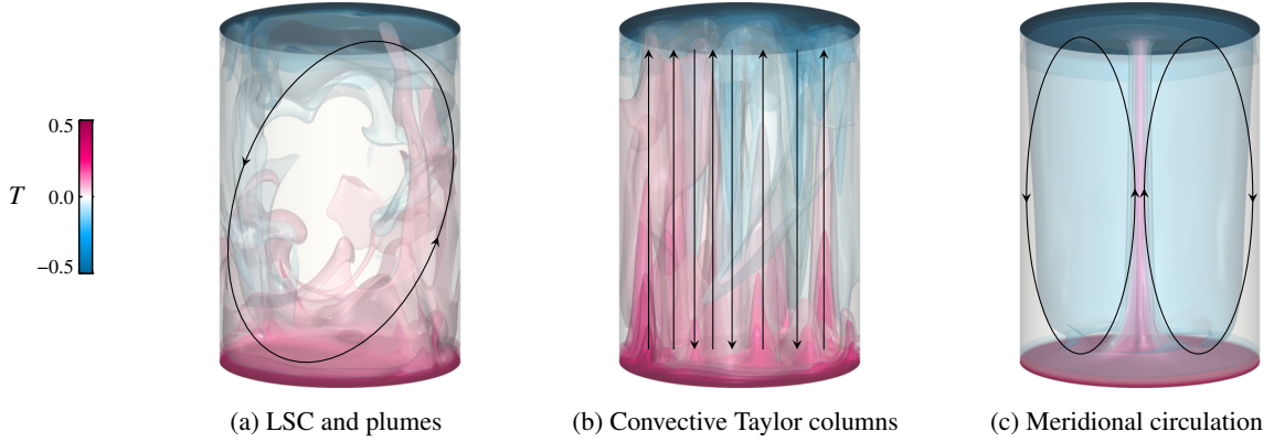
FIG. 2. Prototypal flow components in Coriolis-centrifugal convection. Shown are temperature isosurfaces for Ra = 10^8 . The respective flow configuration is sketched with black lines and arrows demarcating (a) the large-scale circulation with mushroom-like plumes ( Ro_{\parallel} = \infty , Fr = 0 ); (b) the space-filling convective Taylor columns ( Ro_{\parallel} = 0.05 , Fr = 0 ); (c) the donut-shaped, axisymmetric meridional circulation ( Ro_{\parallel} = \infty , Fr = 0.5 ). (See Fig. 5 for their respective 2D slices.)
