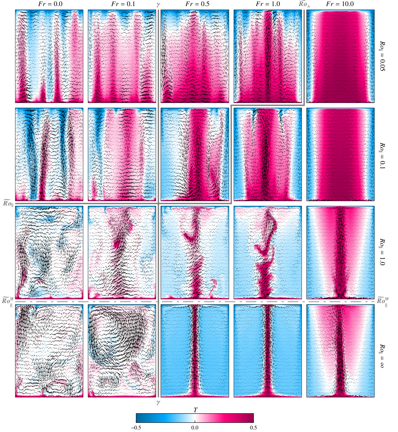
FIG. 5. Instantaneous vertical cross-sections of the temperature field with overplotted velocity vectors for fixed Ra = 10^8 , Pr = 6.52 and \gamma = 0.365 . Ro_{\parallel} \in \{\infty, 1.0, 0.1, 0.05\} decreases from bottom to top, characterizing the increasing Coriolis force, Fr \in \{0.0, 0.1, 0.5, 1.0, 10.0\} increases from left to right, characterizing the increasing centrifugal buoyancy force. Fr = 0.0 corresponds to zero centrifugal force, Ro = \infty to zero Coriolis force cases. The predicted regime boundaries according to Horn and Aurnou [1] are marked with the gray lines, where the full vertical line corresponds to Fr = \gamma , the full horizontal line to \widetilde{Ro}_{\parallel} = 0.1 and the zig-zag line to \widetilde{Ro}_{\perp} = 0.1 according to Eqs. (11). The dash-dotted line is the prediction by Weiss et al. [31], given by Eq. (8).
