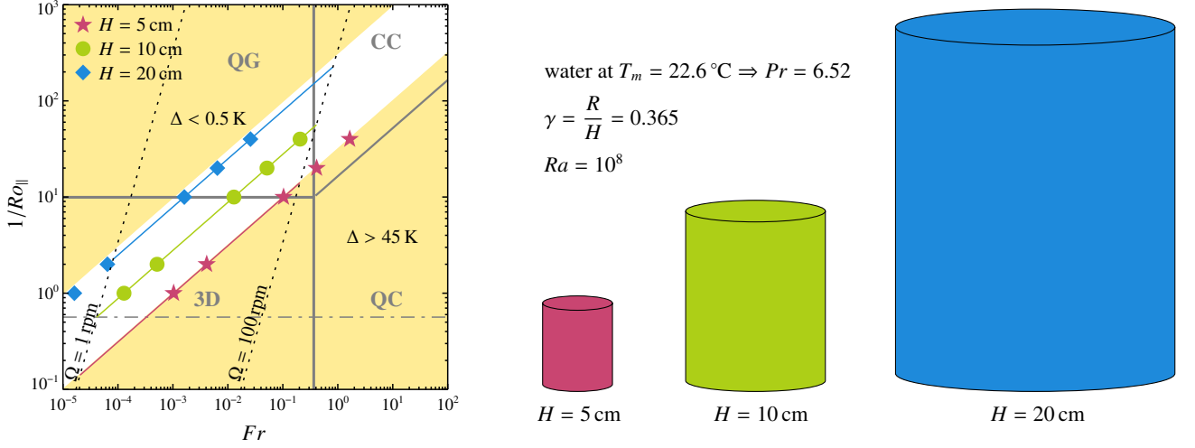
FIG. 3. Regime diagram for water at a mean temperature of T_m = 22.6^\circ\text{C} , corresponding to Pr = 6.52 , and a fixed aspect ratio of \gamma = 0.365 and Rayleigh number of Ra = 10^8 , as in our DNS. The regime boundaries according to the Eqs. (11) and (12) are marked by the grey solid lines. The transition to weakly Coriolis affected flows according to Eq. (8) is marked by the grey dash-dotted line. In laboratory experiments the accessible range is given by the maximum employable temperature difference \Delta and rotation rate \Omega . Here we assume 0.5\text{ K} \leq \Delta \leq 45\text{ K} and 1\text{ rpm} \leq \Omega \leq 100\text{ rpm} . The intimate relation of Ro_{\parallel} and Fr through Ro_{\perp} (Eq. (7)) and consequently \Delta restricts the permissible range to values within the white strip, i.e. within Ro_{\perp} = \sqrt{\alpha\Delta/2} = 5.4 \times 10^{-3} and 5.1 \times 10^{-2} , the upper yellow area indicates \Delta < 0.5\text{ K} and the lower yellow are \Delta > 45\text{ K} . Furthermore, \Omega restricts the range through the definition of Fr and Ro_{\parallel} and assuming \Delta = Ra \kappa \nu / (\alpha g h^3) , where h are all possible heights. The pink, green, and blue lines show the theoretical values for three different virtual convection cells of fixed heights 5 cm, 10 cm, and 20 cm and 1\text{ rpm} \leq \Omega \leq 100\text{ rpm} within the Ro_{\parallel} - Fr space. For fixed Ra , only experiments along isolines of Ro_{\perp} are possible. For DNS there are no restrictions in the Ro_{\parallel} - Fr space, including the possibilities ( Ro_{\parallel} = \infty, Fr \neq 0 ) and ( Ro_{\parallel} < \infty, Fr = 0 ). The symbols correspond to Ro_{\parallel} \in \{0.025, 0.05, 0.1, 0.5, 1.0\} that are studied here with DNS mapped to the virtual convection tanks.
