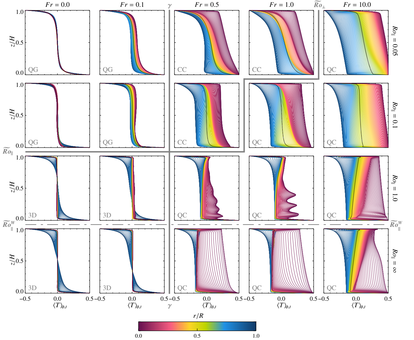
FIG. 6. Azimuthally and temporally averaged temperature profiles \langle T \rangle_{\phi,t} . The color indicates the radial position where the profile is obtained, ranging from the center, r/R = 0.0 , to the sidewall, r/R = 1.0 . The black solid lines demarcate the plane-averaged temperature profile \bar{T}(z) = \langle T \rangle_{t,r,\phi} . Ro_{\parallel} \in \{\infty, 1.0, 0.1, 0.05\} decreases from bottom to top, Fr \in \{0.0, 0.1, 0.5, 1.0, 10.0\} increases from left to right. The gray lines correspond to the regime boundaries as in Fig. 5.
