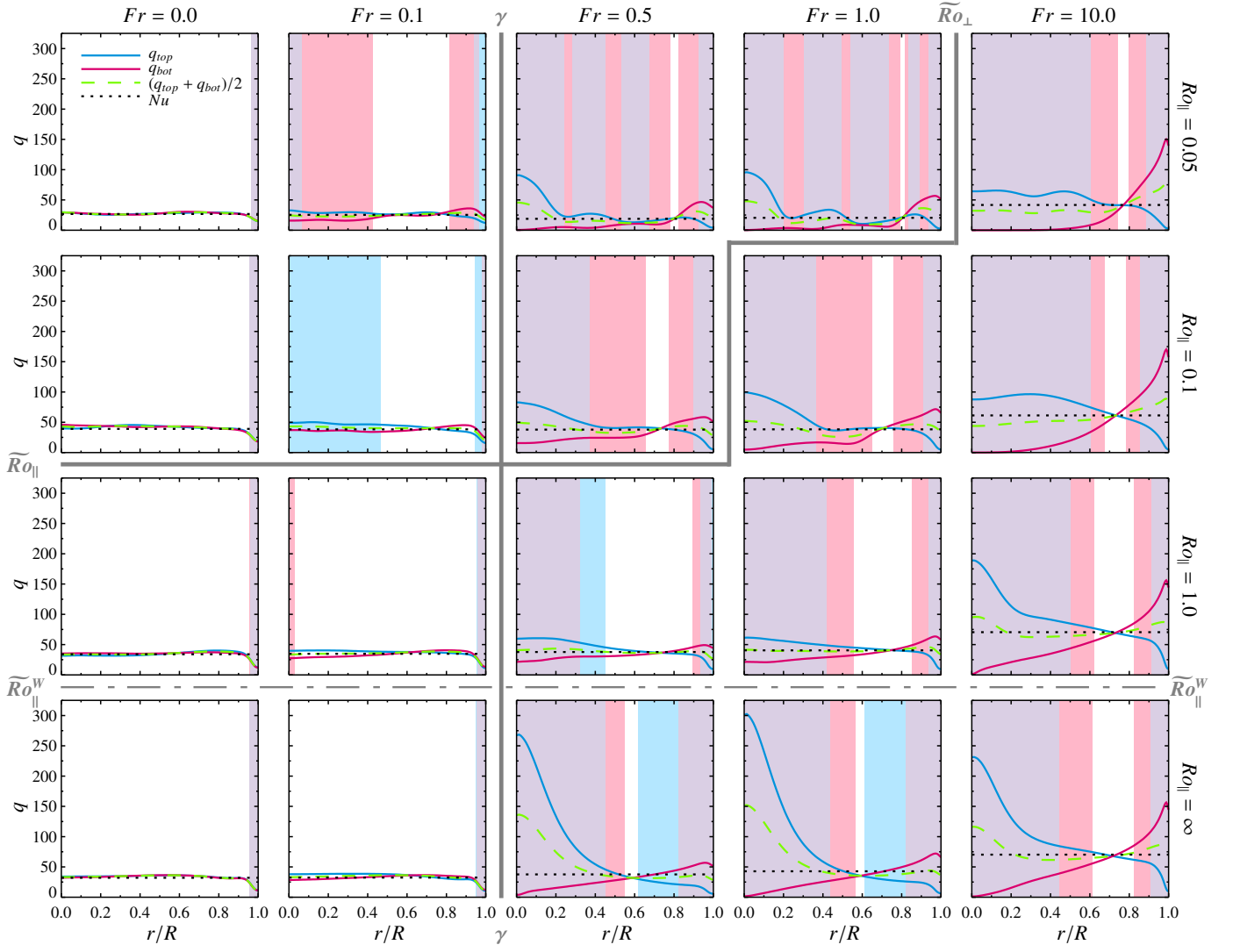
FIG. 9. Local heat fluxes q_{top} (blue line) and q_{bot} (pink line), based on the temperature gradient at the top and bottom plate, respectively. The green long-dashed indicates the average (q_{top} + q_{bot})/2 . The dotted black line shows the Nusselt number Nu for comparison. The blue shaded area indicates where |q_{top} - Nu|/Nu > 0.2 and the pink area where |q_{bot} - Nu|/Nu > 0.2 . Note that purple shading means both local heat fluxes deviate from Nu with more than \pm 20\% .
