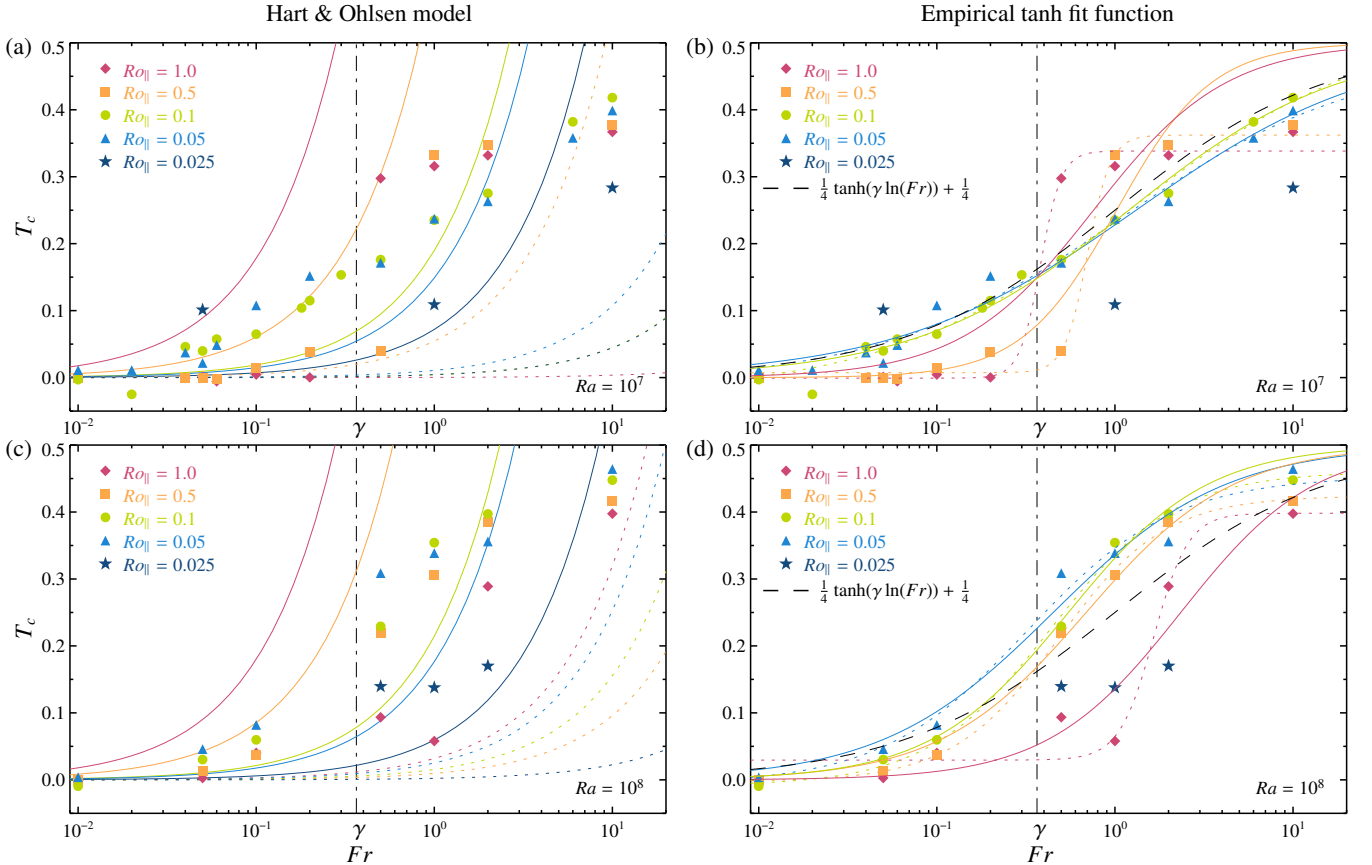
FIG. 8. (a,c) Comparison of the Hart and Ohlsen [2] model and the center temperature T_c obtained by our DNS as function of Fr . The filled symbols mark T_c^a \equiv \langle T(r=0, z=H/2) \rangle_t from our DNS; the solid lines mark the full Hart and Ohlsen [2] model, and the dotted lines the simplified version given by Eq. (20); (a) Ra = 10^7 , (c) Ra = 10^8 . (b,d) The filled symbols are identical to (a); the solid lines correspond to the best fit with four free parameters, Eq. (21); the dotted lines correspond to the best fit with two free parameters, Eq. (22). The black dashed line correspond to the empirical function (23); (b) Ra = 10^7 , (d) Ra = 10^8 .
