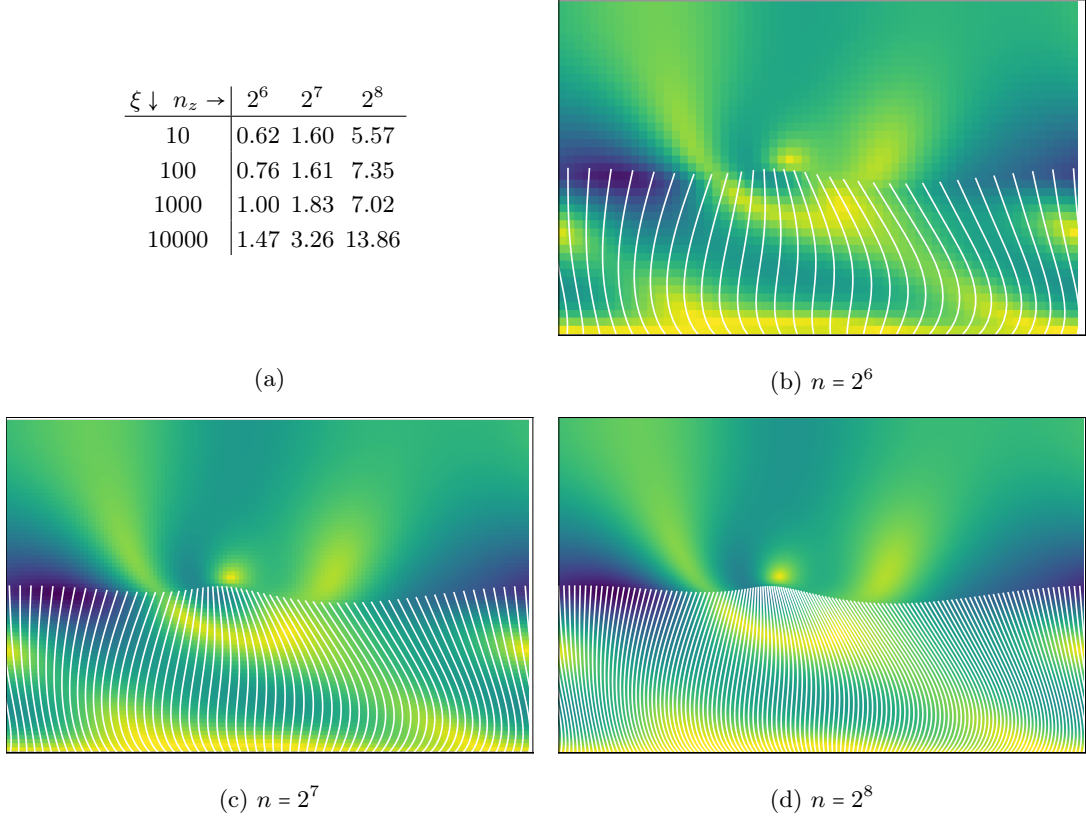
Figure 12: Numerical performance and accuracy in two dimensions. Panel (a) shows the wall clock time-per-timestep, in seconds, measured as the average over the first ten timesteps after t = 1 , for a range of densities and discretizations. Panel (b) through (d) show fiber deformation (in white) and velocity magnitude (color scale, larger magnitudes are darker) at time t = 5 , for coarser (b) to finer (d) discretizations. All discrete fibers used in the computation are shown.
