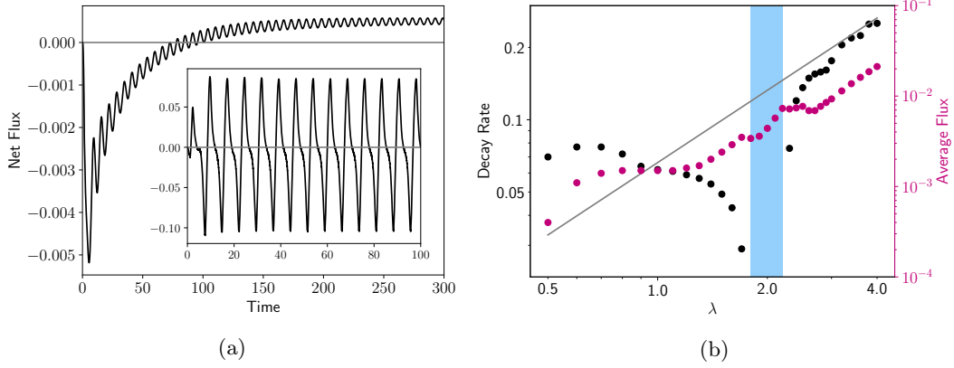
Figure 13: Panel (a) shows the transient behavior and decay of oscillations in the net flux due to small amplitude ( \gamma = 0.01 ) actuation. The density and effective rigidity for the main figure are \xi = 100 and \tilde{E} = 10^{-4} , respectively, and thus \lambda = \xi\tilde{E} = 0.01 . Transient behavior relaxes with a timescale \lambda^{-1} = 100 , while a persistent oscillation at the driving frequency damps with the timescale 2\pi\lambda^{-1} . The inset shows the net flux at large amplitude ( \gamma = \pi/4 ) and in the pulsatile regime ( \lambda = 2 ). In this case, the persistent oscillations are large and do not decay. Panel (b) shows the rate of decay of the persistent oscillations for large amplitude ( \gamma = 0.5 ) actuation with \xi = 1000 over a range of \tilde{E} . Although both the decay rate and flux scale with \lambda for large \lambda , a pulsatile regime exists in a range about \lambda \approx 2 in which these oscillations do not decay.
