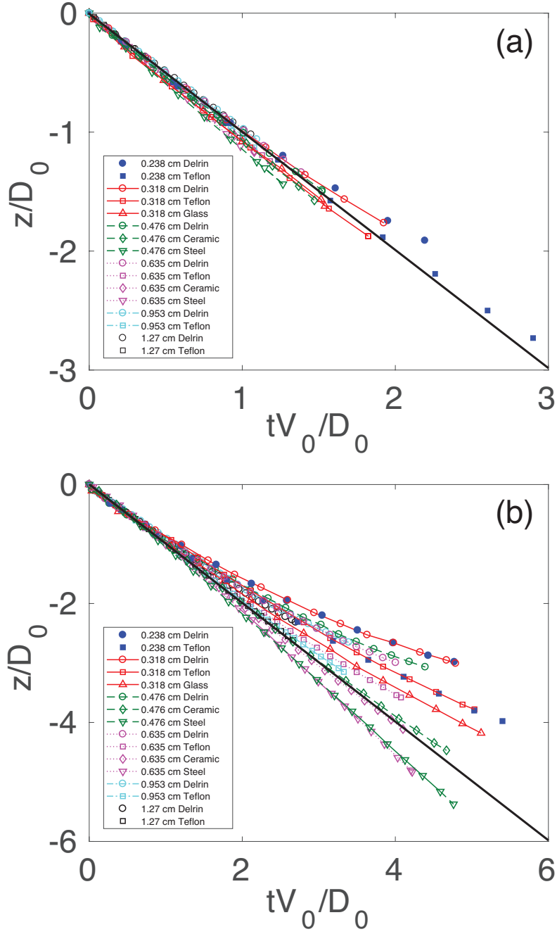
FIG. 8. Sphere trajectory after impact in the (a) water experiments and (b) oil lens experiments with sphere depth normalized by its diameter and time from impact by V_0/D_0 . Symbols: \circ (delrin, \mathcal{D} = 1.35 ), \square (teflon, \mathcal{D} = 2.13 ), \triangle (glass, \mathcal{D} = 2.41 ), \diamond (ceramic, \mathcal{D} = 3.25 ) and \nabla (steel, \mathcal{D} = 7.79 ) for spheres of radii 0.238 cm (solid symbols), 0.318 cm (solid line), 0.476 cm (dashed line), 0.635 cm (dotted line), 0.953 cm (dotted-dashed line) and 1.27 cm (open symbols). The thick line is the trajectory under constant speed V_0 .
