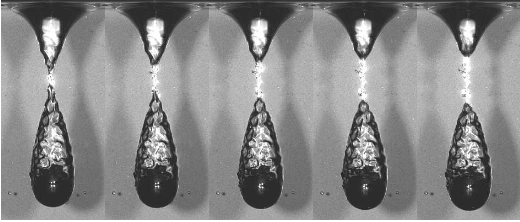
FIG. 6. Formation of oil filament after cavity collapse by deep seal closure for the experiment shown in Fig. 1(b) of a steel sphere of radius 0.635 cm. Time from impact: 54.3, 55.0, 55.7, 56.3 and 57.0 ms. Supplementary movie available online.
