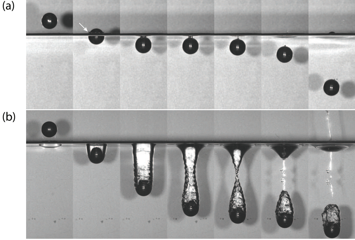
FIG. 1. Comparison of a steel sphere of radius 0.635 cm entering water at impact speed 1.0 \text{ m s}^{-1} and \text{Fr} = 16.1 with (a) a clean free surface, and (b) passing through an oil lens of radius 0.915 cm (left-most image). Time from impact and parameters: (a) -6.2, 5.3, 11.3, 12.0, 12.8, 17.6, 38.5 ms, \text{Bo} = 5.4 , \text{Ca} = 1.4 \times 10^{-2} , \text{Re} = 6.35 \times 10^3 , \text{We} = 87.2 ; (b) -6.0, 14.0, 36.2, 49.5, 54.1, 56.8, 63.2 ms, \text{Bo} = 7.8 , \text{Ca} = 9.0 \times 10^{-1} , \text{Re} = 139 , \text{We} = 125 . The arrow in (a) indicates the climbing water film. Supplementary movies are available at (publisher provides weblink)[28].
