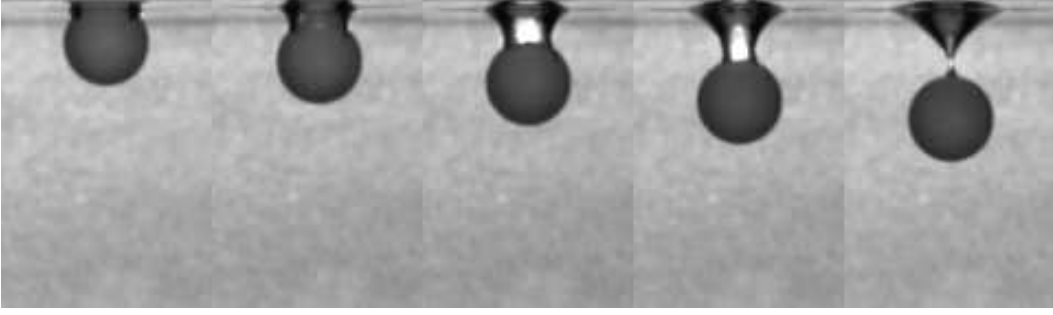
FIG. 3. A quasi-static cavity attached to a delrin sphere of radius 0.318 cm entering water at times 5.8, 7.5, 9.2, 10.8 and 12.5 ms from impact with V_0 = 1.0 \text{ m s}^{-1} , Bo = 1.4 , Ca = 1.4 \times 10^{-2} , Fr = 32.1 , Re = 3.18 \times 10^3 and We = 43.7 . The quasi-static cavity shown in panel 5 can be compared to the air cavity in the corresponding oil lens experiment shown in Fig. 4(c).
