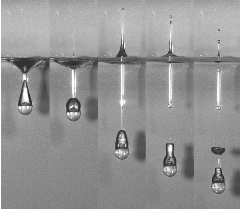
FIG. 12. Dynamics after pinch-off of an air cavity formed by a 0.318 cm radius glass sphere in the oil lens experiment shown in Fig. 4(e) at times 33.3, 38.0, 69.6, 85.1, 101.2 ms from impact with lens radius 0.965 cm, Bo = 2.0 , Ca = 9.0 \times 10^{-1} , Fr = 32.1 , Re = 69.6 , We = 62.5 . Supplementary movie available online.
