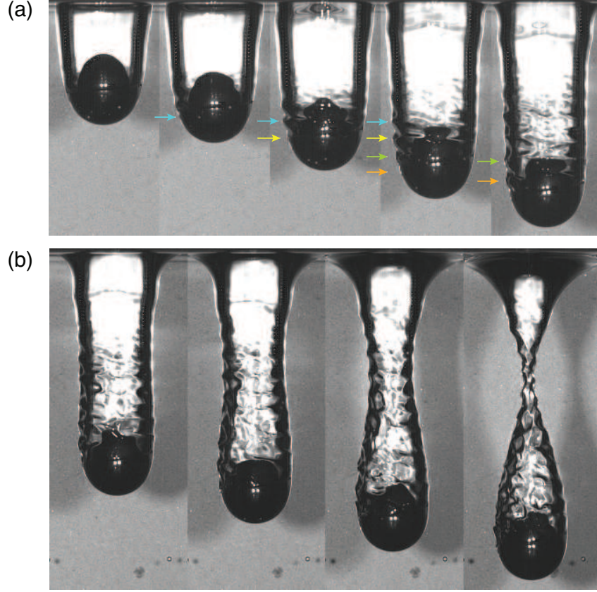
FIG. 13. (a) Shear-induced perturbations that develop along the lower hemisphere generate interfacial waves at the contact line that perturb the cavity wall (colored arrows track a few examples), (b) then take on a three-dimensional form as the cavity contracts under hydrostatic pressure corresponding to the oil lens experiment shown in Fig. 1(b) with a 0.635 cm radius steel sphere. Time from impact: (a) 20.0, 22.9, 27.3, 31.7, 36.1, and (b) 40.6, 45.1, 49.5, 53.9 ms. Supplementary movie available online.
