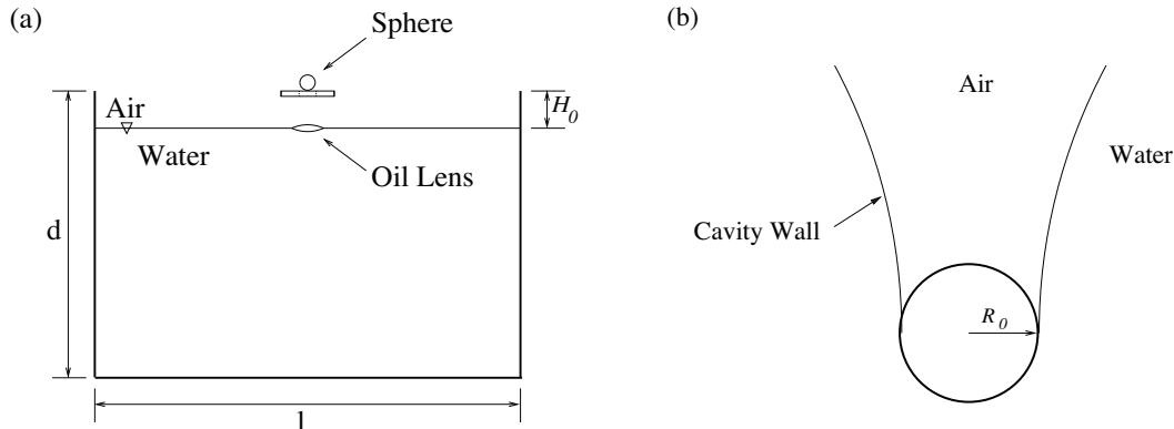
FIG. 2. (a) Schematic of experimental setup with an open top water tank, sphere and oil lens. The sphere is dropped from rest through a 1.2 cm thick sleeve to ensure vertical entry. (b) After impact a thin film of oleic acid lines the lower hemisphere and cavity wall in the oil lens experiments.
