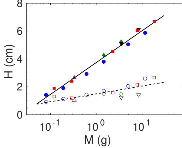
FIG. 11. Sphere depth at pinch-off versus sphere mass with H \approx 0.57 \log(M) (dashed line) and H \approx 2.29 \log(M) (solid line). Symbols: delrin ( \circ ); teflon ( \square ); glass ( \triangle ); ceramic ( \diamond ); steel ( \nabla ); water experiments (open symbols); oil lens experiments (filled symbols).
