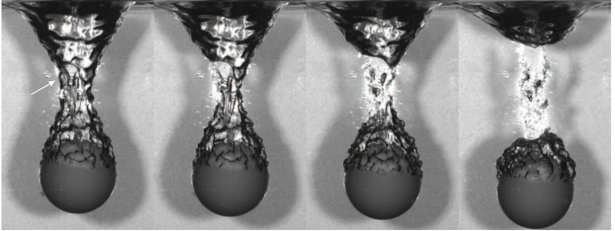
FIG. 7. Rupture of air cavity formed by a 1.27 cm radius teflon sphere in the oil lens experiment shown in Fig. 4(p) at times 72.5, 73.6, 74.7, and 78.0 ms from impact with lens radius 1.19 cm, Bo = 31.2 , Ca = 9.0 \times 10^{-1} , Fr = 8.0 , Re = 278 , We = 249 . The arrow is directed towards a hole that separates the cavity into two subcavities. Supplementary movie available online.
