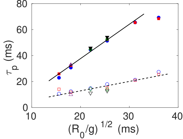
FIG. 10. Pinch-off time versus predicted scaling \sqrt{R_0/g} with \tau_p \approx 0.72\sqrt{R_0/g} (dashed line) and \tau_p \approx 2.64\sqrt{R_0/g} (solid line). Symbols: delrin (o); tefflon (□); glass (Δ); ceramic (◇); steel (▽); water experiments (open symbols); oil lens experiments (filled symbols).
