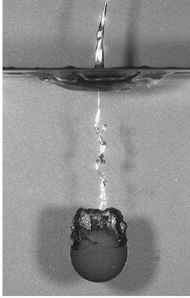
FIG. 16. The oil film that lines the air cavity wall before rupture in Fig. 4(m) dewets from the upper air cavity wall after rupture with the leading edge of the oil film forming a fingering pattern as the cavity retracts to form a Worthington jet. Image is of a 0.953 cm radius teflon sphere 77.3 ms after impact with Bo = 17.5 , Ca = 9.0 \times 10^{-1} , Fr = 10.7 , Re = 209 , We = 187 . See the supplementary movie to Fig. 14.
