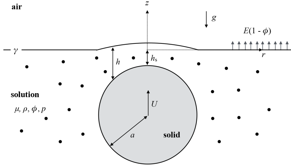
Figure 2: Schematic of the model geometry.
