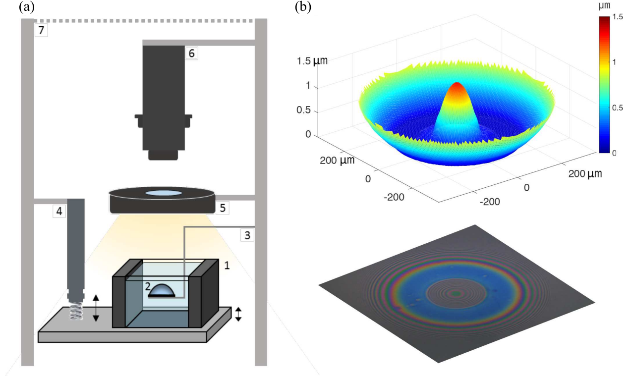
Figure 1: (a) The Dynamic Fluid-Film Interferometer (DFI), a custom-built apparatus [39], is used to create thin liquid films between a spherical solid substrate and an initially planar free surface. Labeled components in the figure correspond to: 1) Delrin chamber, 2) fused-silica substrate, 3) substrate holder, 4) motorized actuator, 5) light source, 6) top camera, 7) DFI cover. (b) Bottom: white-light interferometry is used to map color images recorded from the top camera to film thickness profiles. Top: an image-processing script is used to visualize the spatiotemporal evolution of the entrained liquid film.
