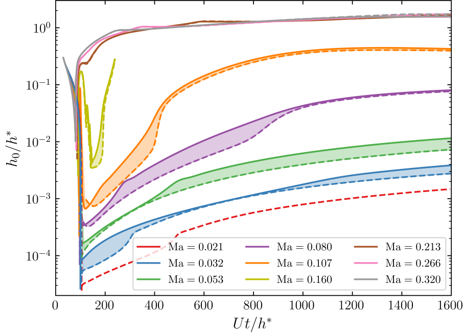
Figure 7: Plot of the theoretical centerline film thickness \bar{h}_0 = h(0, t)/h^* against time \bar{t} for several values of the Marangoni number \text{Ma} = 0.021 - 0.320 ( \phi_\infty = 0.02\% - 0.30\% ). The solid lines correspond to \text{Ha} = 1.6 \times 10^{-5} , the dashed lines correspond to \text{Ha} = 1.6 \times 10^{-6} , and the region in between two curves of the same color is shaded to guide the eye. The other dimensionless parameters are \text{Ca} = 2.4 \times 10^{-6} , \text{Pe} = 10^3 , \text{Bo} = 4.3 \times 10^{-2} , and \text{Ev} = 2.6 \times 10^{-3} , corresponding to a 1.00 cSt/5.00 cSt mixture (reported in Table II).
