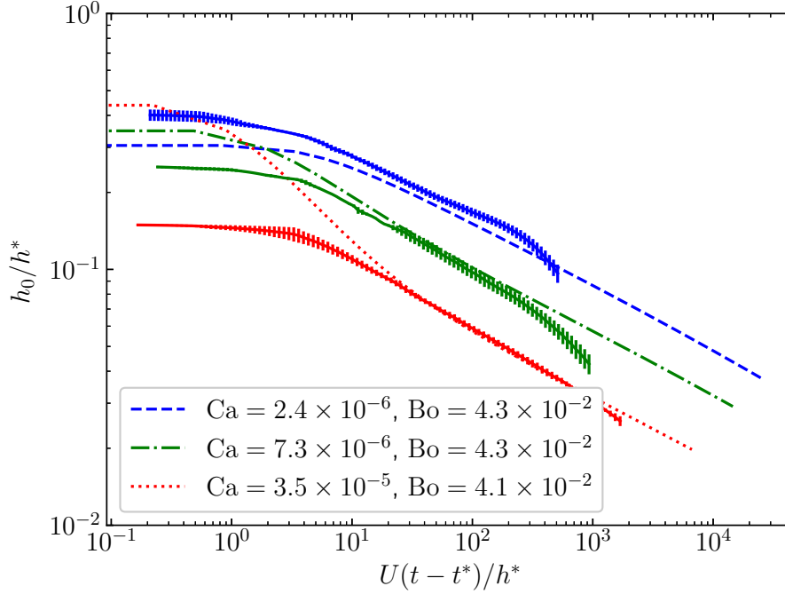
Figure 3: (Color online) Comparison of the numerical computations (dashed lines) to experimental measurements (solid lines) for pure silicone fluids in the absence of evaporation. Lines and error bars in the experimental data represent the mean and standard deviation, respectively, of repeated measurements (duplicates or triplicates). Blue data: \nu = 1 cSt, U = 0.05 mm/s, t^* = 7 s, and b = 0.3 mm. Green data: \nu = 1 cSt, U = 0.15 mm/s, t^* = 2.3 s, and b = 0.3 mm. Red data: \nu = 5 cSt, U = 0.15 mm/s, t^* = 2.3 s, and b = 0.3 mm.
