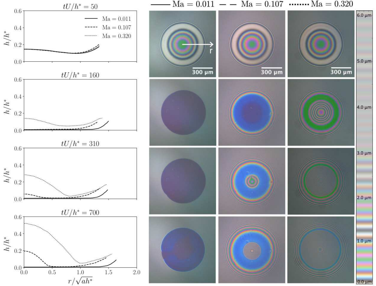
Figure 4: Time series of experimental film thickness profiles are plotted for 1.00 cSt/5.00 cSt blends ( Ev = 2.6 \times 10^{-3} ) at Ma = 0.011 ( \phi_\infty = 0.01\% ), Ma = 0.107 ( \phi_\infty = 0.10\% ), and Ma = 0.320 ( \phi_\infty = 0.30\% ), as determined experimentally. Snapshots of the interferometric patterns, viewed from the top camera, are shown at the corresponding times and compositions. Experiments show the presence of three distinct flow regimes: the van der Waals regime (solid line), the intermediate regime (dashed line), and the capillary regime (dotted line).
