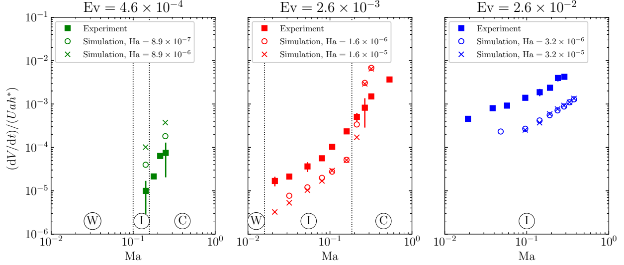
Figure 8: Experimental and simulation data of the dimensionless mound volume flux d\bar{V}/d\bar{t} = [1/(ah^*U)](dV/dt) against Ma for 1.50 cSt/10.0 cSt ( Ev = 4.6 \times 10^{-4} ), 1.00 cSt/5.00 cSt ( Ev = 2.6 \times 10^{-3} ), and 0.65 cSt/5.00 cSt ( Ev = 2.6 \times 10^{-2} ) mixtures. Other relevant dimensionless parameters appear in Table II. The symbols (W), (I), and (C) stand for the van der Waals, the intermediate, and the capillary regimes, respectively. The solid squares (■) correspond to experimental measurements, and the error bars represent the standard deviation obtained from multiple datasets. In all of the experimental measurements reported, the dimensionless mound volume \bar{V} increases linearly with time. For each value of Ev in the simulations, two values of Ha are shown for comparison. Simulation data is shown by circles (○) for low Ha and by crosses (×) for high Ha . In the numerical computations, \bar{V} typically increases nonlinearly with time; thus, the symbols represent the finite-difference approximant of d\bar{V}/d\bar{t} at \bar{t} = \bar{t}_M , the inception point of mound formation.
