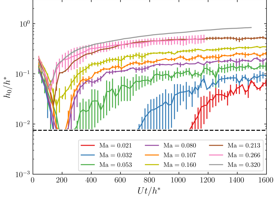
Figure 6: Plot of the experimental centerline film thickness \bar{h}_0 = h(0, t)/h^* against time \bar{t} for a 1.00 cSt/5.00 cSt mixture ( Ev = 2.6 \times 10^{-3} ) at several values of the Marangoni number Ma = 0.021 - 0.320 ( \phi_\infty = 0.02\% - 0.30\% ). The other dimensionless parameters for a 1.00 cSt/5.00 cSt mixture are reported in Table II. Experimental data cannot be obtained for thicknesses below the dotted line at \bar{h} \simeq 7.5 \times 10^{-3} ( h \simeq 90 nm). Error bars represent the standard deviation obtained from multiple datasets.
