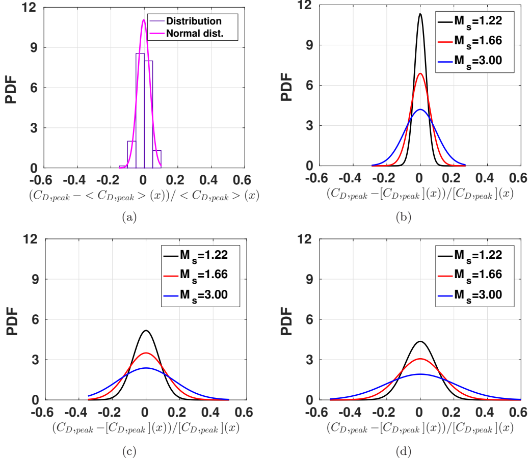
FIG. 13: Plot of normal distribution fit for fluctuating peak drag coefficient for (a) M_s = 1.22 and \phi_1 = 2.5\% , (b) \phi = 2.5\% , (c) \phi = 10\% , and (d) \phi = 20\% .
