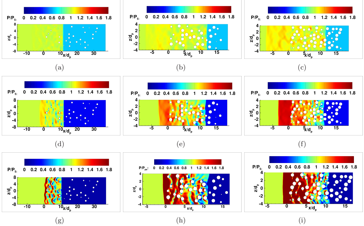
FIG. 4: Contour plot of non-dimensional pressure at t/\tau = 12 along the x - z plane at y = 0 for \phi_1 = 2.5, 10 , and 20\% and (a-c) M_s = 1.22 , (d-f) M_s = 1.66 , and (g-i) M_s = 3 , respectively.
