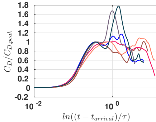
FIG. 11: Plot of normalized drag coefficient, C_D/C_{D,peak} , as a function of logarithmic shifted non-dimensional time, \log((t - t_{arrival})/\tau) , for six particles in the random bed for M_s = 3 and \phi_1 = 20\% .
