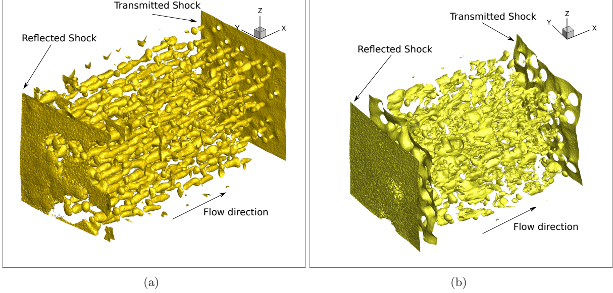
FIG. 3: Iso-surface plot of non-dimensional velocity magnitude for M_s = 3 and for (a) \phi_1 = 2.5\% , and (b) \phi_1 = 20\% .
