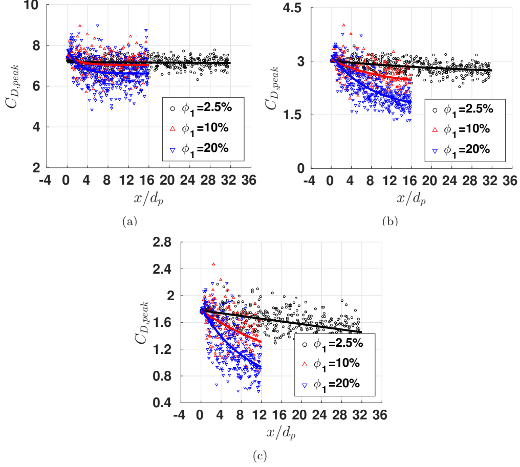
FIG. 12: Plot of peak drag coefficient, C_{D,peak} , along with the exponential curve fit for (a) M_s = 1.22 (b) M_s = 1.66 , (c) M_s = 3 ; \phi_1 = 2.5\% , \phi_1 = 10\% , and \phi_1 = 20\% .
