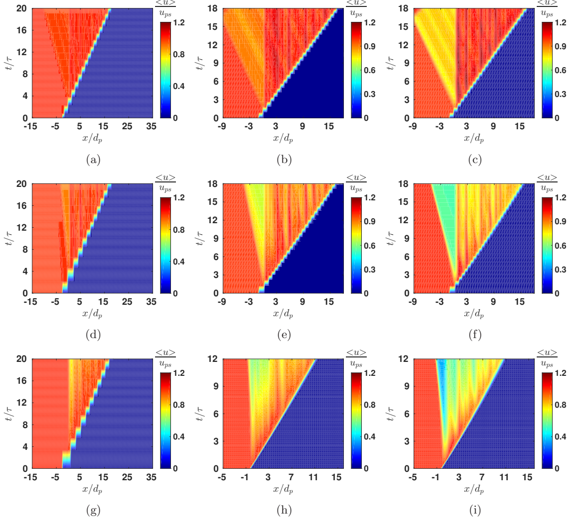
FIG. 7: x - t contour plot of the non-dimensional cross-sectional averaged streamwise velocity, \langle u \rangle / u_{ps} , for \phi_1 = 2.5, 10 , and 20\% and (a-c) M_s = 1.22 , (d-f) M_s = 1.66 , and (g-i) M_s = 3 , respectively.
