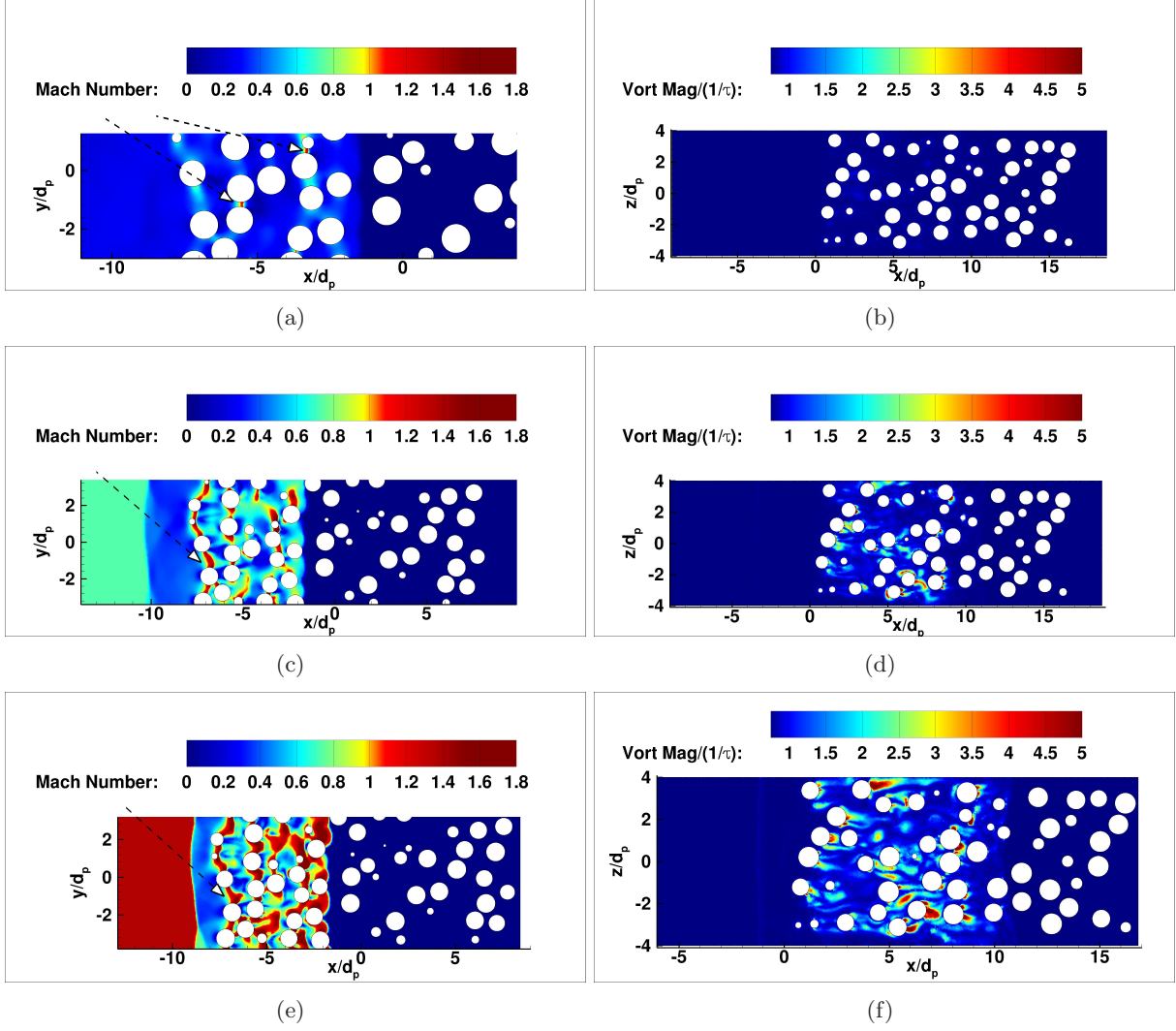
FIG. 5: Zoomed in contour plot of Mach number along the x-y plane at z=0 and t/\tau=7 for (a) M_s = 1.22 , (c) M_s = 1.66 , (e) M_s = 3 ; contour plot of non-dimensional vorticity magnitude along the x-z plane at y=0 and t/\tau=12 for (b) M_s = 1.22 , (d) M_s = 1.66 , and (f) M_s = 1.66 ; \phi_1 = 20\% .
