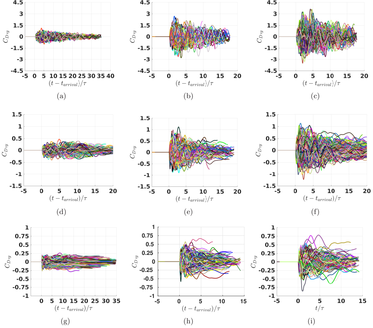
FIG. 14: Plot of non-dimensional y lift force, C_{D,y} , as a function of non-dimensional shifted time (t - t_{arrival})/\tau , for \phi_1 = 2.5, 10 , and 20\% and (a-c) M_s = 1.22 , (d-f) M_s = 1.66 , and (g-i) M_s = 3 , respectively.
