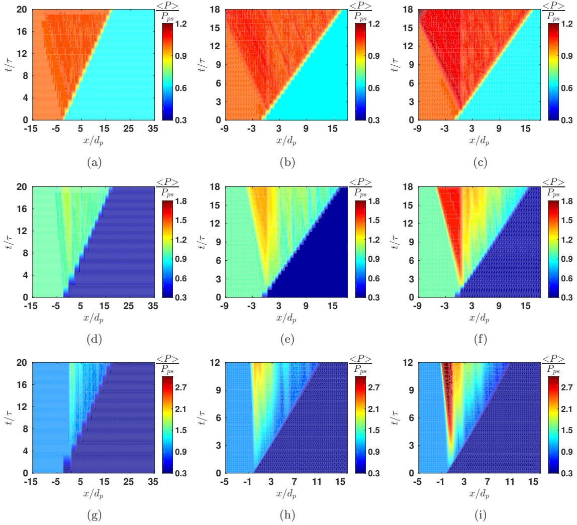
FIG. 6: x - t contour plot of the non-dimensional cross-sectional averaged pressure, \langle P \rangle / P_{ps} , for \phi_1 = 2.5, 10 , and 20\% and (a-c) M_s = 1.22 , (d-f) M_s = 1.66 , and (g-i) M_s = 3 , respectively.
