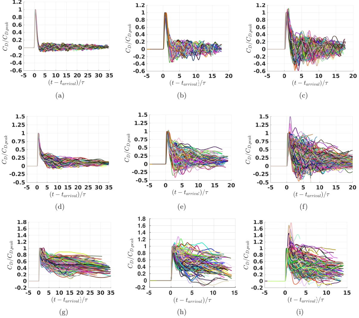
FIG. 10: Plot of normalized non-dimensional drag force, C_D , as a function of non-dimensional shifted time (t - t_{arrival})/\tau , for \phi_1 = 2.5, 10 , and 20\% and (a-c) M_s = 1.22 , (d-f) M_s = 1.66 , and (g-i) M_s = 3 , respectively.
