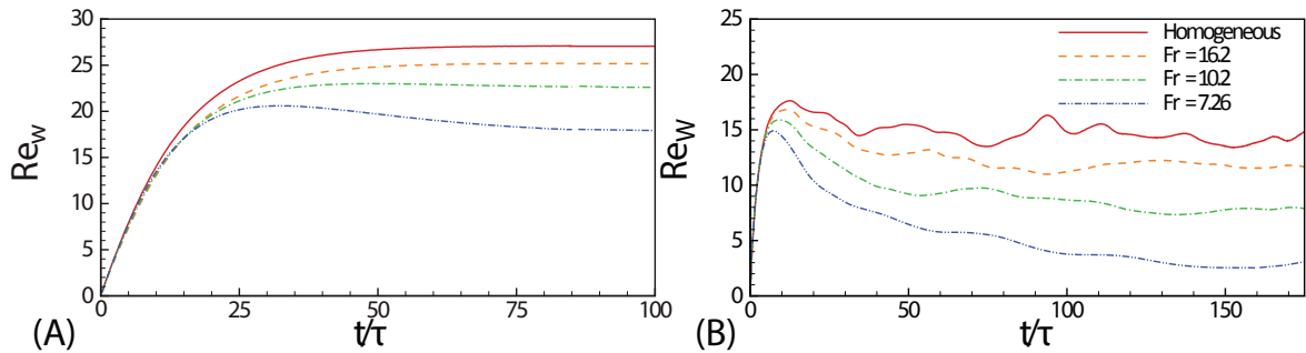
FIG. 4: The time evolution of the instantaneous rise Reynolds number of (a) a single drop, and (b) multiple drops in a stratified fluid at different Fr . (Reprinted from [34] with permission of Elsevier.)
