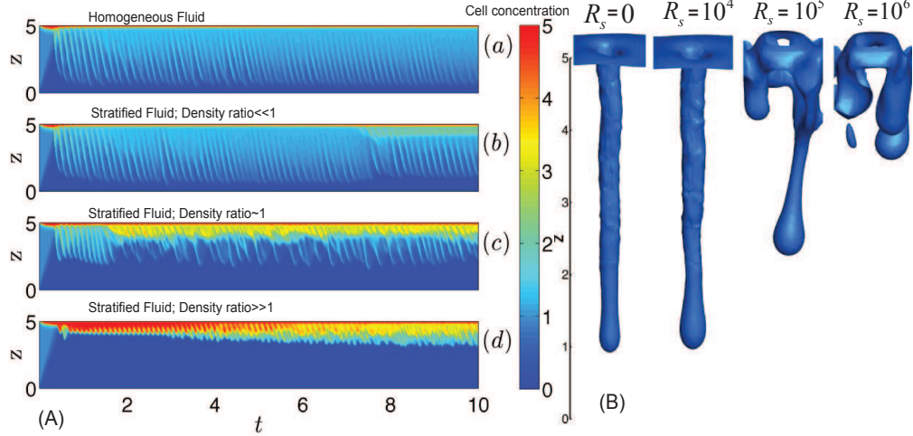
FIG. 7: (a) Space-time plots of the horizontal average of the cell concentration in a salt-stratified fluid. (b) The isosurface of cell concentration for different values of density stratification. Density stratification hinders the bioconvection plumes and leads to the accumulation of algal cells at pycnoclines. (Reprinted from [56] with the permission of Cambridge University Press.)
