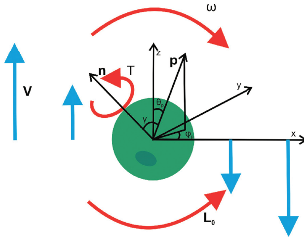
FIG. 8: A schematic of an algal cell like Heterosigma akashiwo , that utilizes two flagella – directed along the unit vectors \mathbf{p} and \mathbf{n} – for swimming. (Reprinted from [73] with the permission of AIP.)
