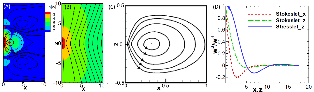
FIG. 1: Stratification dramatically alters flow fields of point force singularities. A vertical point force is shown (a) in a stratified fluid, (b) in a homogeneous fluid and (c) between two horizontal walls. Black lines are streamlines, colors indicate the magnitude of vertical velocity, w . (d) The results show that stratification induces a sharper decay of fluid velocity, w^S , with distance from the disturbance compared to the homogeneous fluid, for both a Stokeslet (red, green) and a stresslet (blue). (Reprinted from [15] with the permission of APS Publishing.)
