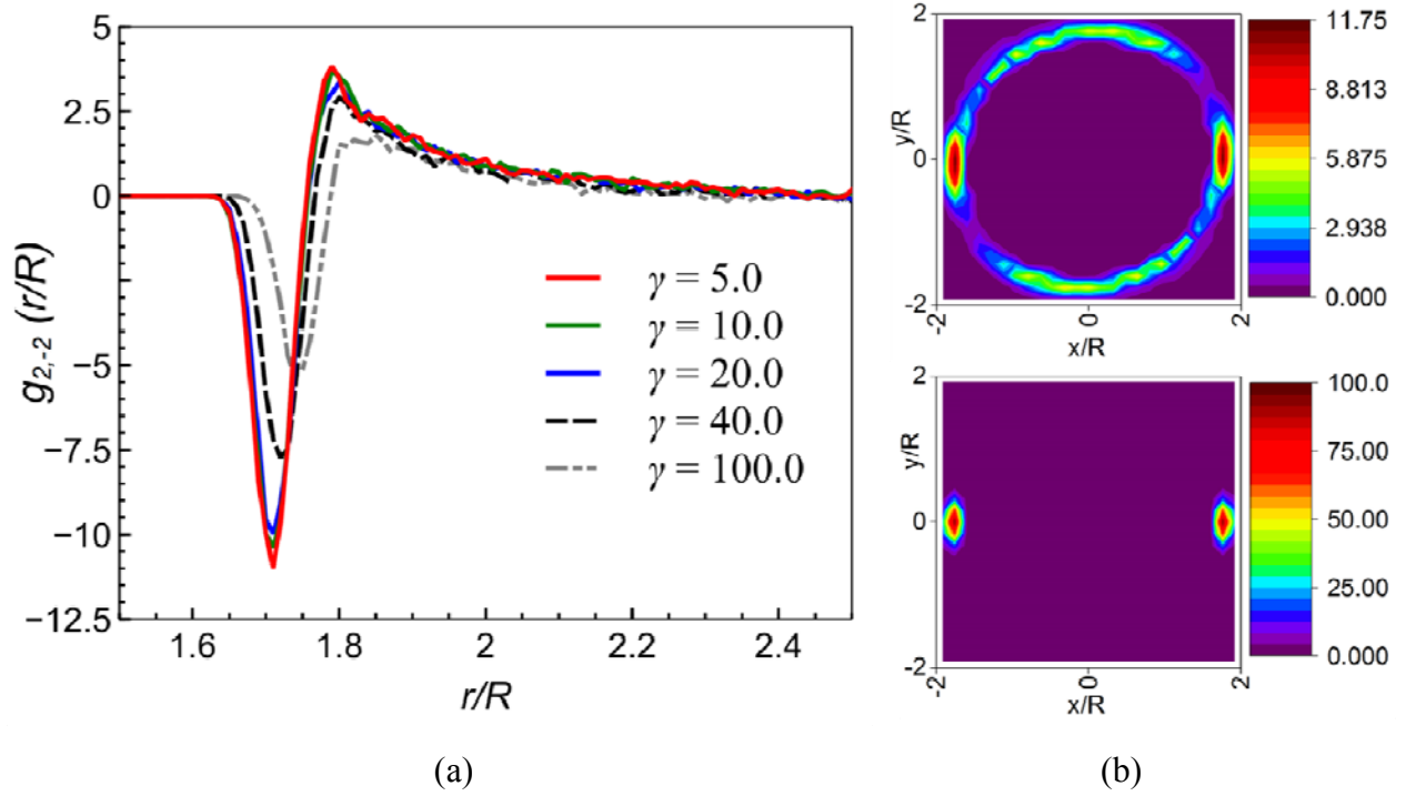
FIG. 7. (a) g_{2,-2}(r/R) as a function of the reduced distance for a suspension with \delta = 0.1 , \phi = 0.9 . (b) Two-dimensional pair distribution function at \gamma = 5 (top) and \gamma = 100 (bottom) obtained at z = 0 . The applied shear rate is \tilde{\gamma} = 10^{-4} .
