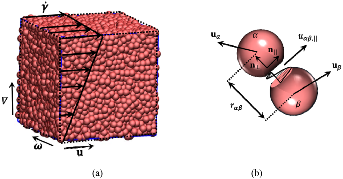
FIG. 1. (a) Configuration of a suspension with a volume fraction of 0.9 and polydispersity index of \delta = 0.1 that is in shear flow with an applied shear rate of \dot{\gamma} . The flow ( \mathbf{u} ), gradient ( \nabla ), and vorticity ( \boldsymbol{\omega} ) directions are shown in the figure. (b) Schematic showing pair-wise interaction between particles \alpha and \beta .
