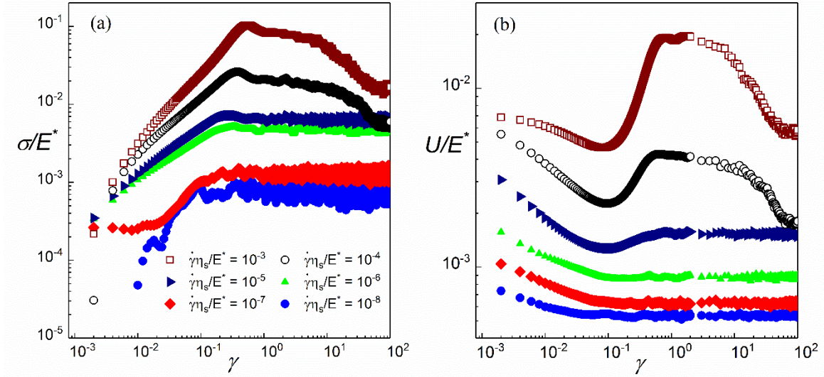
FIG. 3. (a) Shear stress and (b) elastic energy as a function of strain at different shear rates for a suspension with \delta = 0.1 and \phi = 0.8 . The symbols in Fig. 3b are at the same shear rate as Fig. 3a.
