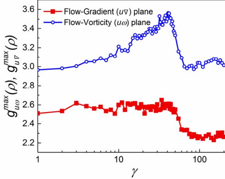
FIG. 11. The magnitude of the pair distribution functions at the first peak for a system with a volume fraction of 0.9 and polydispersity of 0.1. The applied shear rate is \tilde{\gamma} = 10^{-4} .
