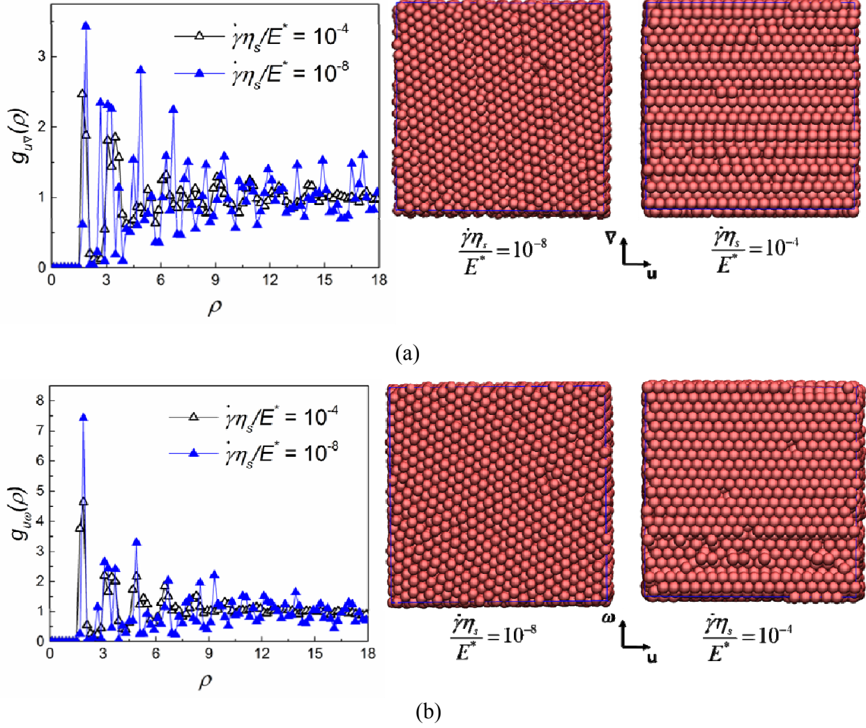
FIG. 5. (a) Flow-gradient and (b) flow-vorticity pair distribution functions of monodisperse suspension \phi=0.9 as a function of the two-dimensional distance ( \rho ) at different shear rates.
