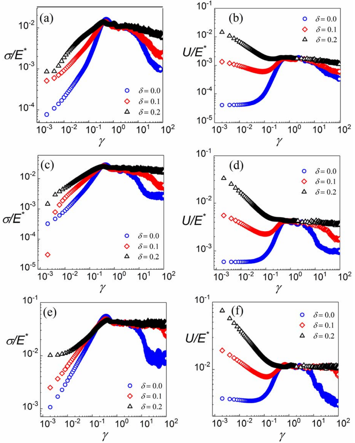
FIG. 2. Shear stress (left panel) and elastic energy (right panel) as a function of strain for different values of the polydispersity index and (a)(b) \phi = 0.7 , (c)(d) \phi = 0.8 , and (e)(f) \phi = 0.9 . The applied shear rate is \dot{\gamma} = 10^{-4} .
