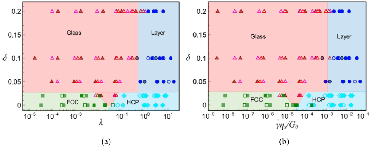
FIG. 10. State diagram of the soft particle glasses in shear flow as a function of (a) \lambda and (b) non-dimensional shear rate (determined using the low frequency modulus G_0 ). Following symbols are used to show the state of each suspension: \phi = 0.7 : layered structure (blue circle), glass (open red triangle), HCP (cyan square), and FCC (green square). \phi = 0.8 : layered structure (open blue circle), glass (open magenta triangle), HCP (open cyan square), and FCC (open green square). \phi = 0.9 : layered structure (half-filled blue circle), glass (half-filled brown triangle), HCP (half-filled cyan square), and FCC (half-filled green square).
