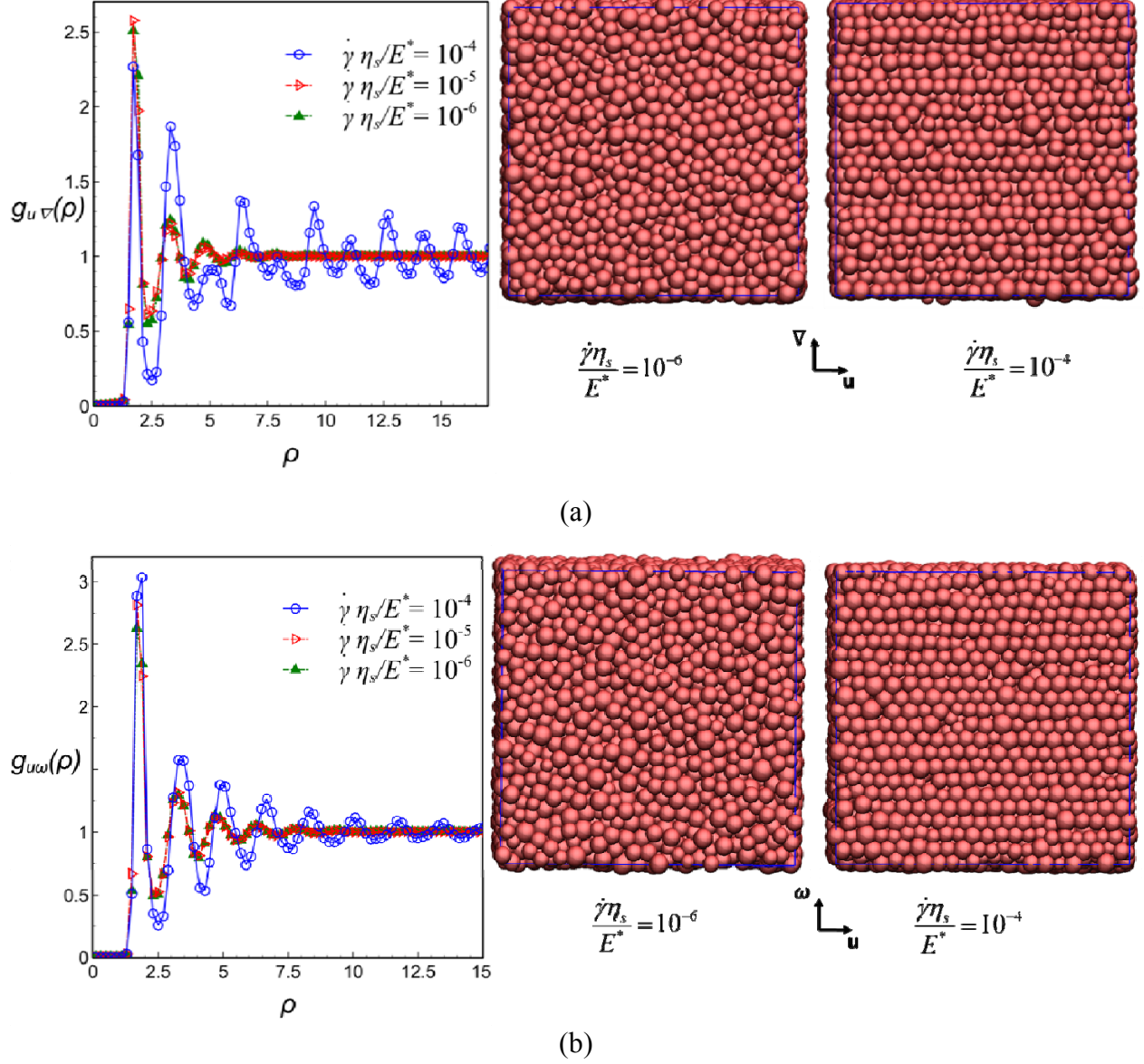
FIG. 8. (a) Effect of shear rate on the pair distribution function in the flow-gradient plane (left panel) and flow-gradient view of the end configuration of simulation box under different shear rates (right panel). (b) Effect of shear rate on the pair distribution function in the flow-vorticity plane (left panel) and flow-vorticity view of the end configuration of simulation box under different shear rates (right panel). Results are shown for the suspension with a polydispersity of 0.1 and volume fraction of 0.9.
