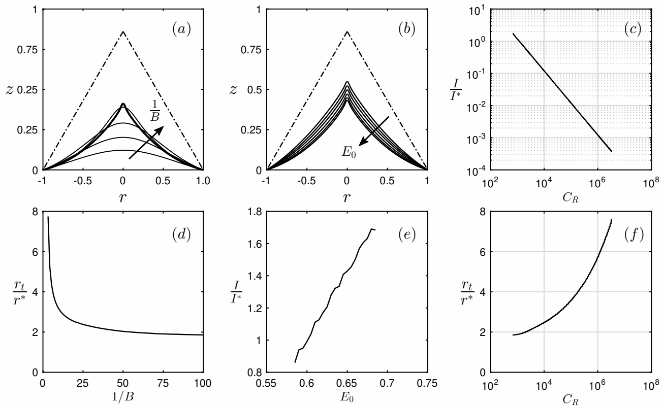
FIG. 6. Select parametric characteristics in the high field regime. Effects of the meniscus size (a,d), electric field (b,e), and impedance (c,f) are represented. (a) Meniscus shapes for E_0 = 0.7 and C_R = 10^3 . The meniscus size 1/B = 3.19, 4.26, 6.38, 17.0, 100 , increasing in the direction of increasing elongation. A classical Taylor cone (dashed) provides spatial reference. (b) Meniscus shapes for 1/B = 106 and C_R = 10^3 . The electric field E_0 = 0.585, 0.605, 0.625, 0.645, 0.665, 0.685 , increasing in the direction of decreasing elongation. A classical Taylor cone (dashed) provides spatial reference. (c) Electrical current for E_0 = 0.62 and 1/B = 106 over a range of impedance. (d) Radius of curvature at the meniscus tip for E_0 = 0.7 and C_R = 10^3 over a range of B . (e) Electrical current for 1/B = 106 and C_R = 10^3 over a range of field. (f) Radius of curvature at the meniscus tip for E_0 = 0.62 and 1/B = 106 over a range of impedance.
