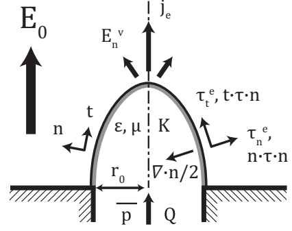
FIG. 2. Modeling configuration for an evaporating ionic liquid meniscus. An axisymmetric meniscus is attached to a conductive plate under vacuo with a contact radius r_0 (arbitrary contact angle) and stressed by an applied electric field E_0 that is asymptotically uniform at distances much greater than r_0 from the plate. Fresh liquid enters the meniscus during steady evaporation at a pressure \bar{p} , by a reservoir that is charged to a prescribed pressure p_r and a feeding line with characteristic impedance R_h .
