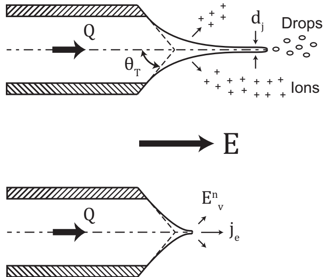
FIG. 1. Evolution of a cone-jet as the flow rate is reduced. Top: At high flow rates Q the meniscus resembles a classical Taylor cone (angle \theta_T \approx 49.2^\circ ) and exhibits a characteristic protuberance at the tip. The tip supplies a train of electro sprayed droplets that propagate under the influence of the external field E . It may eventually shed ions and other charges of low solvation as its diameter d_j decreases in response to waning flow. Bottom: Under certain conditions, very low flow rates lead to complete extinction of the jet, such that only ions emanate from a sharp tip through electrically-induced evaporation.
