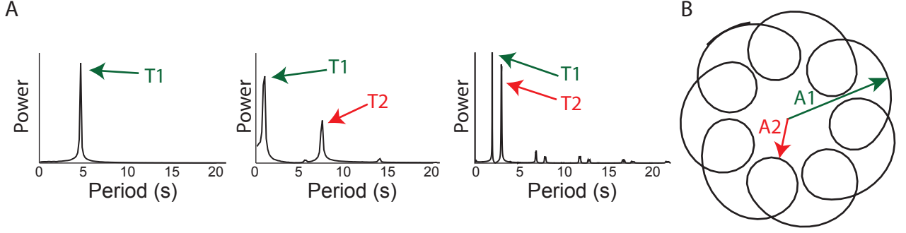
FIG. 2. A: Power spectrum of the x-component of the tip trajectory for the different electrophysiological models and parameter sets used in the main text. The spectra have either one or two peaks, corresponding to the frequencies \omega_1 = 2\pi/T_1 and \omega_2 = 2\pi/T_2 (left panel: FK Set I, middle panel: FK Set II, right panel: KKT). B: The spiral tip trajectory for set II. The maximum and minimum value of the spatial extent of the tip trajectory are denoted by A_1 and A_2 , respectively.
