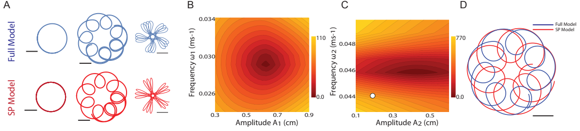
FIG. 4. A: Comparison between the full models (FK Set I right panel, FK Set II middle panel, and KKT right panel) and SP model for homogeneous media. Scale bars are 0.5cm. B, C: Cumulative error (measured in cm, and plotted using a color scheme) in the tip trajectory from the SP model for Set I (B) and II (C) as compared to the trajectory of the full model. The error was computed for every ms and for an entire rotation of the full model. D: Example of a trajectory of the SP model for the non-optimal parameters corresponding to the white symbol in C ( A_1 = 1.075 cm, A_2 = 0.2 cm, \omega_1 = 0.0058 ms -1 , and \omega_2 = 0.0439 ms -1 ).
