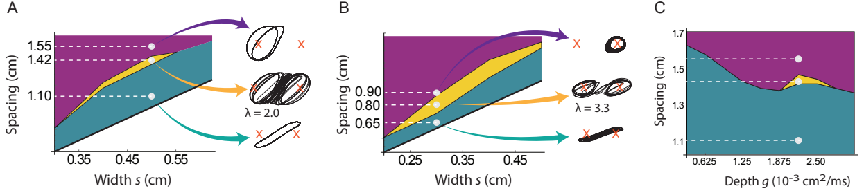
FIG. 6. A, B: Phase diagrams of tip trajectories for set I (A) and set II (B) in the SP model, with tip trajectories and Lyapunov exponents. See also Fig. 1. C: Phase diagram for Set I, illustrating the effect of different well depths g . The circles correspond to the parameter values of the circles in (A).
