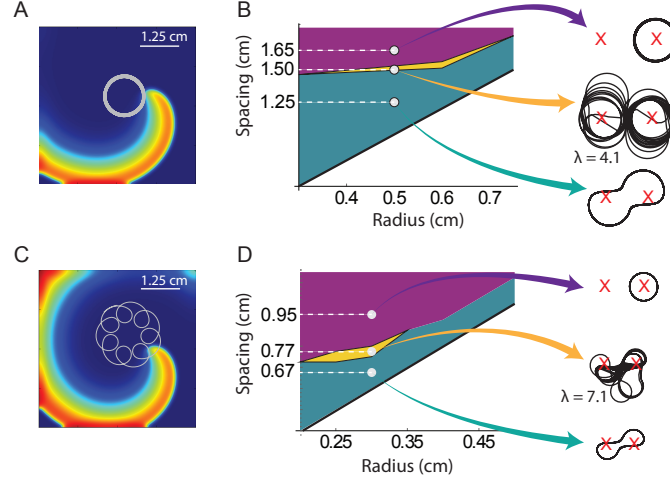
FIG. 1. A, C: Snapshot of a counter-clockwise rotating spiral wave for two different parameter sets of the FK model (voltage color-coded ranging from high (red) to low (blue) values, tip trajectory shown in white, A: Set I, C: Set II). B, D: Phase diagrams in the spacing-size space for the FK model. In this, and all other figures, blue area indicates regular trajectories that wrap around both heterogeneities, purple region represents tip trajectories that circle either one of the heterogeneities, and yellow region corresponds to chaotic trajectories. Displayed spiral tip trajectories correspond to the white dots in the phase diagram. Red X's mark the locations of the circular regions with decreased excitability. Lyapunov exponents ( \lambda ) for the chaotic trajectories are given in units of bits/second (B: Set I, D: Set II).
