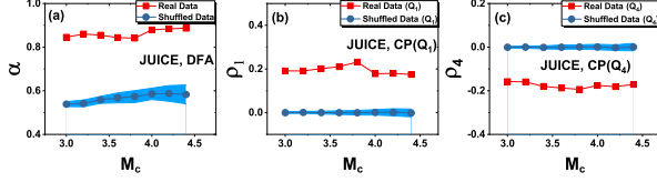
Figure 8. The same as Fig. 6 on the Japan Unified high-resolution relocated Catalog for Earthquakes (JUICE).
