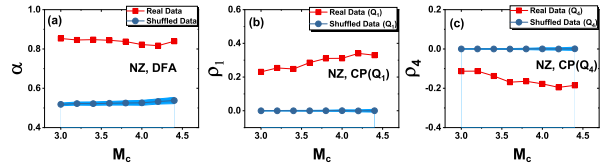
Figure 6. Results on the New Zealand (NZ) earthquake catalog. (a) DFA memory scaling exponent \alpha as a function of magnitude threshold M_c . (b) and (c) CP memory coefficient \rho_1 and \rho_4 as a function of magnitude threshold M_c . The blue lines in the bottom of each subplot indicate the DFA scaling exponent \alpha and the CP memory measure \rho_1, \rho_4 for the control randomly shuffled records, averaged over 1000 realizations; the shaded region indicates the error bars (std).
