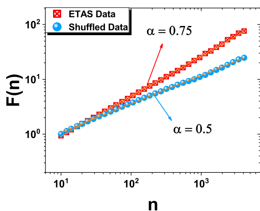
Figure 13. DFA of the interoccurrence times from the ETAS model, with parameters A = 6.26 , \mu = 0.2 , p = 1.1 , \alpha_M = 1.5 and c = 0.007 . The solid line is the best fitting line with slope \alpha = 0.75 , R-square > 0.99 . For comparison, the shuffled data with with slope \alpha = 0.5 , indicating no memory, are presented.
