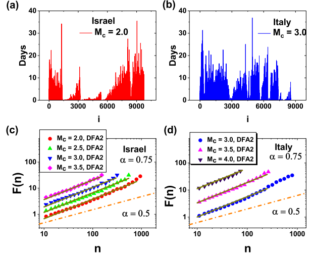
Figure 1. Interoccurrence time series between earthquake events from the Israeli (a) and Italian (b) catalogs using magnitude threshold M_c . DFA of the interoccurrence times from the (c) Israeli and (d) Italian catalogs with different M_c values. The solid lines are the best fit lines with slope \alpha \approx 0.75 ; the R-square is larger than 0.99. For comparison we also include a dashed-dotted line that indicates no memory ( \alpha = 0.5 ).
