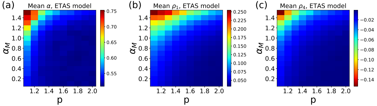
Figure 11. The mean values of the (a) DFA scaling exponent \alpha , (b) CP coefficient \rho_1 for short recurrence times Q_1 , and (c) CP coefficient \rho_4 for long recurrence times Q_4 as a function of ETAS model parameters, p and \alpha_M . The other ETAS parameters used are A = 6.26 , \mu = 0.2 and c = 0.007 , for the Italian catalog, following [31].
