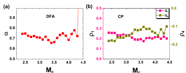
Figure 15. (a) DFA memory scaling exponent \alpha as a function of magnitude threshold M_c ; (b) CP memory coefficient \rho_1 and \rho_4 as a function of magnitude threshold M_c for ETAS model, with parameters A = 6.26 , \mu = 0.2 , p = 1.1 , \alpha_M = 1.5 and c = 0.007 .
