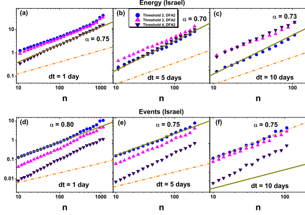
Figure 2. DFA of (a, b and c) the released energy time series, (d, e and f) the number of events time series, within a dt time period for Israeli catalog. The solid lines are the best fitting lines with slope \alpha where R-square > 0.99 . For comparison, the dashed-dotted line with slope \alpha = 0.5 , indicating no memory, is presented.
