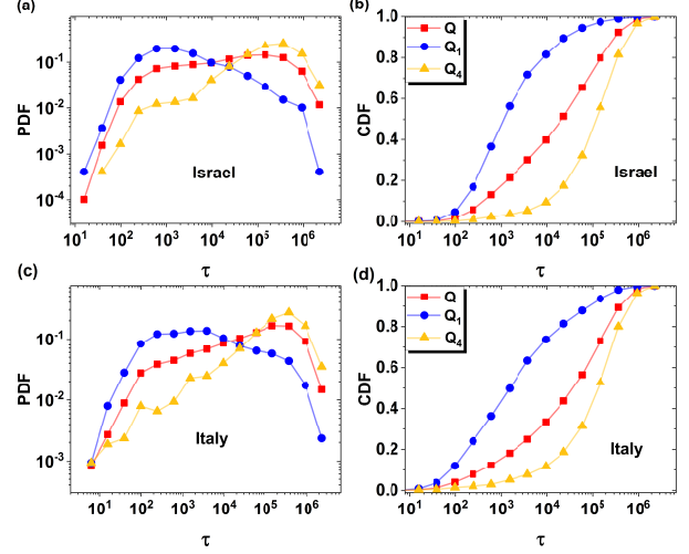
Figure 5. (a,c) Conditional PDF and (b,d) CDF of the recurrence times \tau for the (a,b) Israeli catalog above the threshold M_c = 2.0 and for the (c,d) Italian catalog above the threshold M_c = 3.0 .
