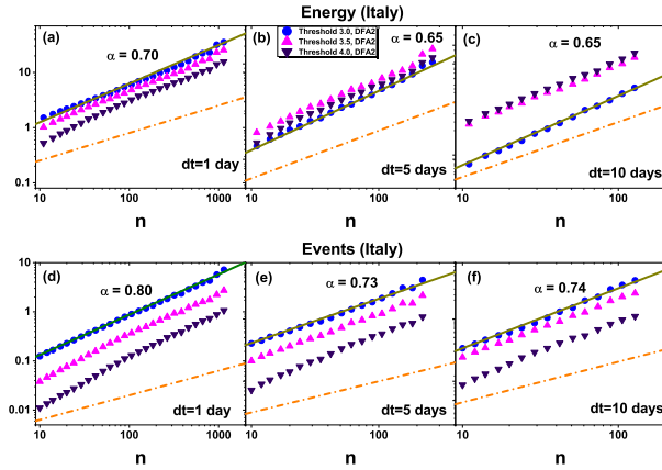
Figure 3. DFA of (a, b and c) the released energy time series, (d, e and f) the number of events time series, within a dt time period for Italian catalog. The solid lines are the best fitting lines with slope \alpha where R-square > 0.99 . For comparison, the dashed-dotted line with slope \alpha = 0.5 , indicating no memory, is presented.
