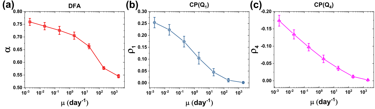
Figure 10. Memory measures \alpha , \rho_1 and \rho_4 as a function of ETAS parameter \mu . (a) DFA scaling exponent \alpha , (b) CP coefficient \rho_1 for short recurrence times Q_1 , (c) CP coefficient \rho_4 for long recurrence times Q_4 . The other ETAS parameters used are A = 6.26 , \alpha_M = 1.4 , p = 1.13 , c = 0.007 , and M_c = 3.0 for the Italian catalog, following [31]. The error bars (std) are based on 100 independent simulation realizations.
