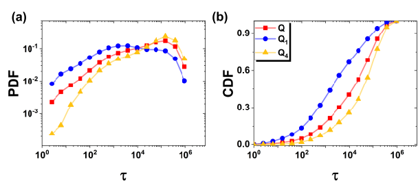
Figure 14. Conditional (a) PDF and (b) CDF of the recurrence times \tau for the ETAS model, with parameters A = 6.26 , \mu = 0.2 , p = 1.1 , \alpha_M = 1.5 and c = 0.007 .
