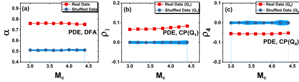
Figure 9. The same as Fig. 6 on the Preliminary Determination of Epicenters (PDE) catalog.
