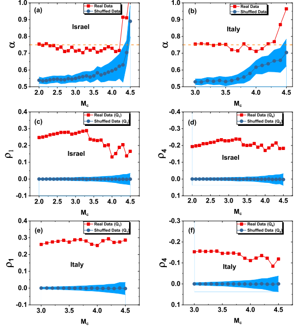
Figure 4. DFA scaling exponent \alpha as a function of the magnitude threshold M_c for the (a) Israeli and (b) Italian catalogs. CP memory coefficient \rho_1 and \rho_4 as a function of magnitude threshold M_c for the (c-d) Israeli and (e-f) Italian catalogs. The blue line (circles) in the bottom of each subplot depicts the mean results of randomly shuffled records, averaged over 1000 realizations; the shaded area indicates the error bars (std).
