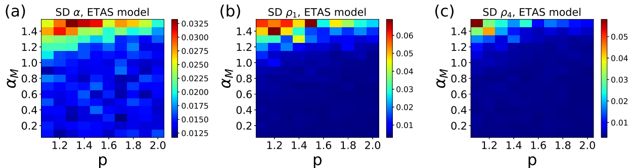
Figure 12. The standard deviation (SD) of (a) DFA scaling exponent \alpha , (b) CP coefficient \rho_1 for short recurrence times Q_1 , (c) CP coefficient \rho_4 for long recurrence times Q_4 . The other ETAS parameters used are A = 6.26 , \mu = 0.2 and c = 0.007 .
