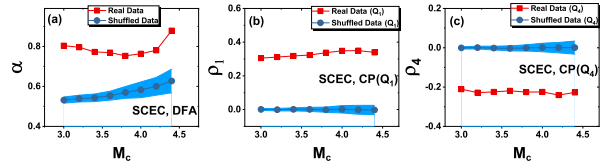
Figure 7. The same as Fig. 6 on the Southern California Earthquake Center (SCEC) earthquake catalog.
