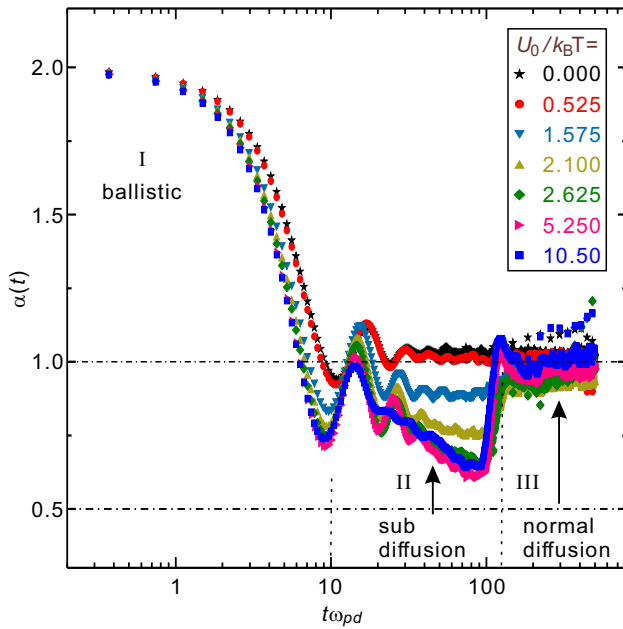
FIG. 7: (Color online) For the motion in the y direction, the obtained exponent \alpha(t) in the relation MSD = 4Dt^{\alpha(t)} for different depths of 1DPS at different times. Here, the exponent \alpha(t) in the y direction are calculated using the data from Fig. 6(c). The diffusion of 2DDP motion in the y direction can be divided into three processes, due to the 1DPS. Initially, the exponent decays from 2, due to the ballistic motion of dust particles, since they are still inside the cages formed by neighboring dust particles. At the intermediate time scale, the exponent of diffusion is between 0.5 and 1, corresponding to the sub-diffusion. This sub-diffusion feature is obvious, even when the depth of the 1DPS is not so large, such as U_0/k_B T \geq 1.575 . For the long time scale, the diffusion all changes to normal diffusion ( \alpha = 1.0 ) for different depths of 1DPS.
