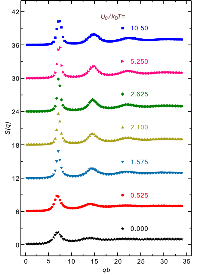
FIG. 4: (Color online) The averaged structure factor S(q) in the y direction, along the potential wells of 1DPS, for U_0/k_B T = 10.5 (squares), 5.25 (right triangles), 2.625 (diamonds), 2.1 (up triangles), 1.575 (down triangles), 0.525 (circles), and 0 (stars). We find the sharpest peaks for intermediate values of U_0/k_B T ranging from 2.1 to 5.25 , where the particles develop the strongest 1D ordering along the substrate troughs.
