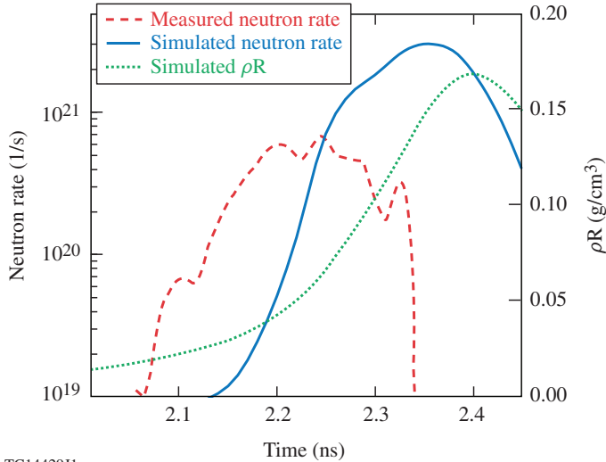
FIG. 5: (color online). Comparison of measured neutron rate, LILAC predicted neutron rate, and predicted evolution.
