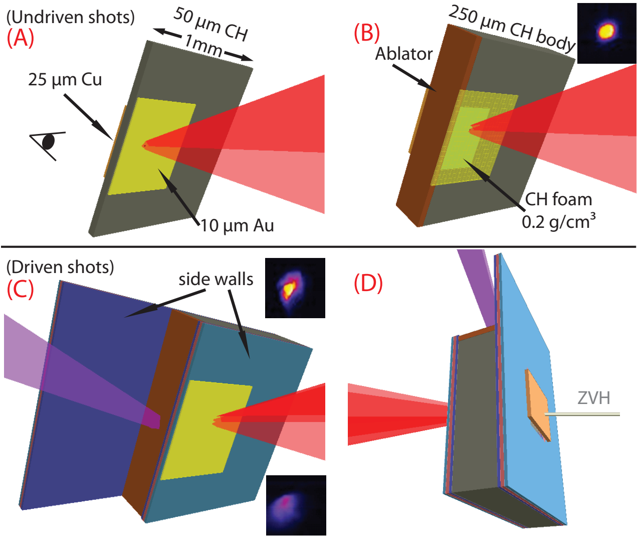
FIG. 1. (color online) Fast electrons from short pulse laser (red) interaction with a Au foil transported through three different CH layers: solid foil (A), foam (B), and foam heated to plasma by a 1.2 kJ beam (purple in C and D). The Au foil is shown partially transparent in (B) to reveal the foam. A Cu foil was behind the transport layers. (D) shows the perspective of the Spherical Crystal Imager and also indicates the line of sight of the Zn Von Hamos spectrometer. Pinhole camera images of the interaction are shown inset.
