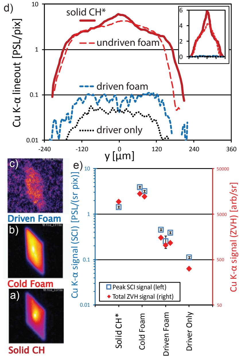
FIG. 2. (color online) Spherical Crystal Imager images of the Cu K \alpha emission (a-c, each normalized individually). Filter-corrected lineouts are plotted (d) and the signals from the SCI and ZVH are analyzed (e). [*The Solid CH data have been scaled by laser power.]
