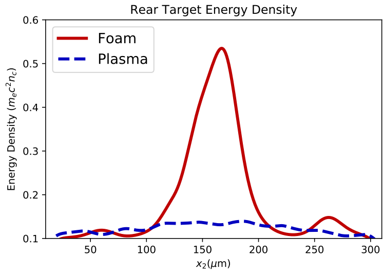
FIG. 4. (color online) Total energy density in the electrons in the rear 20- \mu\text{m} of the simulation target averaged over 6.3ps, for both plasma and foam cases.
