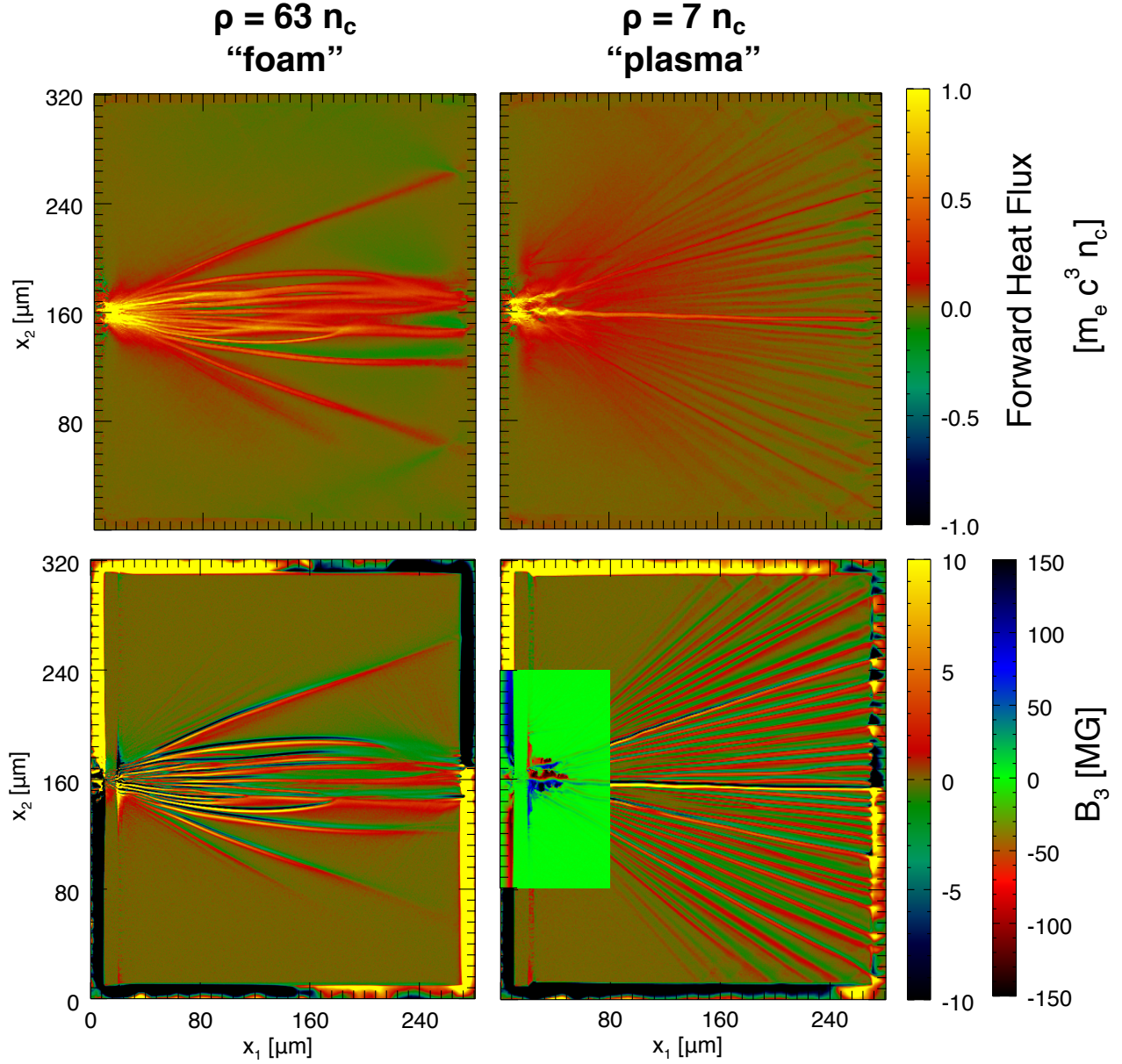
FIG. 3. (color online) Left column: Higher density “foam” case; right column: lower density “plasma” case. Top row: forward heat flux at t=6.3 ps. Bottom row: magnetic field at t=6.3 ps. In the plasma case the strong field at the Au/CH interface is shown with enhanced color scale.
