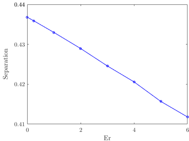
FIG. 11: Particle separation in dimensionless units as a function of Ericksen number. The decrease in separation as Er increases implies the hydrodynamic electrokinetic force is attractive.
