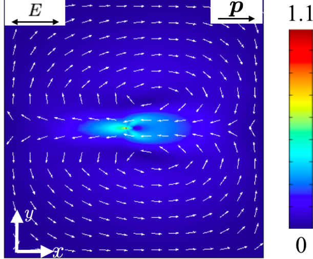
FIG. 6: Numerical velocity field for a (-1,+1) point defect pair, averaged over a period of the applied electric field, plotted in dimensionless units. Note the appearance of only two vortices here in contrast to the six vortices in Fig. 4.
