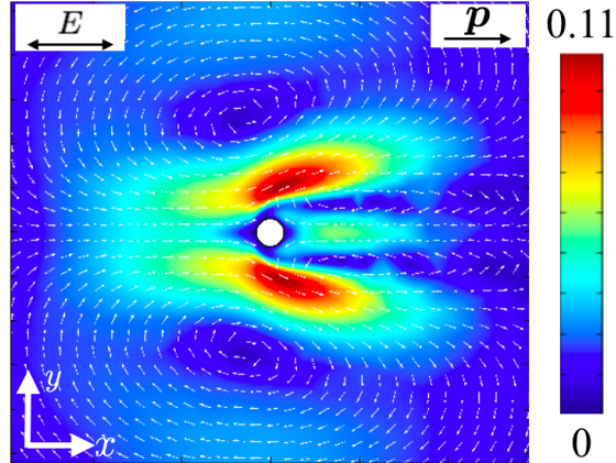
FIG. 8: Two dimensional average flow field induced by the director field, Eq. (28), at z = 0 , plotted in dimensionless units.
