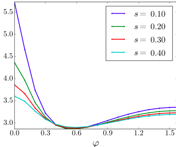
FIG. 12: Elastic energy (dimensionless units) for a system of two circular particles with tangential anchoring at various surface to surface separations s , and relative orientations \varphi (rad).
