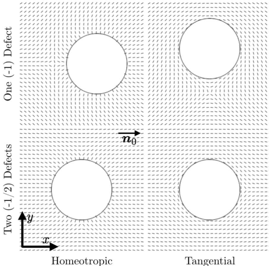
FIG. 2: Possible director fields around a disc in a two-dimensional domain, with far-field director orientation \mathbf{n}_0 = \hat{\mathbf{x}} . For both homeotropic and tangential anchoring, a suspended disc has topological charge (+1), requiring either one (-1) defect or two (-1/2) defects in the bulk.
