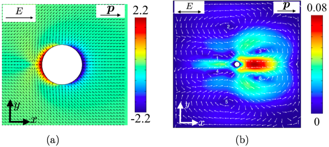
FIG. 4: Subset of the computational domain showing the numerical charge density at t = 2\pi (a), and the time averaged velocity (b) of the electrokinetic flow around a two dimensional particle with electric field parallel to elastic dipole, plotted in dimensionless units. The flow field comprises six vortices as shown by the labels in the figure. The electrokinetic force on the particle, computed using Eq. (18), is found to point opposite the elastic dipole \mathbf{p} .
