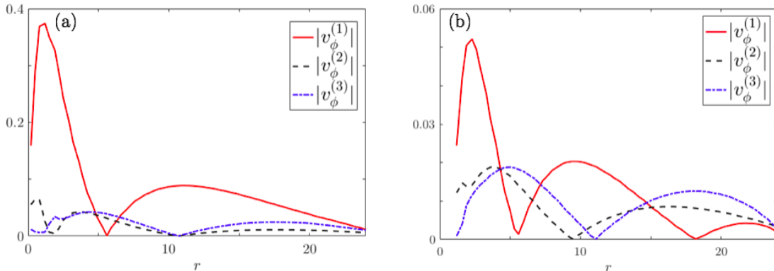
FIG. 7: First three Fourier components of numerical angular velocity for a system with a (-1,+1) point defect set, (a), and a particle-defect pair, (b), averaged over a period of the field, plotted in dimensionless units as a function of r .
