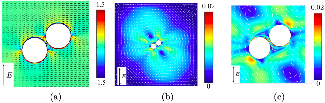
FIG. 13: (a) Instantaneous charge density in corresponding to two circular particles fixed at the separation and angle that minimize the elastic free energy. The oscillatory electric field point in the y direction. (b) Time averaged electrokinetic velocity, which is shown magnified in (c) to highlight the appearance of boundary layer flows near particle surfaces. All values are in dimensionless units.
