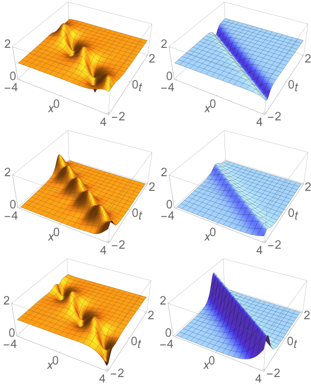
FIG. 5. Amplitudes of a one-soliton solution of the spinor BEC model with NZBC with k_0 = 1 , discrete eigenvalue \zeta = 2ie^{-i\pi/6} and \gamma = 1 in class C. Left: the solution \Phi(x,t) with U_C defined in Eq. (A.5) and parameters \beta_1 = -\pi/2 , \beta_2 = \pi and n = 0 . From top to bottom: |\phi_1(x,t)| , |\phi_0(x,t)| and |\phi_{-1}(x,t)| . Right: the corresponding core soliton component Q(x,t) from Eq. (31), with |q_{1,1}(x,t)| = |q_{2,2}(x,t)| (top), |q_{1,2}(x,t)| (center) and |q_{2,1}(x,t)| (bottom).
