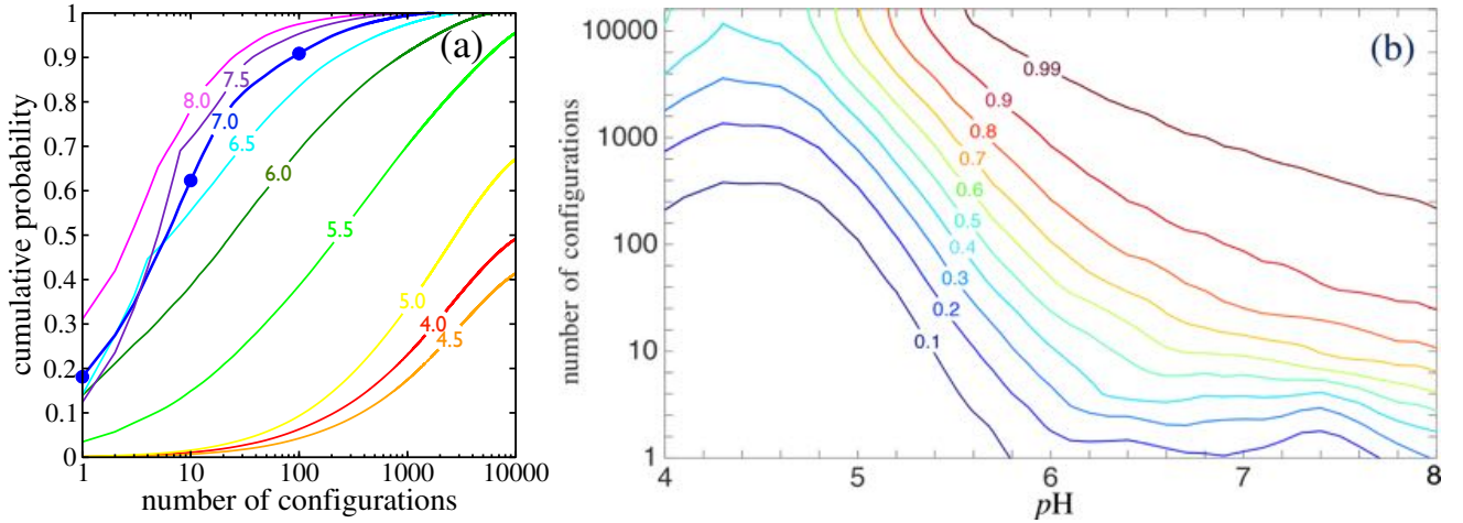
FIG. 13. (color online) (a): Cumulative probabilities of the most probable protonation patterns at a Debye length of 6.0 Å. For example, the dots on the pH 7.0 curve show that under these conditions, the top \gamma B occupancy pattern occurs nearly 20% of the time, one of the first 10 patterns will be present 60% of the time, and one of the top 100 patterns occurs 90% of the time. The pH 4.5 curve shows that one of the first 1,000 patterns will be present 20% of the time. (b): Contours of the cumulative probabilities displayed in the (pH, \log_{10}(\text{number of configurations})) -plane. For example, the 0.99 contour indicates that at pH \approx 6.8 , 1,000 configurations account for 99% of the probability.
