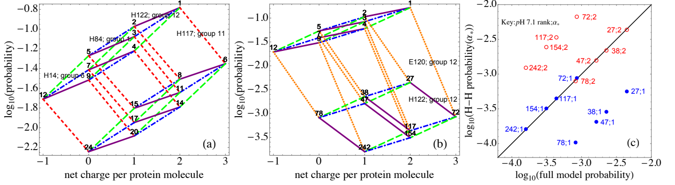
FIG. 7. (color online) In panel (a), because H117 is only weakly linked to other residues (see Fig. 3(c), group 11), when H117 switches charge (red, shorter dashes), the eight-vertex polygon representing the possible switches of H122 (purple, solid), H84 (blue, dash-dot), and H14 (green, longer dashes) undergoes translation with very little distortion (see text). In panel (b), because E120 and H122 interact strongly, when E120 changes from charge -1 to 0 the H122 switching segments markedly change slope, distorting the same polygon. Panel (c) further analyzes the changes in (b), by comparing the full model probabilities with those of a Henderson-Hasselbalch approach. Agreement would correspond to all points being on the solid diagonal line. Panel (c) illustrates that the E120 switch markedly alters some probabilities from Henderson-Hasselbalch values (see text).
