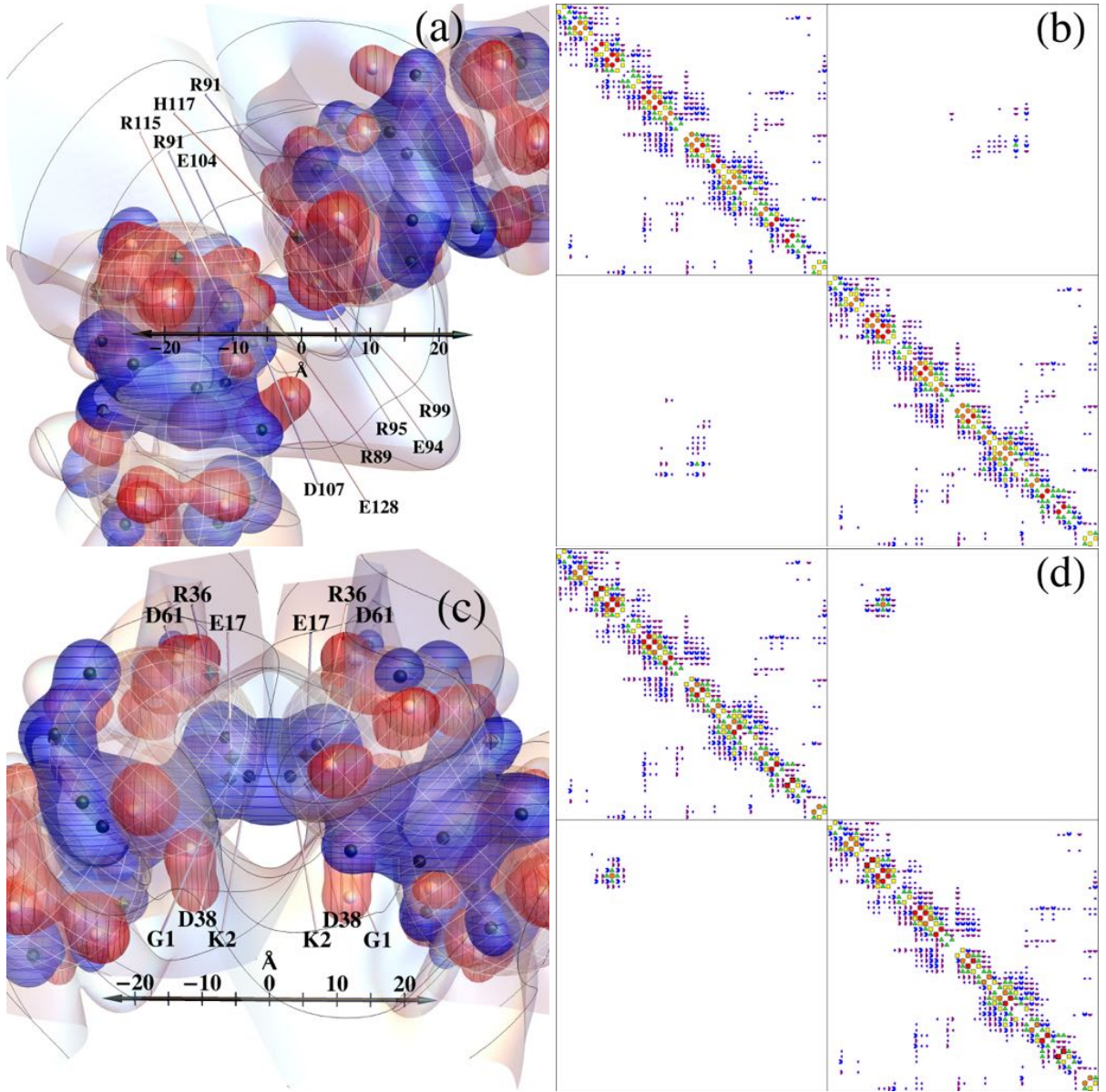
FIG. 19. (color online) Changing the relative orientations of two neighboring proteins alters the expanded, two protein work-of-charging matrix. The voltage contour surface designations in panels (a) and (c) are the same as in Fig. 1(a), except that the curves on the 0 volt contour surface are spaced by 12 Å from the calculation box center. The dielectric surfaces are outlined by white longitude and latitude curves. Panels (b) and (d) use the same color code as in Fig. 3. In panels (b) and (d), the upper left and lower right squares show the within-protein recalculated work-of-charging matrix entries, while the off-diagonal squares show the between-protein entries. In (a) and (c), different sets of residues are adjacent to one another, as indicated, producing differences in the corresponding work-of-charging matrices shown in (b) and (d), respectively. The order of residues is the same for each protein in (b) and (d), but differs from that in Fig. 3.
