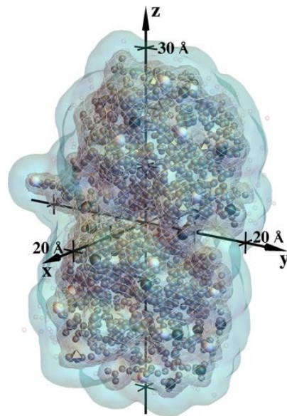
FIG. 2. (color online) Illustration of the dielectric and salt-exclusion zone model for bovine \gamma B-crystallin, based on PDB entry 1AMM [97], rotated and translated to the coordinate system used for numerical solution of Eq. (1). The dark gray netted surface is the boundary of the low dielectric region, and the light plain surface is the boundary of the salt-exclusion zone, described in the text. Larger black and white spheres and gray octahedra show titratable sites that are positive, negative, and neutral, respectively, for the most probable configuration at pH 7.0, modeled to occur about 20% of the time, see Fig. 13(a). Smaller dark gray spheres are locations of non-hydrogen atoms in the 1AMM structure, and smaller lighter spheres are positions of heteroatoms.
