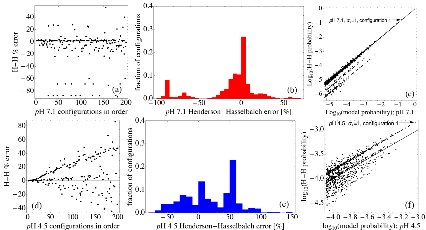
FIG. 9. (color online) (a): Percentage deviation of the Henderson-Hasselbalch probabilities of the top-ranked 200 configurations from those of the full model at pH 7.1. Panels (a), (b), and (c) all use \alpha_* = 1 for pH 7.1 to determine pK_{\text{eff},\alpha_*} values for use in calculating Henderson-Hasselbalch probabilities. (b): Histogram of the same deviations, for the top-ranked 1000 configurations from the Henderson-Hasselbalch probabilities. (c): Log-log comparison of the top-ranked 1000 configuration probabilities from the full model with the Henderson-Hasselbalch probabilities. Note the clustering along diagonal lines. (d): Similar percentage deviations of the top-ranked 200 configurations at pH 4.5. Panels (d), (e), and (f) all use \alpha_* = 1 for pH 4.5 to determine pK_{\text{eff},\alpha_*} values for use in calculating Henderson-Hasselbalch probabilities. (e): Histogram of the deviations at pH 4.5. (f): Log-log comparison of the top-ranked 1000 configuration probabilities; note the changed scales.
