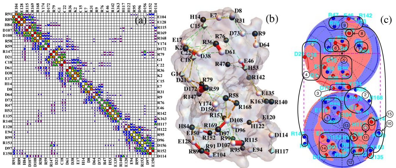
FIG. 3. (color online) (a) Approximate block-diagonal form of the dimensionless work-of-charging matrix W for interior dielectric coefficient 3 and Debye length 6.0\text{\AA} . W_{ij} magnitude categories: white < 0.05 \leq dark purple quarter circles < 0.1 \leq purple half circles < 0.2 \leq blue 3/4-circles < 0.4 \leq green triangles < 0.8 \leq yellow squares < 1.6 \leq orange pentagons < 3.2 \leq red circles. The matrix includes all 54 titratable residues used in the present model, which as noted in the text omits the tyrosine residues and four of the cysteine residues; the entire protein contains 174 residues. Designations for the 54 residues considered alternate between left and right (and top and bottom) margins. (b) Cylinders with radii proportional to W_{ij} mapped onto the PDB 1AMM structure of \gamma B-crystallin; W_{ij} magnitude categories: 0.4 \leq green cylinders with three gaps < 0.8 \leq yellow cylinders with two gaps < 1.6 \leq orange cylinders with one gap < 3.2 \leq red cylinders. (c): Lambert projections with potential and charges indicated as in Fig. 1(c). Groups of titratable sites participating in approximate blocks of W are circled in black and numbered in (c), and indicated by black squares in (a). Group numbering corresponds to the order of sites in W in Fig. 3(a), from top to bottom, and group numbers are those to which Figs. 7 and 8 refer. In (b) and (c) the protonation configuration is that modeled to be the most common one at pH 7.1.
