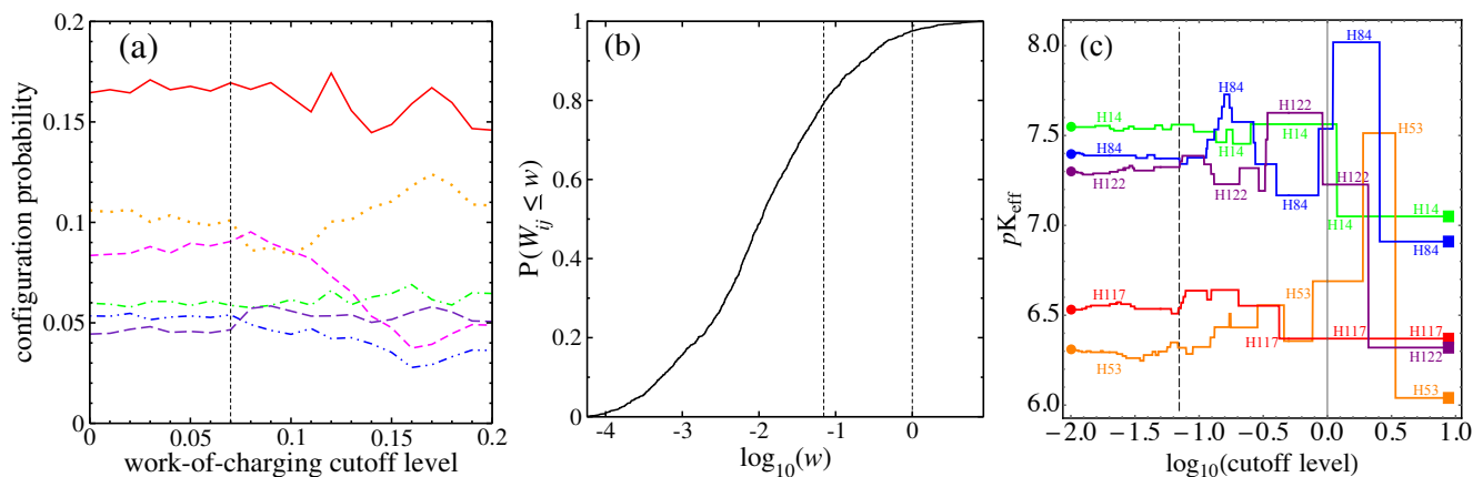
FIG. 10. (color online) (a): Dependence on dimensionless work-of-charging cutoff level of the six most common proton configurations at pH 7.1, Debye length 6.0\text{\AA} . At each cutoff level on the horizontal axis, all of the entries in W below the given level were set to zero, and the probabilities of the configurations were recalculated using Eq. (5). At this pH , the order of the configurations is stable up to a cutoff level of 0.07, which is shown by the vertical dashed line. (b): Cumulative distribution function of the work-of-charging matrix entries (see text). The left vertical line in (b) corresponds to the cutoff level of 0.07 indicated in (a). The right vertical line is at 1. (c) Changes in pK_{\text{eff},\alpha_*} values of the indicated histidine residues, whose protonation switches produce the top-ranked configurations shown in (a). Above a cutoff of 0.07, the H84 pK_{\text{eff},\alpha_*} value changes are the primary reasons for the configuration probability changes in (a); see text.
