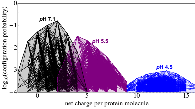
FIG. 12. (color online) \log_{10} P vs. net charge, with line segments indicating single-residue protonation switches, for protonation patterns that occur at pH 7.1 (black, the same as in Fig. 5), pH 5.5 (purple, dash-dot), and pH 4.5 (blue, dotted); see text.
