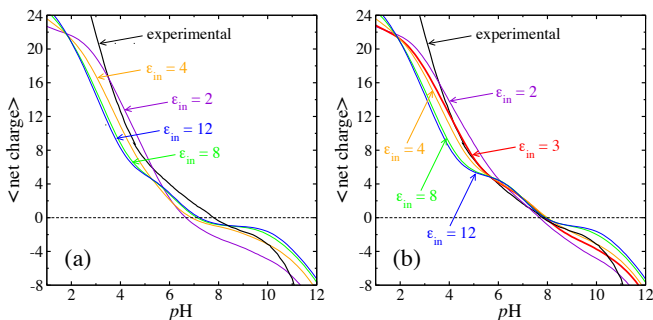
FIG. 4. (color online) Selection of interior dielectric coefficient and pK values through comparison of modeled titration curves with experiment. The experimental data [74] are shown by the labeled curve. The work-of-charging matrix W was calculated as described in the text, for different choices of \varepsilon_{in} . (a) Calculated titration curves when all pK_{int,\varepsilon_{in}} values were calculated according to the \mathbf{D}(\mathbf{r}) \cdot \mathbf{E}(\mathbf{r}) integral method described in Section IID, for the same \varepsilon_{in} values used for solution of Eq. 1 to yield the matrix W . (b) Calculated titration curves when all but the histidine pK_{int,\varepsilon_{in}} values were estimated with the integral method, as functions of \varepsilon_{in} , while PropKa 3.1 values were used for histidine (Table I) pK_{int} values; see text. In panel (b), the red (bold) \varepsilon_{in} = 3 curve is that of the model adopted for further study of the probability distributions.
