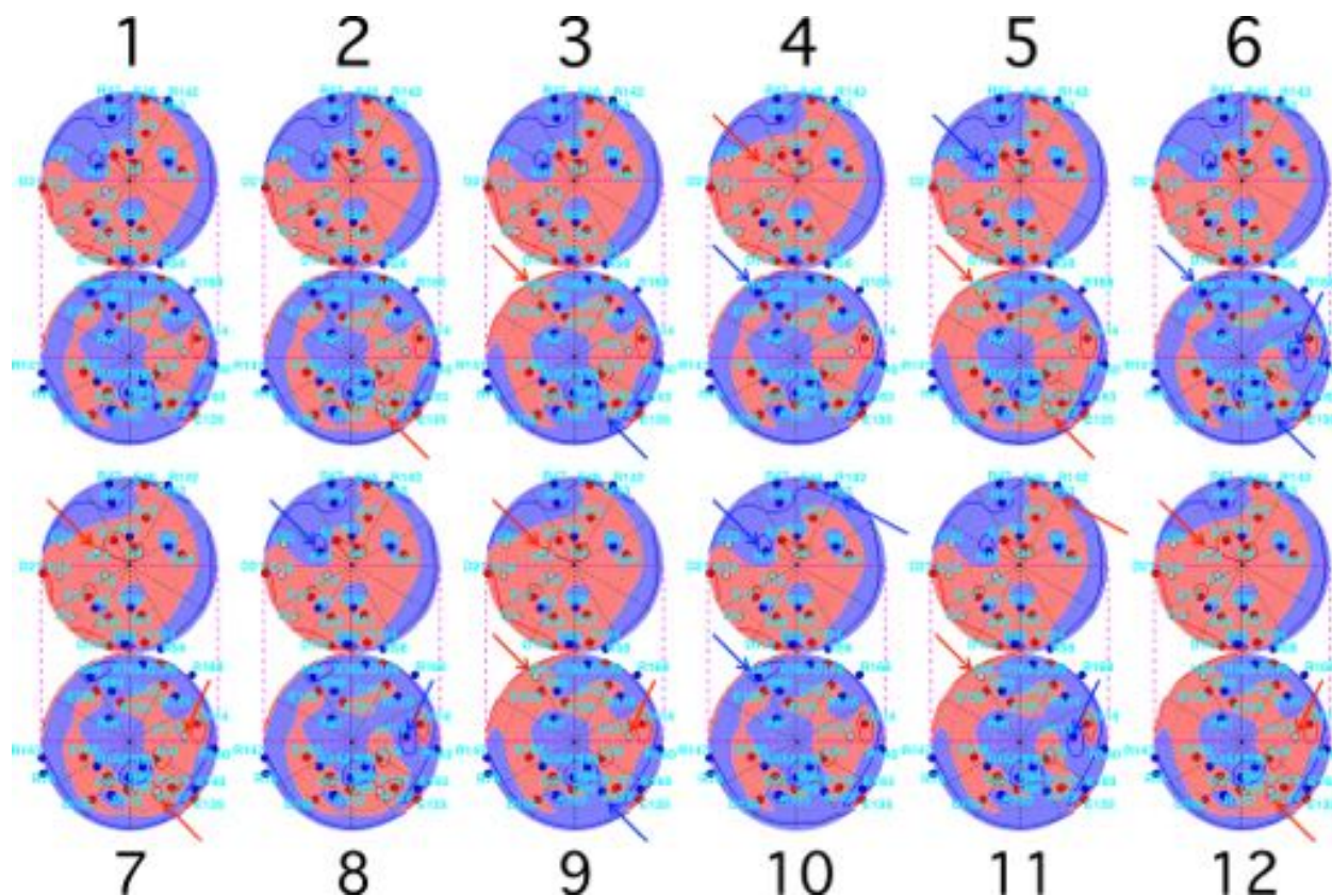
FIG. 6. (color online) Lambert projections, with potentials and charges indicated as in Fig. 1(c), for the 12 most probable configurations at pH=7.1 and Debye length 6\text{\AA} , in order of probability (see Table II). Residues that have gained or lost a proton, with respect to the more common configuration that is adjacent in order, are shown by blue (darker) and red (lighter) arrows, respectively. For many protonation switches, positive (blue, dark) and negative (red, lighter) voltage regions change connectivity.
