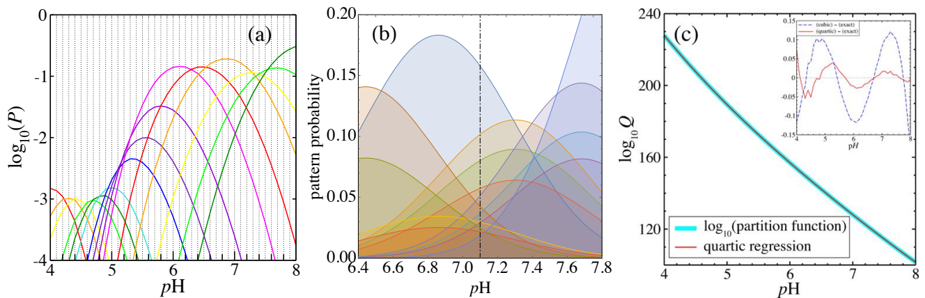
FIG. 14. (color online) (a) pH dependence of the probabilities of patterns that are each the top pattern in some interval of pH . (b) P_a vs. pH for the top 12 configurations at pH 7.1 have nearly Gaussian distributions with respect to pH . (c) \log_{10} Q from the present model, determined using Monte Carlo simulations (10 million samples per pH , in 0.1 pH steps). The inset shows the residuals to two of the fits, which for the quartic fit in this pH interval have a range of about 1 part in 4,000 of \log_{10} Q .
