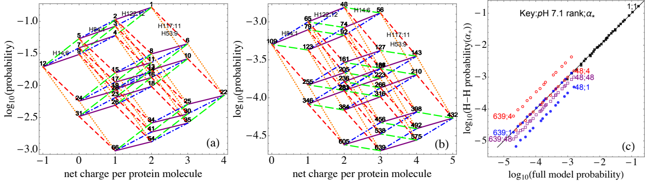
FIG. 8. (color online) (a): The most common 32-vertex polygon representing possible switches of all 5 histidine residues at pH 7.1; H53 switches (orange, dotted) are shown as well as the H122 (purple, solid), H84 (blue, dash-dot), and H14 (green, longer dashes) depicted in Fig. 7. (b): The 32-vertex polygon of histidine switches that occurs under the condition that E7, a neighbor of H14, has gained a proton to become neutral. The positively charged state of H14, which had been stabilized by a neighboring negative charge, is now less probable than its neutral state, and the green, long-dashed segments have negative slopes, while the others retain their slopes. Note the change in the vertical scale. (c): Comparison of probabilities from the full model and a Henderson-Hasselbalch approach for the topmost 32-vertex polygon in (a) (black squares), using \alpha_* = 1 , and the choices \alpha_* = 1 (blue solid circles), \alpha_* = 4 (red open circles), and \alpha_* = 48 (purple open squares) for the polygon in (b). The diagonal solid line is that of agreement between the two methods.
