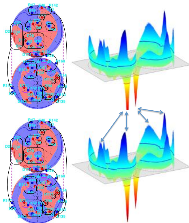
FIG. 18. (color online) Visualization of the sets of relative orientations that could give electrostatic attractions between neighboring \gamma -crystallins. Lambert projections, as in Fig. 3(c) and described there, of the electrostatic potential at about one-half Debye length from two copies of the most common pH 7.1 protonation configuration are shown at left. Voltages on the same surfaces are plotted vertically at right, above and below the Lambert projections, with positive up. While the arrows here simply join positive to negative peaks, non-peak locations can also attract, depending on twist angle.
