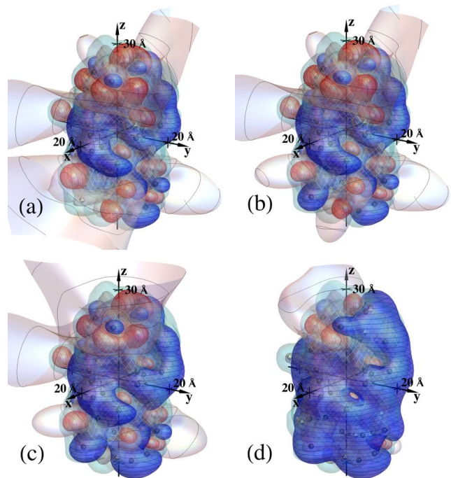
FIG. 11. (color online) Screened potential contours of \gamma B-crystallin, for the most common protonation patterns at pH=7.1 ((a), as in Fig. 1), 6.5 (b), 5.0 (c), and 4.5 (d). Debye length 6.0\text{\AA} ; contour values +k_B T/e volts (blue with horizontal curves), 0 volts (gray; curves as in Fig. 1(a)), and -k_B T/e volts (red with vertical curves); dielectric and electrolyte boundaries are designated as in Fig. 1(a). Note the changing balance between positive and negative voltage regions with pH , and an accompanying shrinkage of zero-voltage contours, most of which, at pH 4.5, extend to less than a Debye length from the protein.
