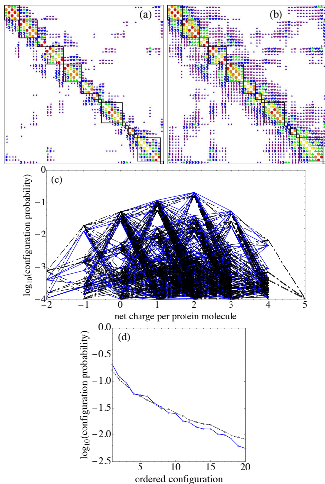
FIG. 16. (color online) Lowering ionic strength, corresponding to increasing the Debye length, \lambda_D , from 6 Å in (a) to 20 Å in (b) increases off-diagonal work-of-charging entries, and makes the top configurations more prominent while suppressing others, as shown in (c) and (d). In panels (a) and (b) W_{ij} magnitude codes are as in Fig. 3(a). For a 1:1 electrolyte in water at 298K, panels (a) and (b) correspond to ionic strengths of 257mM and 23.1mM, respectively. In going from (a) to (b), in all categories but the top (red circles), entries above 0.05 k_B T increase in number with increased \lambda_D . (c) \log_{10} P vs. net charge, as in Fig. 5. Black dot-dashed lines: \lambda_D = 6 Å, blue solid lines: \lambda_D = 20 Å. (d) \log_{10} P for the top 20 configurations; note the changed vertical scale. Black dashed line: \lambda_D = 6 Å, blue solid line: \lambda_D = 20 Å. The contrast between changes in top- and lower-ranked probabilities is shown by the crossing of the dashed and solid curves.
