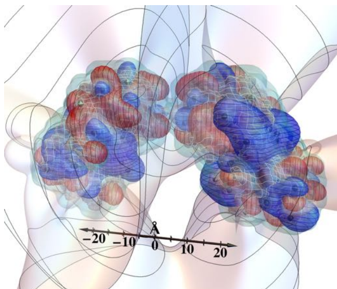
FIG. 17. (color online) Screened voltage contours around neighboring \gamma B-crystallin molecules, pH 7.1, Debye length 6 Å. The voltage contour surface designations are as in Fig. 1(a), except that the curves on the 0 volt contour surface are spaced by 12 Å from the calculation box center. Each molecule has the top-ranked protonation configuration.
