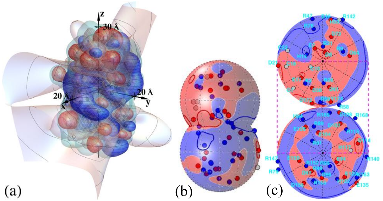
FIG. 1. (color online) (a) Screened potential contours produced by the charges of \gamma B-crystallin, for the most common protonation pattern occurring at pH=7.1 and Debye length 6.0\text{\AA} , corresponding to an ionic strength of 257\text{mM} for a 1:1 electrolyte in water at 298\text{K} : +k_B T/e volts (blue with horizontal curves), 0 volts (light) and -k_B T/e volts (red with vertical curves). Black spheres, gray octahedra, and white spheres show positive, neutral, and negative sites, respectively. Curves on the 0 volt contour are spaced by two Debye lengths from the center of the protein. The netted surface is the low-dielectric boundary, and the plain (light blue) surface just outside it is the electrolyte boundary; see Fig. 2. (b) To aid in visualization, auxiliary spheres of radius 18.5\text{\AA} were placed over top and bottom parts of the molecule, and the potential and charges are shown in blue (+) (dark gray and nearly black, respectively) or red (-) (potential light and charges dark gray). Neutral charges are lightest in (b). (c) A simultaneous view of voltages around the entire protein surface can be given with use of two Lambert azimuthal equal-area projections, one for each of the top and bottom spheres; projected locations of amino-acid residues of possibly charged sites are indicated. Grayscale description of (c) is like that in (b). The dashed rectangle in (c) shows the portion that is visible in (b). The top and bottom perimeter circles in (c) are both images of the crease between the auxiliary spheres in (b). Darker curves in (b) and (c) show +k_B T/e and -k_B T/e volt contours.
