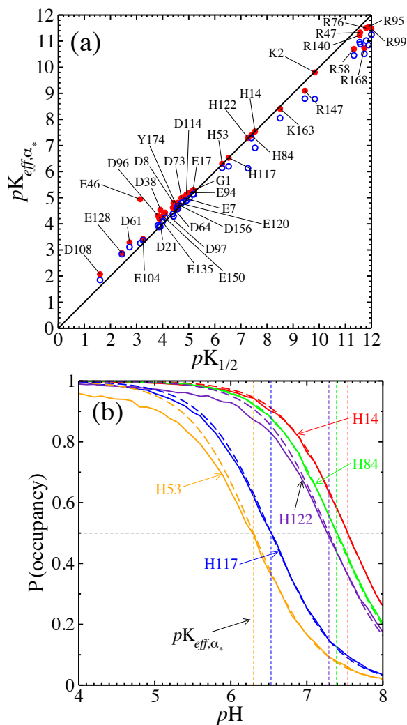
FIG. 15. (color online) (a): pK_{1/2} values from simulations of the full model with interactions, on the horizontal axis, are close to pK_{\text{eff}, \alpha_*} values. Red dots result from taking \alpha_* to be the most prominent protonation configuration within 6.6 < \text{pH} < 7.3 ; pK_{1/2} values further from 6.6 < pK_{1/2} < 7.3 differ from those pK_{\text{eff}, \alpha_*} , as expected. Blue open circles result from taking \alpha_* to be the most prominent configuration within 4.4 < \text{pH} < 4.6 ; again pK_{1/2} values further from that of \alpha_* differ more from those of pK_{\text{eff}, \alpha_*} . (b): Except for H53 and H122 below their respective pK_{1/2} s, histidine titration curves from the full model (solid) also agree well with Henderson-Hasselbalch curves (dashed) as parametrized by the pK_{\text{eff}, \alpha_*} values of the \alpha_* used in (a).
