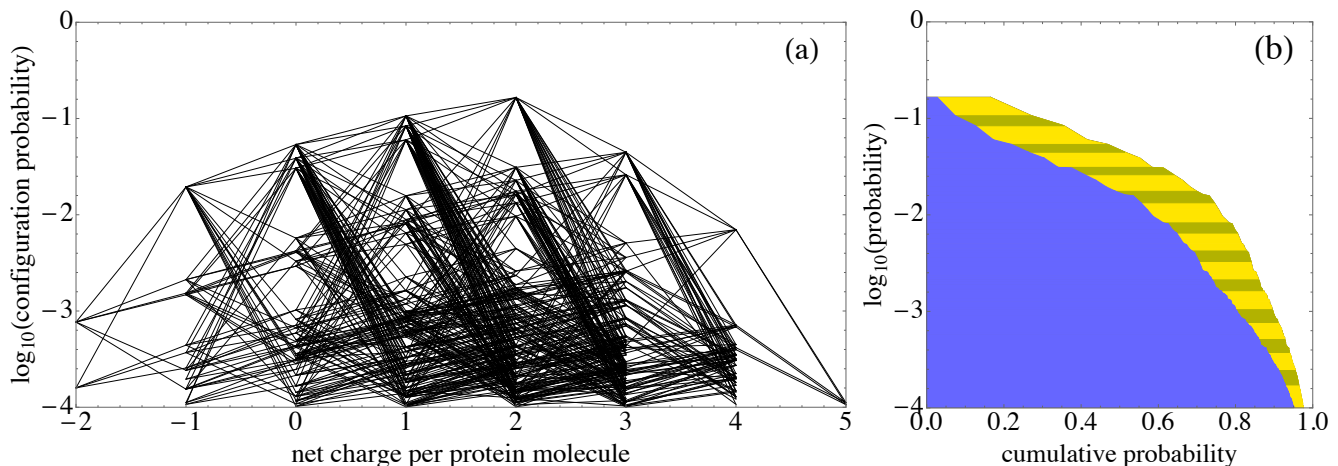
FIG. 5. (color online) Protonation patterns that have opposite net protein charge readily occur at pH 7.1. In both panels, \log_{10} P is plotted vertically for the most prominent pH 7.1 configurations that together account for over 97% of the configuration probability. (a): The net protein charge of each configuration is plotted horizontally. Line segments join configurations that can be transformed into one another with a single-residue protonation switch. (b): (i) The horizontal coordinate of the yellow-striped/clear boundary is the sum of the probabilities of that configuration and more common ones, that is, their cumulative probability. (ii) The horizontal coordinate of the blue/yellow-striped boundary is the square of the same, cumulative probability. The blue/yellow-striped boundary estimates the fraction of pairs of neighboring proteins, both molecules of which have one of the configurations down to a given \log_{10} P level; this estimate neglects biasing of pattern probabilities due to protein proximity.
