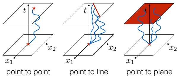
FIG. 3: Some typical polymer geometries for DP in d = 2 . See text for applications to the RW problem.
