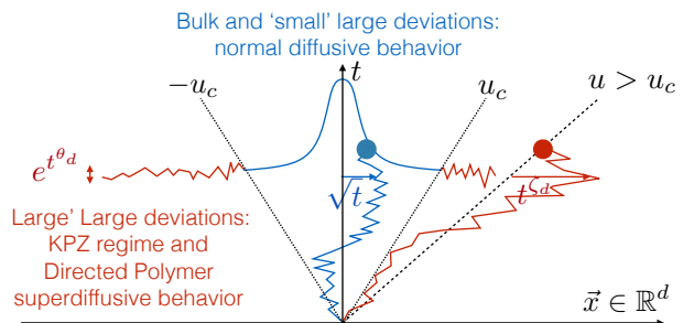
FIG. 1: Conjectural picture for TD-RWRE in arbitrary dimension d . While particles typically diffuse normally as if the random environment had been averaged out, particles conditioned on arriving away from the Gaussian bulk of the distribution in the ‘large large deviations regime’ (for |x(t)| > u_c t ) are superdiffusive with the roughness exponent of the directed polymer in the pinned phase \zeta_d > 1/2 . In this regime, fluctuations of the logarithm of the transition probability are large (scale with t^{\theta_d} with \theta_d = -1 + 2\zeta_d > 0 ) and identical to those of the height in the rough phase of the KPZ equation. The two phases are separated by an Edward-Wilkinson regime of fluctuations when x = u_c t + o(t) . In d = 1, 2 u_c = 0 while for d \geq 3 there is a phase transition with u_c \neq 0 . If an external bias \vec{f} is added, the bulk is around \vec{x} \sim \vec{f}t and the transition occurs for \vec{x} = \vec{u}t with |(\vec{f} + \vec{u})| = u_c .
