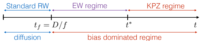
FIG. 2: The behavior of the RW crosses over from a diffusive to a bias dominated regime when t \sim t_f . The latter is also subdivided in between a EW regime and a KPZ regime for t^* \gg t_f (see text for an estimation of t^* in d = 1, 2 ).
