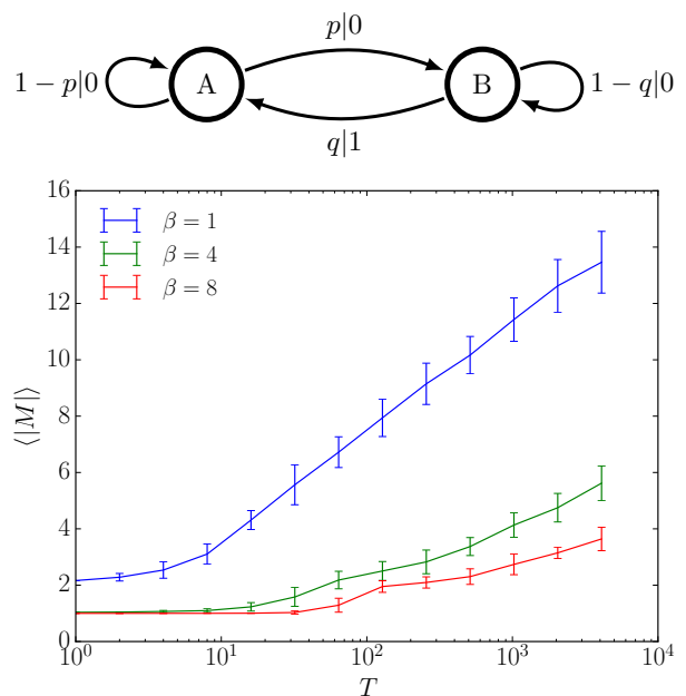
FIG. 2. Model-size scaling for the parametrized Simple Nonunifilar Source (SNS). (Top) Generative HMM for the SNS. (Bottom) Scaling of \langle |M| \rangle = \sum_M |M| P(M|x_{0:T}) with T , with the posterior P(M|x_{0:T}) calculated using formulae from BSI [34] with \alpha = 1 and the set of model topologies being the eventually Poisson \epsilon -machines described in Ref. [36]. Data generated from the SNS with p = q = \frac{1}{2} . Linear regression reveals a slope of \approx 1 for \log \log T vs. \log \langle |M| \rangle , confirming the expected N_T \approx \log T , where the proportionality constants depend on \beta . Curves from top to bottom: \beta = 1, 4, 8 and (online) blue, green, and red, respectively.
