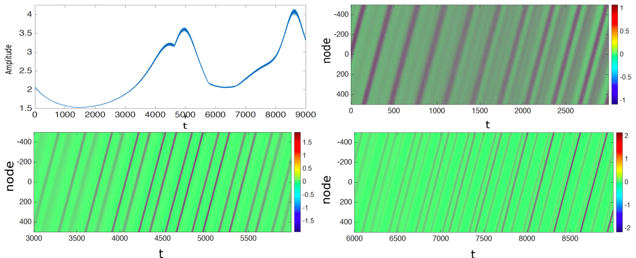
FIG. 7: (Color online) Evolution through the left handed metamaterial lattice of a Peregrine soliton for \omega = 1.926 ( f \approx 503 kHz in physical units), and g = 0.056 . Here, Eq. (12) is utilized to obtain the initial condition in the original variables. The top left panel shows the evolution of the solution's maximum. The top right, bottom left and bottom right panels show a very long space-time contour plot for the evolution of the voltage. For the formation of a large-amplitude (extreme) event and the subsequent splitting see details in the text.
