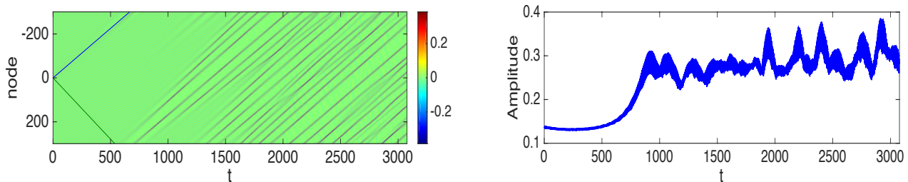
FIG. 6: (Color online) Evolution of a Peregrine soliton in the left-handed metamaterial lattice, for parameter values as in the left panel of Fig. 3. The left panel shows the space-time contour plot of the lattice, while the right panel the evolution of the maximum voltage amplitude. Note that, in physical units, the initial and maximum values of the voltage are 1.03 V and 2.7 V, respectively.
