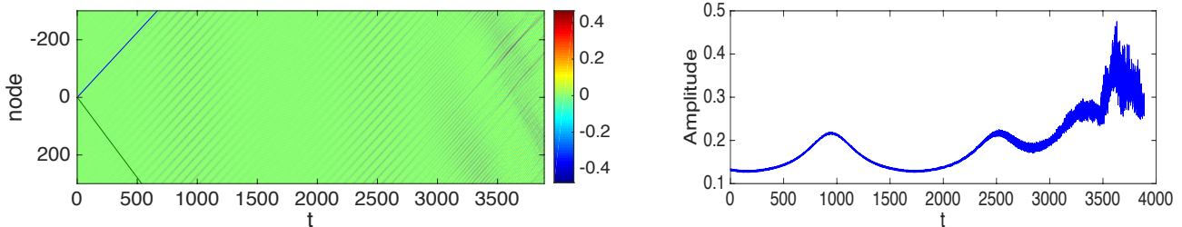
FIG. 8: (Color online) Evolution through the left handed metamaterial lattice of an Akhmediev breather for f \approx 200 kHz, and g = 0.056 . We use Eq. (13) with a = 0.1131 to obtain the initial condition in the original variables. Here, we start from time before the formation of maximum amplitude of Akhmediev breather. Once again, the space-time contour plot of the voltage (left) and of the maximal evolution of the voltage amplitude over time (right) are shown. In this case, in physical units, the initial and maximum values of the voltage are 0.98 V and 3.6 V, respectively.
