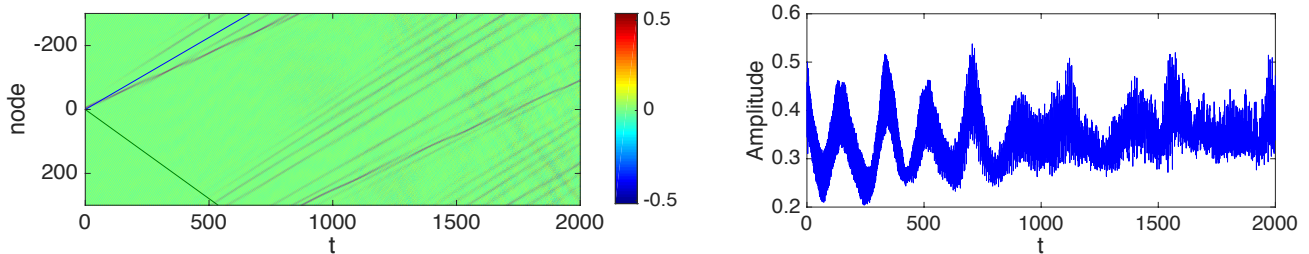
FIG. 10: (Color online) Evolution through the left handed metamaterial lattice of a Kuznetsov-Ma soliton for f \approx 200 kHz and g = 0.056 . The solution of Eq. (13) with a = 0.9 is utilized to obtain the initial condition in the original variables. The same diagnostics, namely voltage space-time contour plot (left panel) and maximal voltage vs. time (right panel) are depicted. In this case, in physical units, the initial and maximum values of the voltage are 3.4 V and 4.0 V, respectively.
