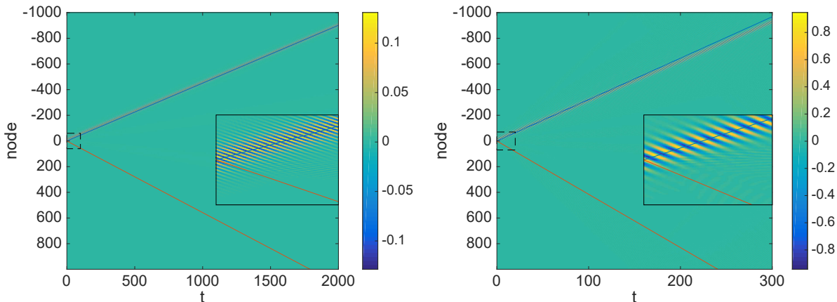
FIG. 3: (Color online) Contour plots depicting the space (node)-time ( t ) evolution of a bright soliton propagating through the left-handed medium. Note that v_p > 0 and v_g < 0 , as seen by the slopes of the lower and upper straight lines, respectively. In both panels, insets zooming in the initial stage of the evolution highlight the fact that v_p v_g < 0 , as is the case for a left-handed medium. The soliton clearly propagates with the prescribed group velocity. The initial data are obtained from the bright soliton solution of Eq. (10) with u_0 = 1 , c = 0 . For the quasi-continuum, long-wavelength approximation, we use \epsilon = 0.1 , and (k, \omega) \approx (1.3823, 0.7712) on the left panel, (k, \omega) \approx (0.4650, 1.9305) on the right panel; respective values in physical units are: (k, f) \approx (1.3823 \text{ cm}^{-1}, 200 \text{ kHz}) and (k, f) \approx (0.4650 \text{ cm}^{-1}, 501 \text{ kHz}) . The maximum soliton amplitude is 0.93 V (left panel) and 6.7 V (right panel); in both cases, g = 0.056 .
