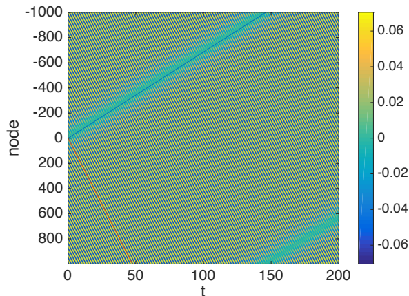
FIG. 5: (Color online) Dark soliton space-time contour plot evolution for g = 0.056 . The initial data for the dark soliton solution are obtained on the basis of Eq. (11) using u_0 = 0.1 , A = 0 , B = 1 , K = 0 , \epsilon = 0.1 and (k, \omega) \approx (0.1649, 3.4681) [i.e., (k, f) \approx (0.1649 \text{ cm}^{-1}, 900 \text{ kHz}) , in physical units]. The background voltage amplitude is 0.53 V. We observe the nearly undistorted propagation of the dark soliton which is now supported by the defocusing NLS model.
