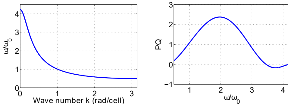
FIG. 2: (Color online) Left panel: the linear dispersion relation – cf. Eq. (7). Right panel: the dependence of the factor PQ (which determines the focusing or defocusing nature of the model) on the frequency \omega ; see also the text. When PQ > 0 , the nonlinearity is self-focusing while for the opposite sign, it is self-defocusing.
