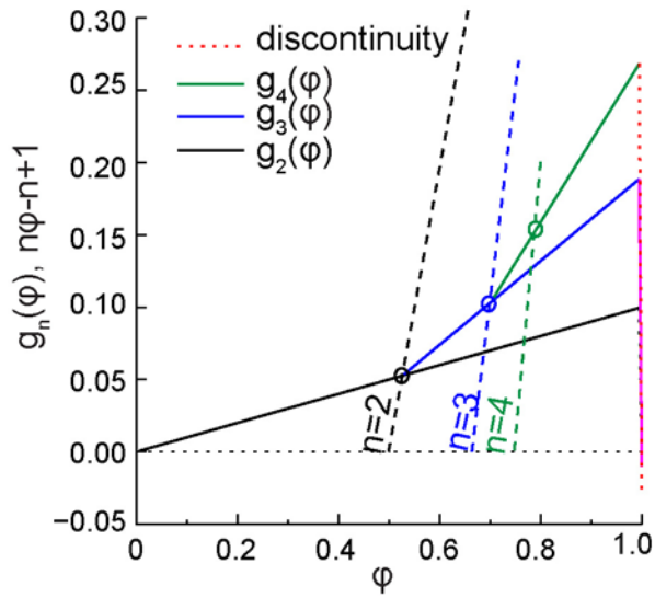
Figure 3. Graphical method. The phase of the last input ( \phi_n^* , indicated by the open circles) received by each cluster in an n -cluster mode with no delay falls at the intersection of these two functions described in the text.
