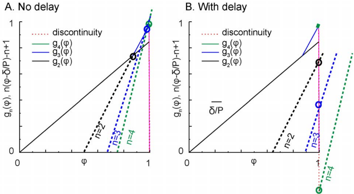
Figure 5. How delays destroy cluster modes. The intersection of the g functions with the dashed lines labeled with n=2, 3 or 4 gives the phase of the last input for cluster modes. (A) With no delay and a linear PRC with slope 0.85, cluster modes 2, 3 and 4 are stable. B. A normalized delay shown by the labeled bar shifts all lines to the left, destroying all cluster modes and leaving virtual (or ghost) repellers in their wake. This particular PRC with the illustrated delay guarantees that global synchrony is globally attracting, see text.
