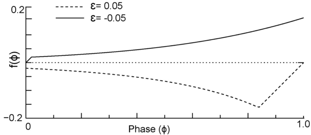
Figure 1. PRCs for leaky integrate and fire oscillator. S_0 = 1.0 and \gamma = 0.9 . These PRC shapes result when an instantaneous change in voltage of magnitude epsilon is applied to an oscillator with a monotonically increasing concave down membrane potential waveform between threshold crossings that result in a reset. Excitatory pulse coupling (dashed lines) and inhibitory pulse coupling (solid lines) each have two regions, a linear region where the slope is one due to the requirement to keep the phase between zero and 1, and a region in which the advance or delay increase with phase.
