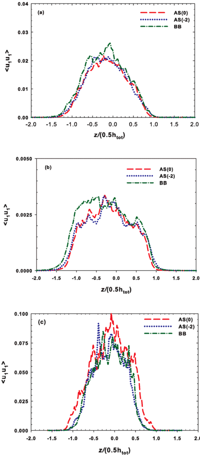
Figure 16. Spatial profiles of \langle u_1 u_1 \rangle at a) Z=8 cm b) Z=16 cm and c) Z=24 cm for all ICs.
