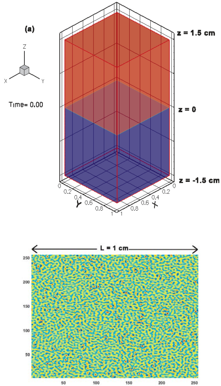
Figure 1. (a) Schematic of the computational domain used in simulations. The box size is 1 \times 1 \times 3 \text{ cm} (in the x -, y - and z - directions) with densities \rho_1 = 3.0 \text{ g/cm}^3 (red: heavy), \rho_2 = 1.0 \text{ g/cm}^3 (blue: light). (b) Contour plot of initial amplitudes at center-plane ( z = 0 ); the amplitudes correspond to annular narrowband ICs with energy in modes 32-64
