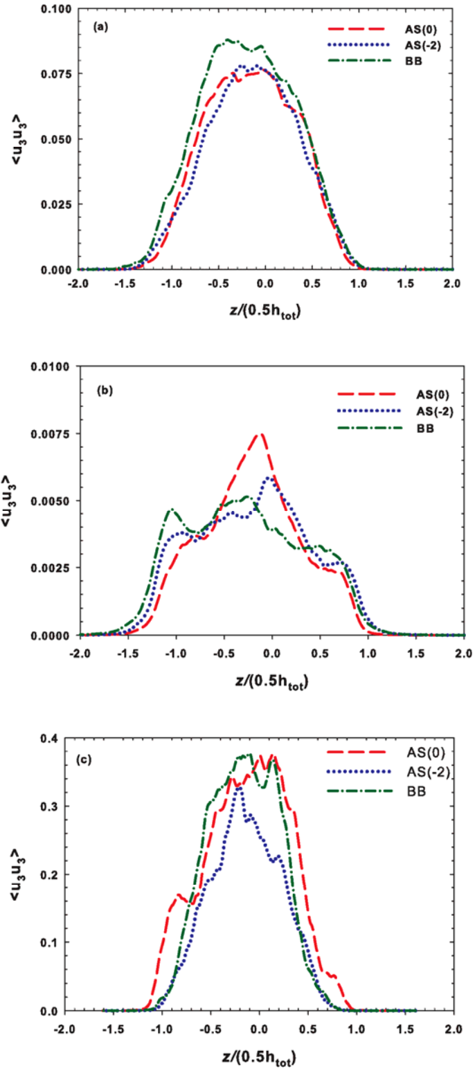
Figure 17. Spatial profiles of \langle u_3 u_3 \rangle at a) Z=8 cm b) Z=16 cm and c) Z=24 cm for all ICs.
