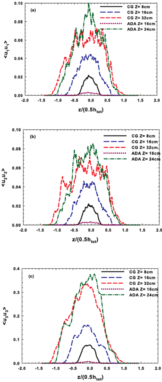
Figure 13. Spatial profiles of a) \langle u_1 u_1 \rangle , b) \langle u_2 u_2 \rangle and c) \langle u_3 u_3 \rangle for both CG_AS-0 and AS-0 at different Z values.
