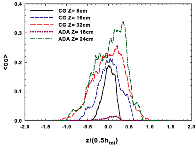
Figure 15. Spatial profiles of \langle cc \rangle for both CG_AS-0 and AS-0 at different Z values.
