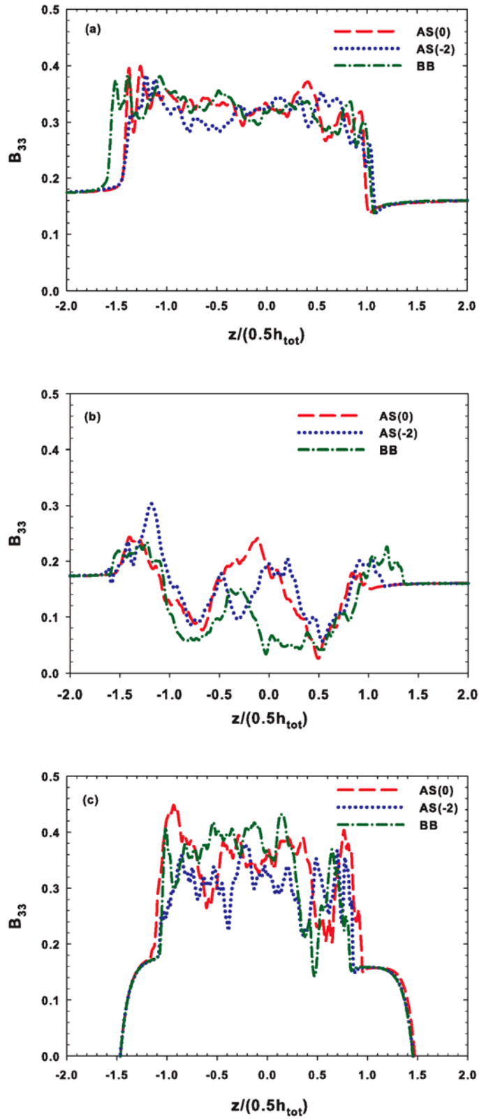
Figure 18. Spatial profiles of B_{33} at a) Z=8 cm b) Z=16 cm and c) Z=24 cm for all ICs.
