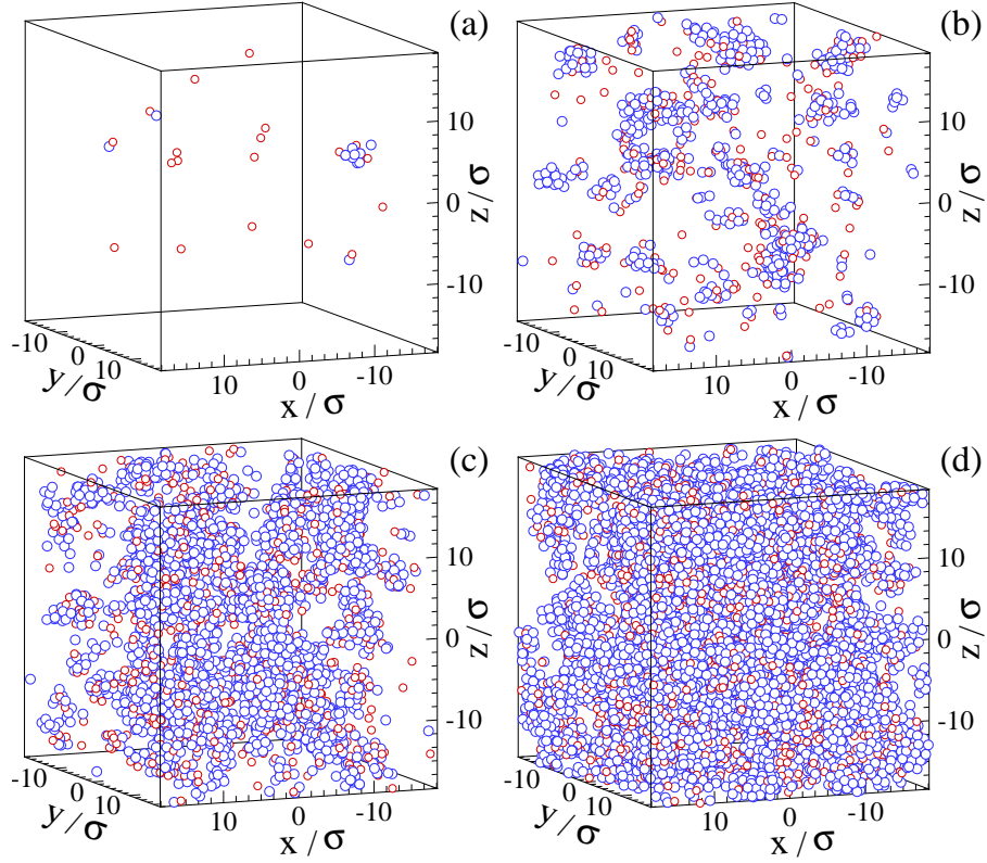
FIG. 5: (Color online) Spatial configurations of atoms with large nonaffine displacements after a quarter of a cycle, D^2(t, T/4) > 0.01 \sigma^2 , for the strain amplitudes (a) \gamma_0 = 0.00 , (b) \gamma_0 = 0.02 , (c) \gamma_0 = 0.04 , and (d) \gamma_0 = 0.06 . The atoms of type A and B are denoted by blue and red circles.
