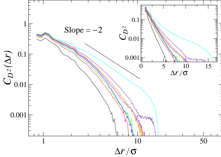
FIG. 6: (Color online) The correlation function C_{D^2}(\Delta \mathbf{r}) defined by Eq. (4) for the strain amplitudes \gamma_0 = 0, 0.01, 0.02, 0.03, 0.04, 0.05, 0.06, 0.07, 0.08 (from left to right). The straight line with the slope -2 is plotted for reference. The inset shows the same data on the log-normal scale.
