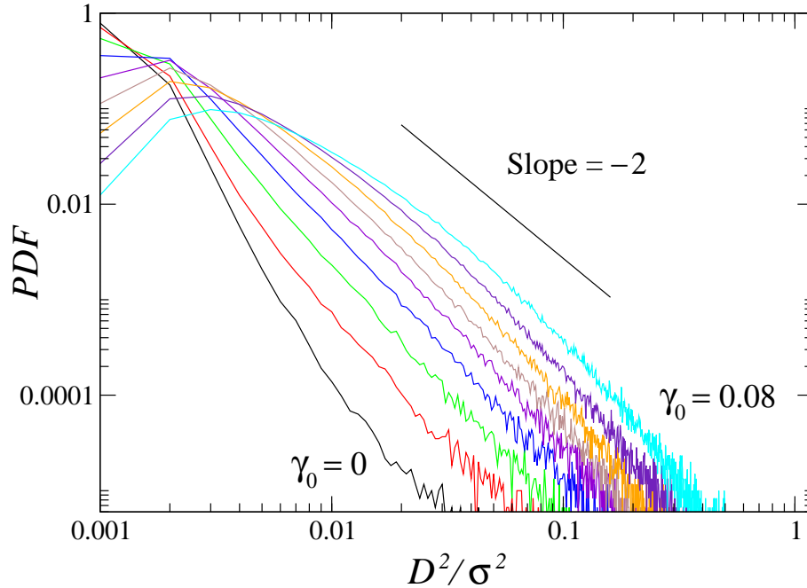
FIG. 3: (Color online) The probability distribution function of D^2(t, T/4) for the strain amplitudes \gamma_0 = 0, 0.01, 0.02, 0.03, 0.04, 0.05, 0.06, 0.07, 0.08 (from left to right). The straight solid line indicates the slope -2 .
