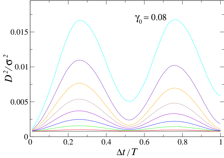
FIG. 4: (Color online) Variation of the averaged quantity D^2(t, \Delta t) during one oscillation period for the strain amplitudes \gamma_0 = 0, 0.01, 0.02, 0.03, 0.04, 0.05, 0.06, 0.07, 0.08 (from bottom to top).
