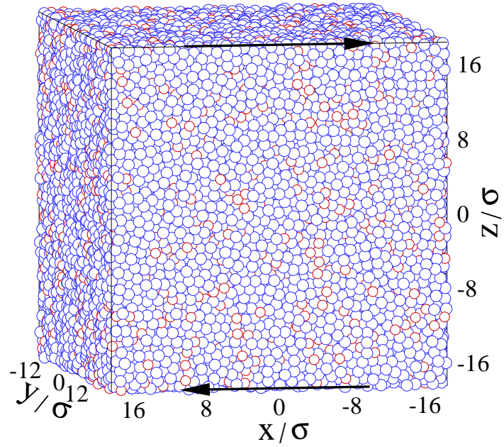
FIG. 1: (Color online) The instantaneous atomic positions for a binary LJ glass annealed with a slow cooling rate of 10^{-5} \varepsilon/k_B\tau to the temperature T_{LJ} = 10^{-2} \varepsilon/k_B . Atoms of type A are shown by large blue circles and type B by small red circles. The arrows indicate the plane of periodic shear deformation.
