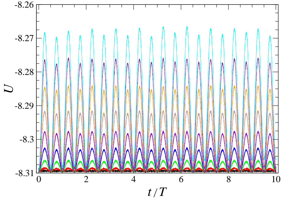
FIG. 2: (Color online) The potential energy per atom U (in units of \varepsilon ) during ten oscillation cycles for the strain amplitudes \gamma_0 = 0, 0.01, 0.02, 0.03, 0.04, 0.05, 0.06, 0.07, 0.08 (from bottom to top).
