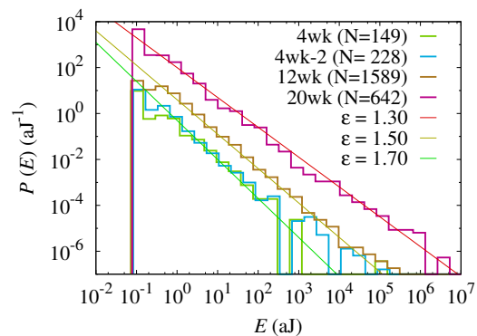
FIG. 4: Distribution of AE event energies in log-log scales for samples of pigs of 4 (4wk and 4wk-2), 12 (12wk) and 20 (20wk) weeks. The continuous lines indicate the power-laws with exponents obtained from the study of maximum likelihood maps.
