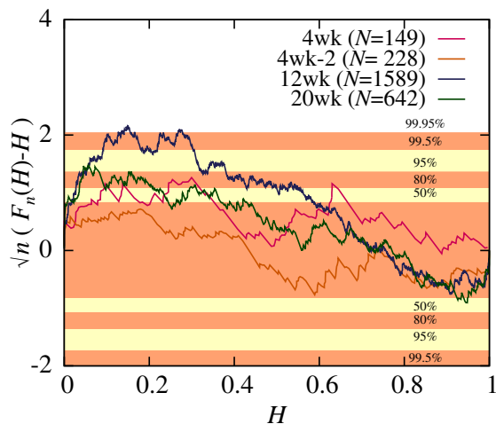
FIG. 9: Kolmogorov-Smirnov test of uniformity of the variable H obtained from the Bi-test analysis of the AE signals corresponding to samples of pigs of 4 (4wk and 4wk-2), 12 (12wk) and 20 (20wk) weeks. The colored horizontal bands show rejection probabilities of the local Poisson hypothesis.
