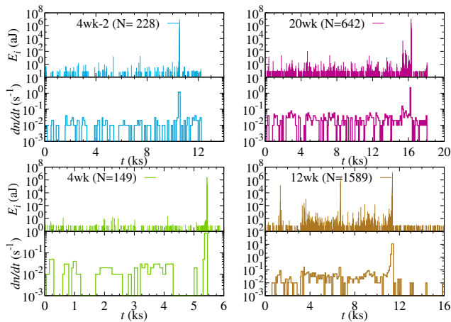
FIG. 3: Signal energy (top panels) and AE activity (bottom panels) as a function of time for samples of pigs of 4 (4wk and 4wk-2), 12 (12wk) and 20 (20wk) weeks. The activity is obtained with time intervals of 100 s. The total number of recorded signals N in each experiment is indicated in the panels.
