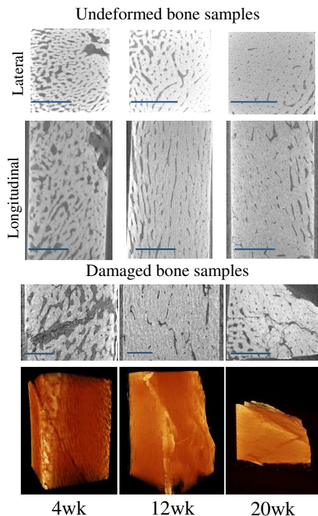
FIG. 1: Micro-CT images of 4wk, 12wk and 20wk samples (using 5 \mu\text{m} resolution). Two top rows show select close up slices of undeformed specimens in lateral and longitudinal planes. Third row shows 2D images of damaged specimens after loading them up to 1% strain. Images were taken in unloaded state. Length bars are 1 mm. Last row represents 3D images. Note that 12wk and 20wk specimens broke in two parts.
