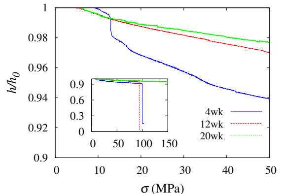
FIG. 2: Relative deformation, h/h_0 , vs. compressive stress for samples of selected pig ages.
