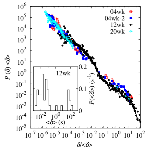
FIG. 8: Same data as in Fig. 7 represented after scaling with the rate, for thresholds increasing by a factor 2 and starting at E = 0.01 aJ. The inset gives the distribution of AE rates averaged over fifty successive events for AE data corresponding to the sample 12wk.
