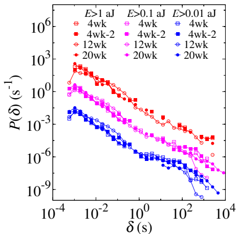
FIG. 7: Non-scaled representation of the waiting times with threshold fixed at E > 0.01 aJ, E > 0.1 aJ and E > 1 aJ for AE data corresponding to samples of pigs of 4 (4wk and 4wk-2), 12 (12wk) and 20 (20wk) weeks. For the sake of clarity curves corresponding to E > 0.1 aJ and E > 1 aJ have been shifted upwards two decades.
