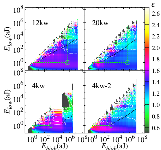
FIG. 5: Maximum likelihood maps for AE data corresponding to samples of pigs of 4 (4wk and 4wk-2), 12 (12wk) and 20 (20wk) weeks. The energy exponent that characterizes the energy distribution within the boundaries E_{low} and E_{high} is color coded. The exponent value has been chosen from data inside the green circle. See text for more details.
