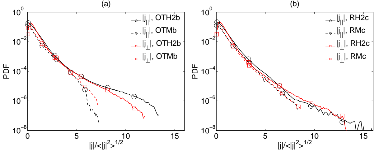
FIG. 9. (Color Online) (Panel a) Distributions of |j_{||}| = |\mathbf{j} \cdot \mathbf{b}|/|\mathbf{b}| (black circles) and |j_{\perp}| = \sqrt{|\mathbf{j}|^2 - |j_{||}|^2} (red squares) for runs OTH2b (solid lines) and OTMb (dashed lines). (Panel b) Same as panel a but for runs RH2c (solid lines) and RMc (dashed lines). The magnitudes are normalized to the standard deviation of the current. The HMHD runs have wider wings to the distributions than the MHD runs.
