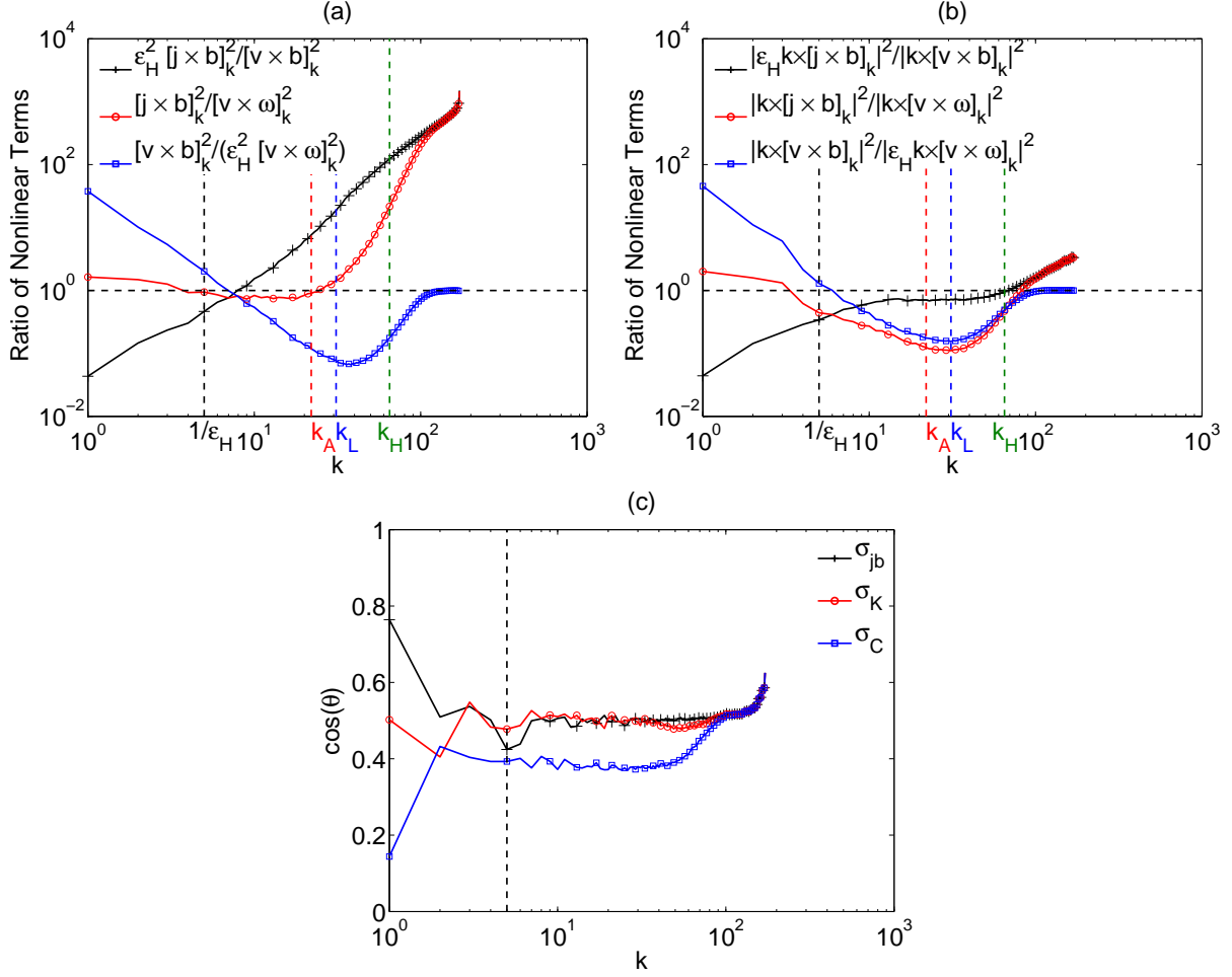
FIG. 6. (Color Online) (Panel a) Ratios of the spectra of the nonlinear terms present in the magnetic vector potential, velocity, and “uncurled” \Omega_L equations. The horizontal dashed line marks a value of unity, and the vertical dashed lines mark the ion inertial length ( 1/\epsilon_H ), and dissipation scales given by Eq. 5 ( k_A , k_L , and k_H ). (Panel b) Same as panel a but for the nonlinear terms in the induction, vorticity, and \Omega_L equations. (Panel c) Spectra of the cosine of the angles between the vectors involved in the nonlinear terms ( \sigma_{jb} , \sigma_K , and \sigma_C ). In creating the spectra, the absolute value of the correlation is taken before averaging over spherical shells so as to avoid cancellation of positive and negative alignment. The vertical dashed line gives the ion inertial length. All three plots are for run RH2c. Other HMHD runs show the same general behavior.
