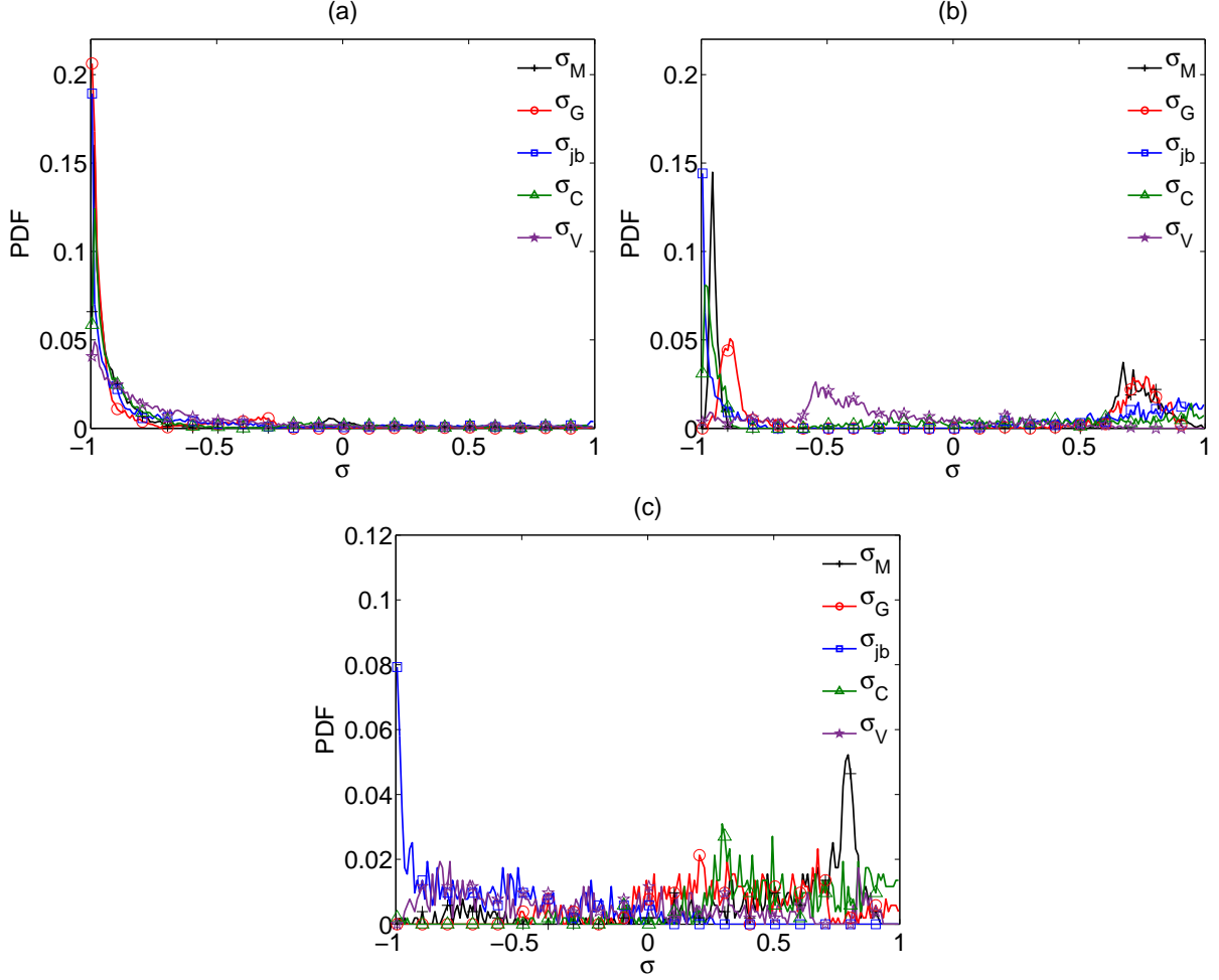
FIG. 8. (Color Online) Conditional PDFs of \sigma_M , \sigma_G , \sigma_{jb} , \sigma_C , and \sigma_V for points where |j| is greater than 75% of the maximum. Panels a and b show run OTH2b at the time of peak \Omega_T and 1.2 times the time of peak \Omega_T respectively. Panel c shows run RH2c at the time of peak \Omega_T . At all times and initial conditions examined, peaks in the conditional PDF for \sigma_{jb} are present at either +1 or at -1 (as plotted here).
