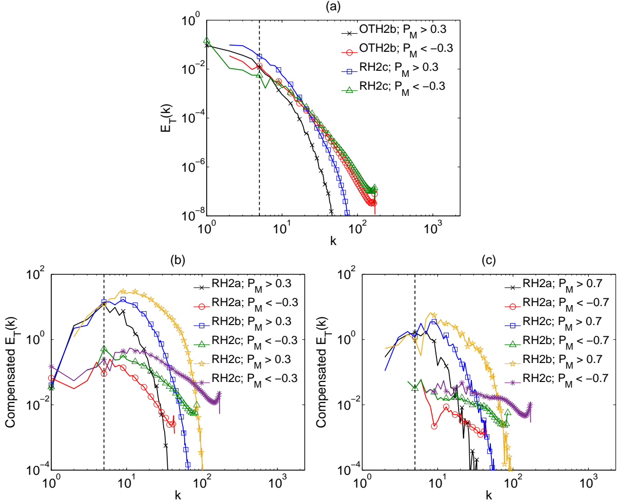
FIG. 3. (Color Online) (Panel a) Spectra for fluctuations with |P_M| > 0.3 for runs OTH2b and RH2c. (Panel b) Spectra for the same values of P_M as panel a, but compensated by either k^{11/3} for positive P_M (left polarized ion cyclotron fluctuations) or k^{7/3} for negative P_M (right polarized whistler fluctuations) as predicted and observed in hyperdiffusive simulations by Meyrand and Galtier [47]. (Panel c) Spectra with |P_M| > 0.7 compensated by either k^{11/3} for positive P_M or k^{7/3} for negative P_M . The compensated spectra are for runs RH2a, RH2b, and RH2c, which have various Reynolds numbers. In all panels, vertical dashed lines mark 1/\epsilon_H .
