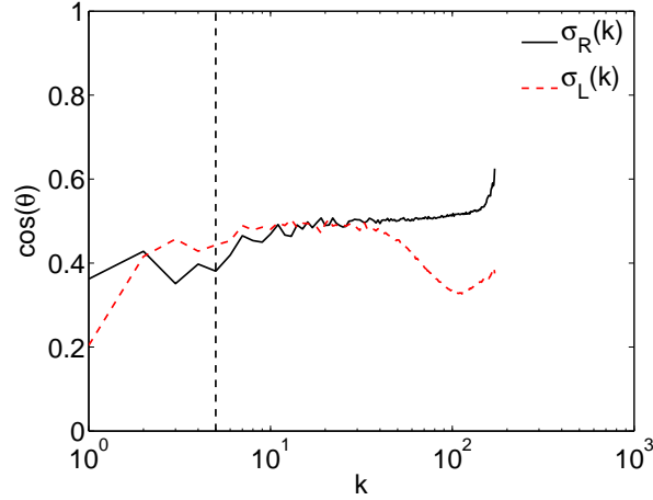
FIG. 5. (Color Online) Spectra of the alignments associated with the double curl Beltrami state [58] for run RH2c. The solid black curve gives \sigma_R and the red dashed curve gives \sigma_L . An absolute value is taken before averaging over spherical shells to avoid cancellation of positive and negative alignment. The vertical dashed line marks 1/\epsilon_H .
