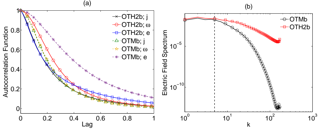
FIG. 10. (Color Online) (Panel a) Autocorrelation functions of the current, vorticity, and electric field for runs OTH2b (solid lines) and OTMb (dashed lines). In MHD, the current and vorticity autocorrelation functions are nearly identical consistent with current and vorticity structures that are of similar scales. In HMHD, the current autocorrelation function is narrower and the vorticity autocorrelation function is wider consistent with thinner current structures and wider vorticity structures. Electric field structures are much narrower and follow the current autocorrelation function at small separations in HMHD. (Panel b) Spectra of \mathbf{e} (Fourier transform of \mathbf{e} autocorrelation function) for runs OTMb (black circles) and OTH2b (red squares). The vertical dashed line marks 1/\epsilon_H .
