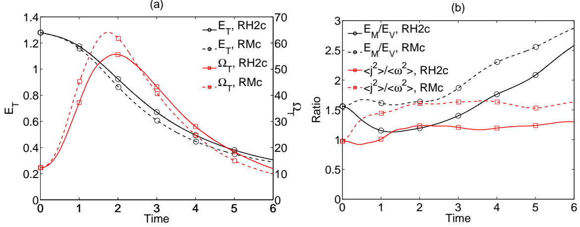
FIG. 1. (Color Online) (Panel a) Total energy (black circles) and enstrophy (red squares) as a function of time for RMc (dashed lines) and RH2c (solid lines). (Panel b) Ratio of magnetic to kinetic energy and ratio of mean square current to mean square vorticity as a function of time for the same runs and in the same format as in Panel a.
