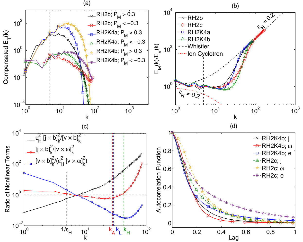
FIG. 11. (Color Online) (Panel a) Energy spectra for Fourier modes with |P_M| > 0.3 for the two hyperdiffusive runs, as well as run RH2b for comparison. The spectra for negative P_M are compensated by k^{7/3} and the positive P_M spectra are compensated by k^{11/3} . The vertical dashed line marks 1/\epsilon_H . (Panel b) E_M(k)/E_V(k) for the two hyperdiffusive runs with runs RH2b and RH2c (note that this run has 512^3 resolution) for comparison. The vertical dashed line marks 1/\epsilon_H . (Panel c) Ratio of nonlinear terms in the magnetic vector potential equation, momentum equation, and “uncurled” \Omega_L equation for run RH2K4b. The horizontal dashed line denotes unity and the four vertical dashed lines mark the scales 1/\epsilon_H , k_A , k_L , and k_H . (Panel d) Autocorrelation functions for the current, vorticity, and electric field in run RH2K4b and RH2c for comparison.
