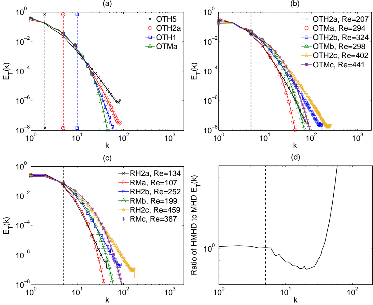
FIG. 2. (Color Online) (Panel a) E_T(k) for runs OTMa, OTH1, OTH2a, and OTH5, which have varying values of \epsilon_H . Vertical dashed lines mark 1/\epsilon_H with colors and markers corresponding to the run. (Panel b) E_T(k) for runs OTMa,b,c and OTH2a,b,c, which have varying Reynolds numbers. (Panel c) E_T(k) for runs RMa,b,c and RH2a,b,c, which have varying Reynolds numbers. In panels b and c, Reynolds numbers Re = \langle |\mathbf{v}|^2 \rangle L_{int} / \nu at the peak of \Omega_T are given in the legend. (Panel d) Ratio of E_T(k) for run RH2c to E_T(k) for run RMc. The region of negative slope indicates where HMHD is steeper than MHD. In panels a, b, and c vertical dashed lines show 1/\epsilon_H .
