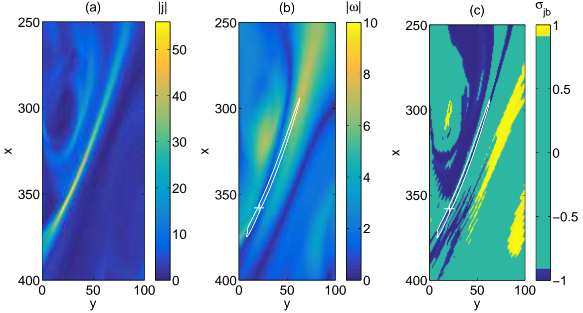
FIG. 7. (Color Online) 2D cuts of |\mathbf{j}| (panel a), |\boldsymbol{\omega}| (panel b), and \sigma_{jb} (panel c) at the location of maximum current near the peak of \Omega_T for run OTH2b. White crosses mark the location of maximum current and white curves give the half-maximum contours of the current. Values of |\sigma_{jb}| < 0.9 are masked out to highlight the highly-aligned structures. The x and y axes are in units of grid points.
