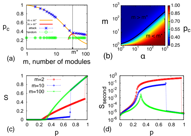
FIG. 2. (Color online) Two percolation regimes when attacking interconnected nodes. (a) p_c as a function of m calculated for ER networks with k = 4 , \alpha = 100 . Simulation points obtained from at least 1000 simulation runs of networks of size N = 600\,000 . Solid lines represent the analytical result obtained in Eqs. 15 and 19. (b) Two-parameter ( \alpha , m ) phase diagram for a fixed mean degree k = 4 . The black line corresponds to the critical number of modules m^* obtained from Eq. 22. (c)-(d) Fraction of nodes in the largest cluster S and second largest cluster S_{\text{second}} respectively, with solid lines representing the analytical result obtained in Eq. 24 and symbols are from simulations.
