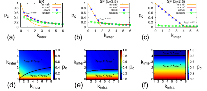
FIG. 5. (Color online) Critical concentration of interconnected nodes (a)-(c) p_c as a function of k_{inter} calculated for (a) ER and (b)-(c) SF networks with m = 10 and k_{intra} = 2 . Simulation points obtained from at least 1000 simulation runs of networks of size N = 600\,000 . Solid lines represent the analytical result obtained in Eqs. 19,25-27. (d)-(f) Two-parameter (k_{intra}, k_{inter}) phase diagram for a fixed number of modules m = 10 . The black line corresponds to the critical mean inter-degree k_{inter}^* at which the two p_c solutions cross.
