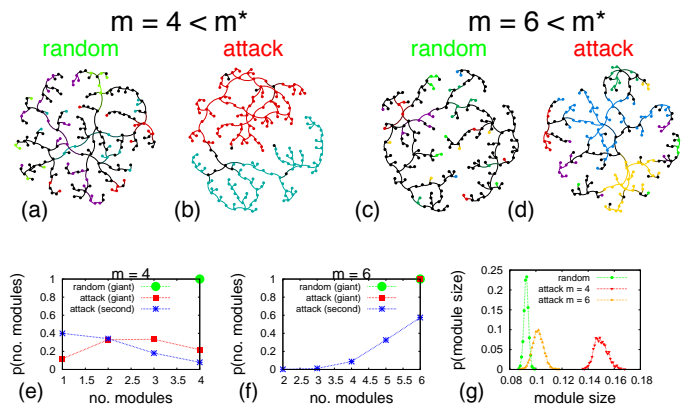
FIG. 3. (Color online) Size of modules in the giant component at S = 0.1 . Visualization is shown for networks of size N = 2000 with mean degree k = 4 and \alpha = 10 , at the point where the giant component contains 10% of the nodes ( S = 0.1 ) (a),(c) for random node removal, (b),(d) for attack on interconnected nodes. (e)-(f) Distribution of the number of modules in the giant component and second largest component at S = 0.1 . A module is considered to be part of a component if at least one of its nodes are part of the component. (g) Distribution of the size of modules in the giant component at S = 0.1 , normalized by the initial module size. Note that in (g), the size of modules is measured by reconstructing the graph of each module in the giant component, and counting its number of nodes in this graph. In other words, interconnected nodes that have been detached from their original module are not considered. Results obtained by at least 1000 simulation runs of networks of size N = 600\,000 with mean degree k = 4 .
