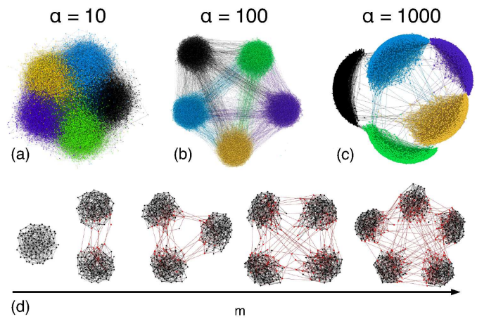
FIG. 1. (Color online) Visualization of the model for generating random modular networks. (a)-(c) Illustration of the effect of \alpha on the obtained modular network using Gephi [38], on a Erdős-Rényi (ER) network of size N = 10\,000 with mean degree k = 8 divided into m = 5 modules. (d) Illustration of the effect of the number of modules m on the obtained network with a number of inter-module links increasing with the number of modules. Inter-connected nodes and links are shown in red (light gray).
