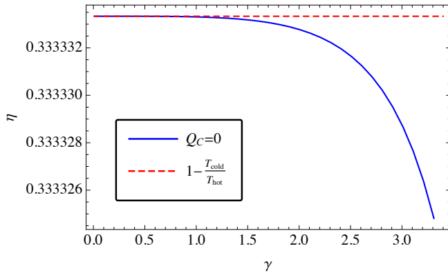
FIG. 2. (color online) Efficiency of the quantum Carnot cycle for Eq. (17). The blue, solid line results from W/Q_{\text{tot}} , which does not properly account for the house keeping energy Q_c . The red, dashed line is the Carnot efficiency (16). Parameters are T_{\text{cold}} = 1 , T_{\text{hot}} = 1.5 , \omega_1 = 0.2 , \omega_2 = 0.6 , \hbar = 1 , and m = 1 .
