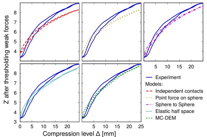
Figure 5: Number of contacts per grain Z after thresholding weak forces, averaged over multiple cycles.
