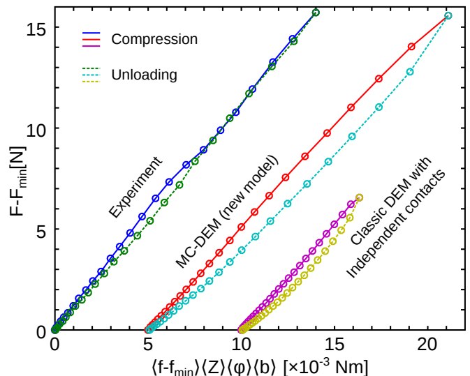
Figure 6: Validation that the scaling law from [8], derived from experimental data, also holds in the simulation. Here, F is the force exerted by the grains on the top plate, f is the average force at each contact, Z the number of contacts per grain, \phi is the volume fraction within the packing (starting one diameter away from walls) and b is the distance between grain centers. Microscopic quantities were averaged on all grains/contacts within the packing. Data was then averaged on the 15 retained compression or unloading phases with the same strain. Each marker in the diagram represents one such strain level. MC-DEM and the usual DEM data have been shifted for clarity by 5 and 10 mNm respectively.
