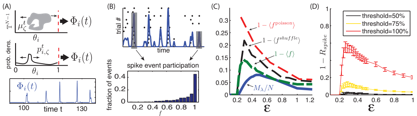
FIG. 4. (Colors online) (A) Top and middle: cartoon representations of the flux \Phi_i(t) . Bottom: sample \Phi_i time trace for a randomly chosen cell approximated from 1000 trajectories. (B) Top: Illustration of spike event definition. Bottom: Distribution of spike event participation fraction f . (For (A) and (B): \eta = -0.5 , \epsilon = 0.5 , \lambda_1 \simeq 2.5 ) (C) Curves of 1 - \langle f \rangle (network), 1 - \langle f^{shuffle} \rangle (single cell with shuffled input spike trains from networks simulations) and 1 - \langle f^{poisson} \rangle (single cell with random poisson spike inputs) vs. \epsilon . Also shown is the fraction of \lambda_i > 0 , M_\lambda/N vs. \epsilon . (D) Mean 1 - R_{spike} vs. \epsilon curves for three threshold values. Error bars show one standard deviation of mean R_{spike} across all cells in the network. (For (C) and (D): \eta = -0.5 )
