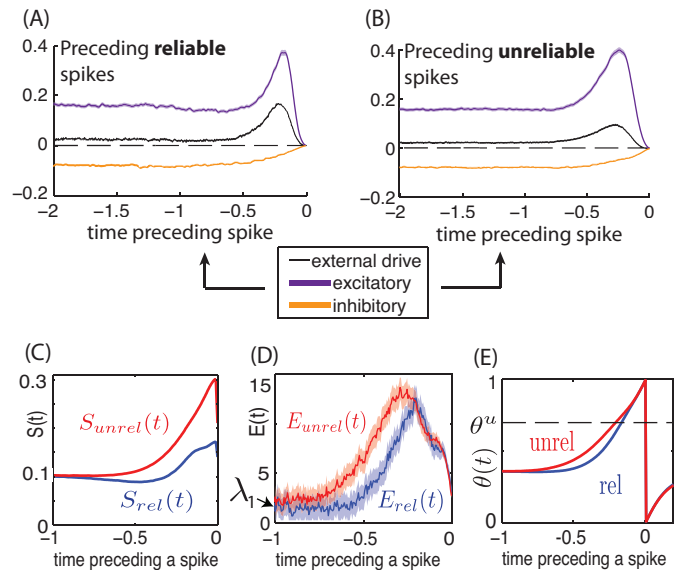
FIG. 5. (Color online) For (A) through (E), t = 0 marks the spike time and rel/unrel indicates the identity of the spike used in the average. (A) and (B), Spike triggered averaged external signal \varepsilon Z(\theta_i) \zeta_i(t) (black), excitatory (purple) and inhibitory (orange) network inputs Z(\theta_i) \sum_j a_{ij} g(\theta_j) . (A) Triggered on reliable spikes. (B) Triggered on unreliable spikes. (C) Spike triggered support score S . (D) Spike triggered local expansion measure E . (E) Spike triggered average phase \theta_i . For all panels: \eta = -0.5 , \varepsilon = 0.5 with \lambda_1 \approx 2.5 . Shaded areas surrounding the computed averages show two standard errors of the mean. a No shade indicates that the error is too small to visualize.
