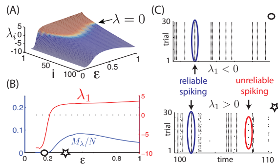
FIG. 2. (Color online) (A) First 100 Lyapunov exponents of network with fixed parameters as in Fig. 1, as a function of \epsilon . (B) Plot of \lambda_1 (right scale), M_\lambda/N : the fraction of \lambda_i > 0 (left scale) vs \epsilon . (C) Raster plots show example spike times of an arbitrarily chosen cell in the network on 30 distinct trials, initialized with random ICs. Circle and star markers indicate \epsilon values of 0.18 and 0.5, respectively, shown in panel (B). For all panels, \eta = -0.5 .
