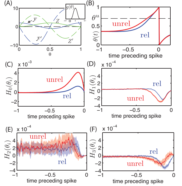
FIG. 6. (Colors online) (A) Distinct terms of the single cell flow and Jacobian. Inset : synaptic coupling function g(\theta) . For panels (B-F), t = 0 marks the spike time and rel/unrel indicate the identity of the spike used in the average. (B) Spike triggered average phase \theta_i (same as in Fig 5 E). (C-F) Spike triggered average terms H_0(\theta_i) , H_1(\theta_i) , H_2(\theta_i) and H_3(\theta_i) . Network parameters: \eta = -0.5 , \varepsilon = 0.5 , yielding \lambda_1 \simeq 2.5 . For all panels except (A): shaded areas surrounding the computed averages show two standard errors of the mean. a No shade indicates that the error is too small to visualize.
