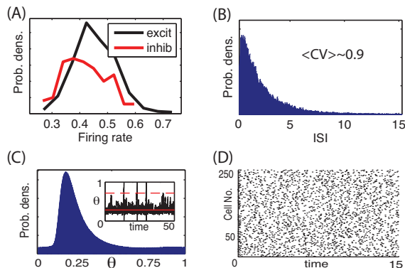
FIG. 1. (Color online) (A) Typical firing rate distributions for excitatory and inhibitory populations. (B) Typical inter-spike-interval (ISI) distribution of a single cell. The coefficient of variation (CV) is close to 1. (C) Invariant measure for an excitable cell ( \eta < 0 ); inset: typical trajectory trace of an excitable cell where solid and dotted lines mark the stable and unstable fixed points. (D) Network raster plots for 250 randomly chosen cells. For all panels, \eta = -0.5 , \varepsilon = 0.5 .
