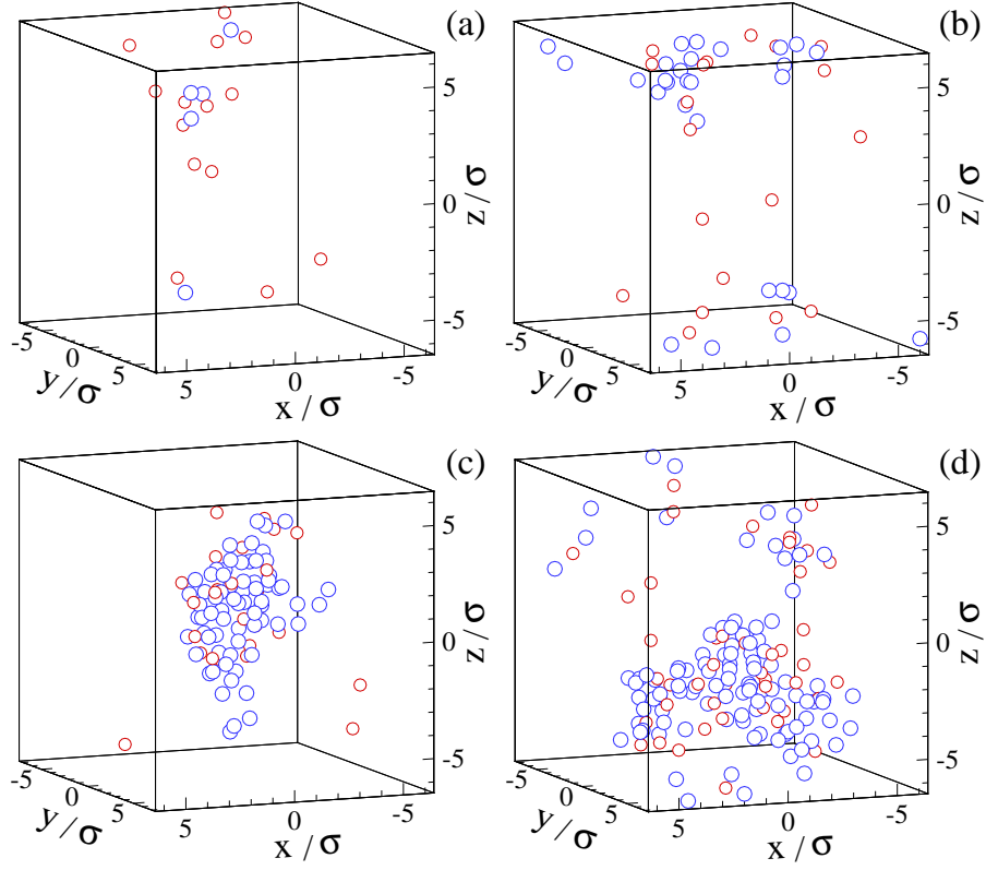
FIG. 6: (Color online) Typical clusters of mobile particles A (large blue circles) and B (small red circles) for the oscillation frequency \omega\tau = 0.02 and strain amplitudes (a) \gamma_0 = 0.02 , (b) \gamma_0 = 0.03 , (c) \gamma_0 = 0.04 , and (d) \gamma_0 = 0.05 .
