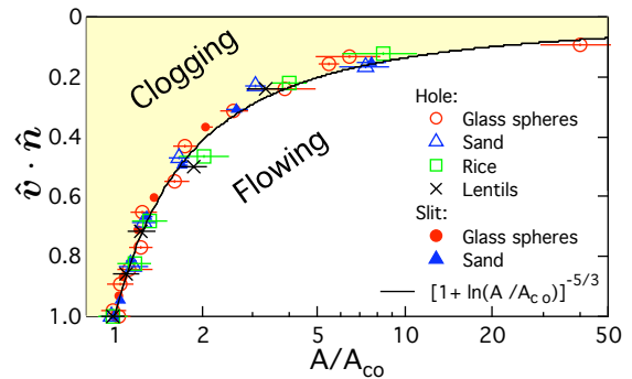
FIG. 10: (Color online) Clogging transition curves for most materials and both aperture geometries. The x -axis is the hole area, normalized by the critical hole area at zero tilt angle. The y -axis is the component \hat{v} \cdot \hat{n} of the average flow direction normal to the plane of the aperture (see Fig. 9 for illustration defining these unit vectors). The solid curve is an empirical fitting function; if allowed to float, the exponent is -1.84 \pm 0.02 .
