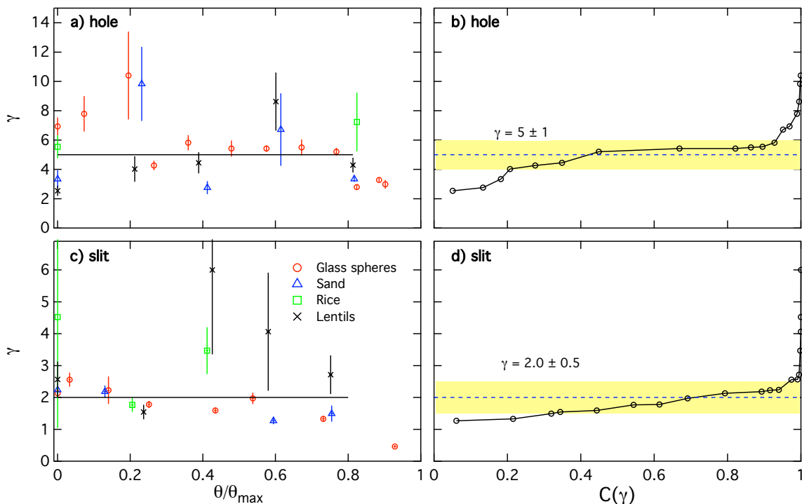
FIG. 5: (Color online) Exponents \gamma from fits to Eq. (3), versus \theta/\theta_{max} , for (a) circular holes and (c) long slits. The error bars \delta\gamma indicate the fitting confidence intervals. The average values of \gamma , weighted by 1/(\delta\gamma)^2 , for \theta/\theta_{max} < 0.8 , and the uncertainty in the means, are \gamma = 5.1 \pm 0.3 for circular holes and \gamma = 1.9 \pm 0.1 for long slits. The cumulative distributions C(\gamma) , with \Delta C(\gamma) increments proportional to 1/(\delta\gamma)^2 , are shown in (b) and (d) for holes and slits, respectively. There, eighty percent of the weight lies within the ranges 5 \pm 1 and 2.0 \pm 0.1 , as indicated by the yellow shading. This provides a conservative estimate of the exponents and their uncertainties.
