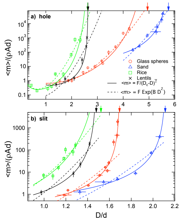
FIG. 4: (Color online) Dimensionless measure of the average mass discharged \langle m \rangle / (\rho_b A d) before a clog occurs versus dimensionless aperture size D/d . A is the aperture area, \rho_b is the material bulk density, and d is the long grain axis. For the circular hole, D is the hole diameter, while for the rectangular slit, D is the width of the slit. Plotted are data for (a) the circular hole and (b) the rectangular slit, for \theta = 0 . The average mass grows with D faster than exponential or even exponential squared (indicated by the dashed curves). Instead, \langle m \rangle versus D is better described by the power-law of Eq. (3), shown by the solid curves that diverge at critical aperture sizes D_c , indicated by the arrows. The exponents, \gamma , were adjusted as part of the fits and the values are given in Fig. 5. For the rice data, however, such fits did not converge and the exponents for the displayed fits were instead fixed to \gamma = 5 in (a) and \gamma = 2 in (b).
