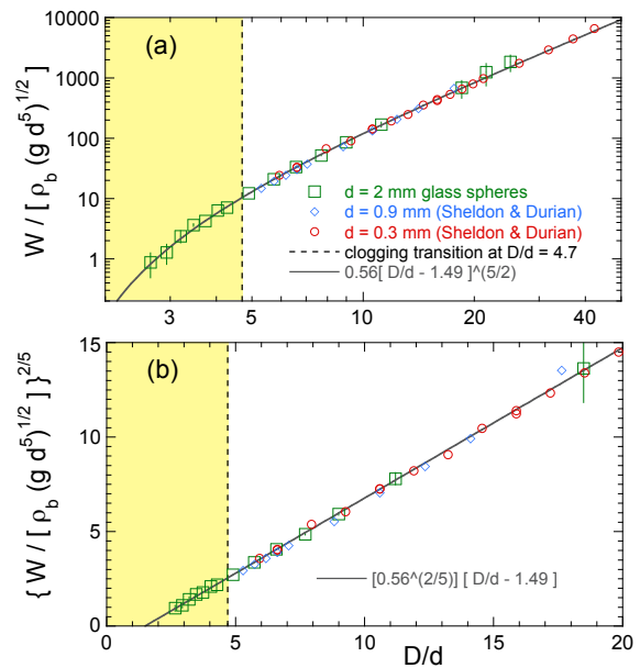
FIG. 1: (Color online) (a) Dimensionless discharge rate W/(\rho_b\sqrt{gd^5}) , and (b) the same quantity raised to the 2/5 power, for glass beads as a function of dimensionless hole diameter D/d , where W is the mass discharge rate, \rho_b is the bulk density of the packing, g = 9.8 \text{ m/s}^2 , and d is the grain diameter as labeled. The data for the d = 2 \text{ mm} spheres are new, while the other data are taken from Ref. [26]. The fit to the Beverloo form, Eqs. (1,2), gives C = 0.56 and k = 1.5 , and is shown a solid gray curve (a) and line (b). The shaded region to the left of D/d = 4.7 indicates where the system is susceptible to clogging
