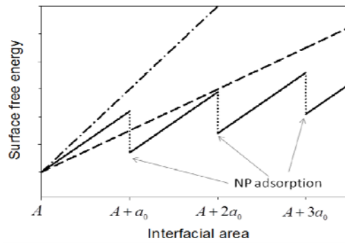
Figure 8. Schematic representing the variation in surface free energy as the interfacial area A increases. For a description of the various symbols and lines please refer to the text. a_0 is the interfacial area necessary for one NP to adsorb. \gamma_0 , \gamma_c , and \gamma_M are obtained as the slopes of the dash-dotted, dashed, and solid lines, respectively.
