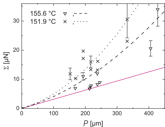
FIG. 7: Dependence of the filament tension upon the perimeter, calculated from the two half axes a, b with a corrugation correction factor of \pi/2 (see text) for all filaments. The solid line indicates the capillary force calculated with \sigma = 0.02 \text{ N/m} , dots/dashes are fits to Eq. (2).
