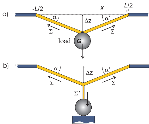
FIG. 2: Geometries for the measurement of filament tensions: a) deflection under the weight of a glass sphere, b) force balance of three filaments
