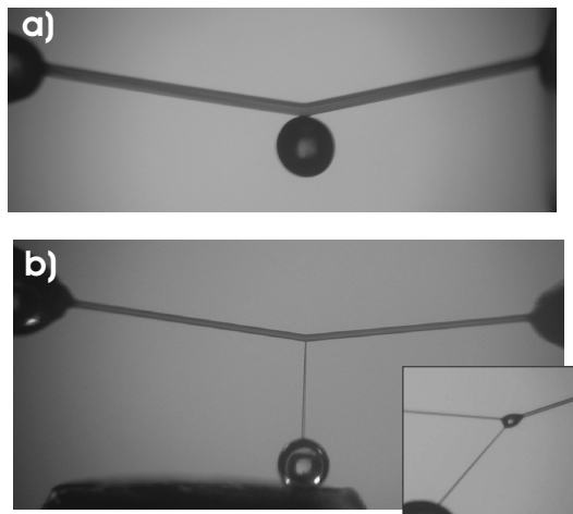
FIG. 3: a) Image of a filament of 152 \mu\text{m} diameter with an attached glass bead. The distance between the two supports is 6 \text{ mm} , the temperature is 2.2 \text{ K} below the melting point. b) Bent filament of 80 \mu\text{m} diameter with a branch to a thin, nearly vertical filament ( 20 \mu\text{m} diameter). The inset shows three connected filaments with different diameters ( 8 \mu\text{m} (top left), 15 \mu\text{m} (right) and 7 \mu\text{m} (bottom left)). The tensions determined from the angles relate as 0.63 : 1.0 : 0.49 , resp.
