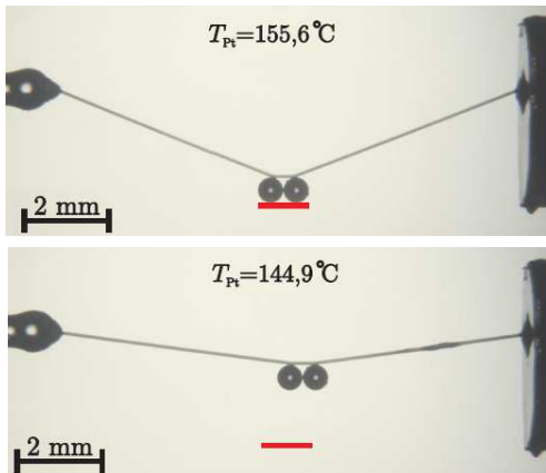
FIG. 5: Filament deflection under load. The horizontal bar marks the initial position at 155.6^\circ\text{C} . All changes are fully reversible. After temperature changes the force equilibrium is established within less than one minute.
