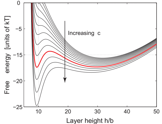
FIG. 3: (Color online) The total mean field thermodynamic potential \Phi vs. polymer layer height h for a = 4 , N = 100 , \chi = -10 , and 10^{-4} < c < 10^{-2} . The development of a minimum of the free energy (global thermodynamic potential) \Phi at low values of h reflects the predicted transition induced by the increase in nanoparticle density. At approximately c = 1.2 \times 10^{-3} (shown via the bold red line), the two minima are equal in energy.
