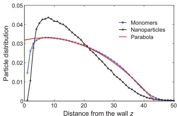
FIG. 4: (Color online) Time averaged histograms of the monomers’ and nanoparticles’ distribution above the grafting surface for parameter values for which few nanoparticles are bound to the brush. The monomer distribution profile is nearly parabolic, as expected for a brush with no nanoparticles. The solid red line shows a parabola to guide the eye. Both profiles were generated for a = 4 , \epsilon_b = 2 , c = 4.2 \times 10^{-5} . The area under both data curves is normalized to unity for presentation purposes.
