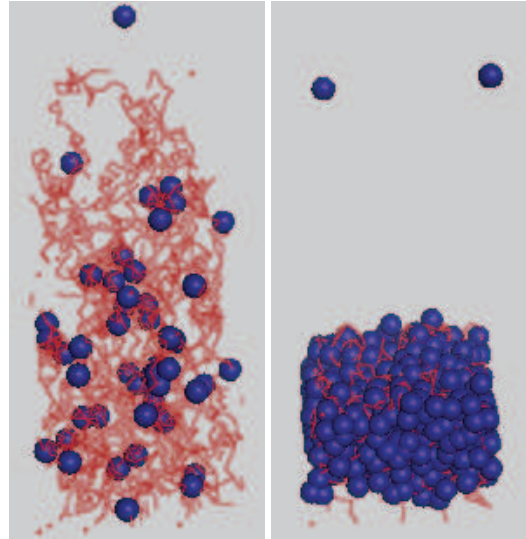
FIG. 1: (Color online) Snapshots of the Langevin simulations illustrating the collapse of the polymer layer upon addition of the nanoparticles. The nanoparticles are shown as blue spheres. Polymer chains, grafted from below onto a flat surface (not shown), are depicted in line format (i.e., their bead-spring structure is not resolved here). Left panel: The layer in the extended swollen state just below the transition; c = 6.9 \times 10^{-5} . Right panel: The collapsed layer packed with nanoparticles, just above the transition; c = 2.4 \times 10^{-4} . \epsilon_b = 2 and a = 4 for both panels. Snapshots were visualized using PyMOL [50].
