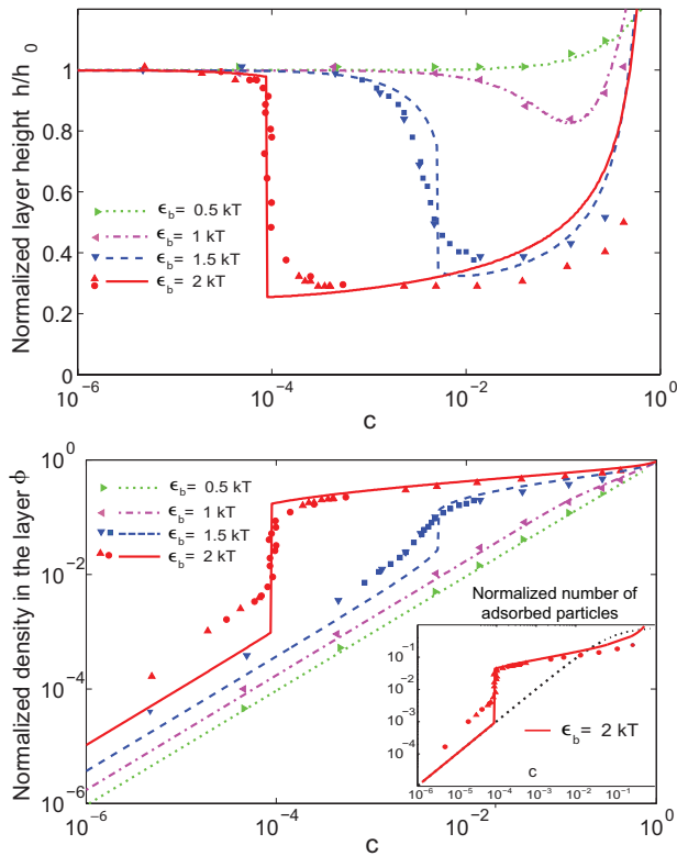
FIG. 2: (Color online) Upper panel: Layer height, h , normalized by the height in the absence of nanoparticles, h_0 , as a function of the concentration of the free nanoparticles in solution, c , for different interaction strengths. Lower panel: Average nanoparticle density in the layer as a function of c for the same interaction strengths as in the upper panel. The inset shows the number of adsorbed particles, per unit area, compared to a simple Langmuir adsorption isotherm (dotted line). In both panels the lines are the mean field theory ( \chi = -0.75, -4, -8, -13.5 ), filled triangles correspond to grand-canonical simulations, filled circles or squares - canonical simulations. In both panels the grafting distance is a = 4b .
